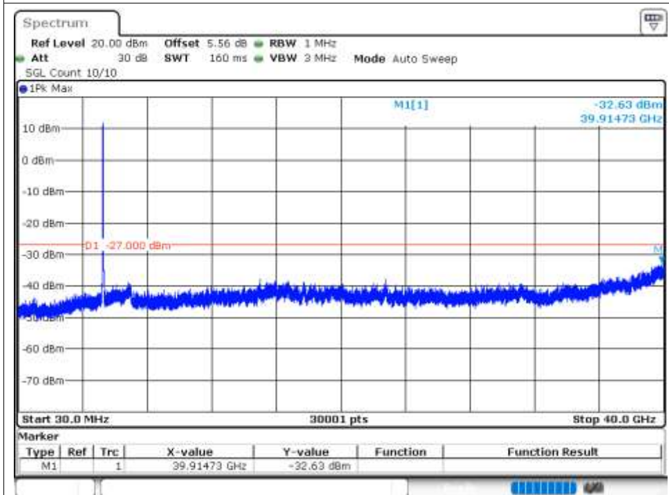
Tx. Spurious NVNT n40 5270MHz Ant1 Emission
