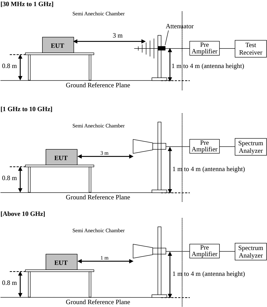
Figure 2: Test Setup
