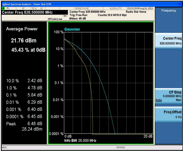
Band5-5MHz-QPSK-20425-1RB#0-PASS
