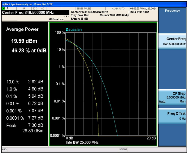
Band5-5MHz-16QAM-20625-25RB#0-PASS
