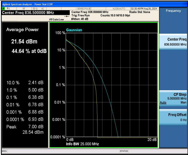
Band5-1.4MHz-QPSK-20525-1RB#0-PASS
