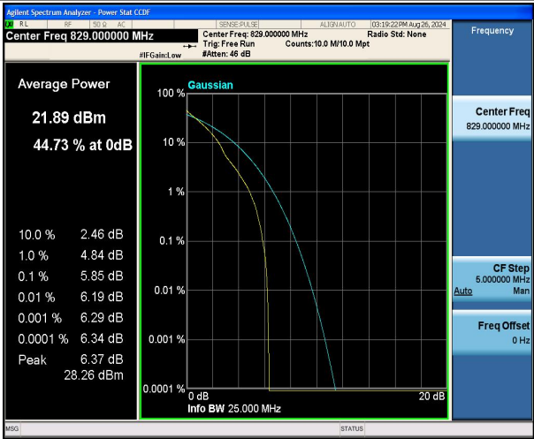
Band5-10MHz-QPSK-20450-1RB#0-PASS
