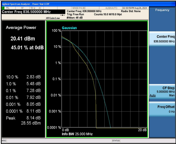
Band5-1.4MHz-16QAM-20525-1RB#0-PASS
