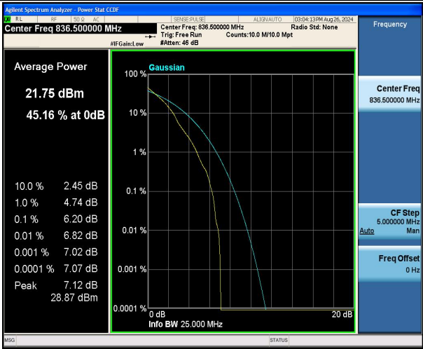
Band5-5MHz-QPSK-20525-1RB#0-PASS
