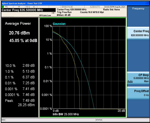
Band5-5MHz-16QAM-20425-1RB#0-PASS
