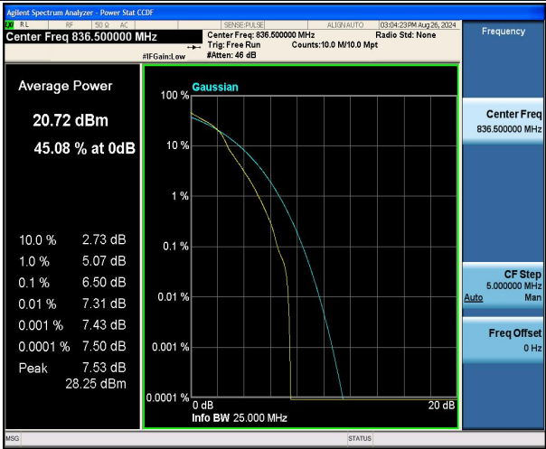
Band5-5MHz-16QAM-20525-1RB#0-PASS
