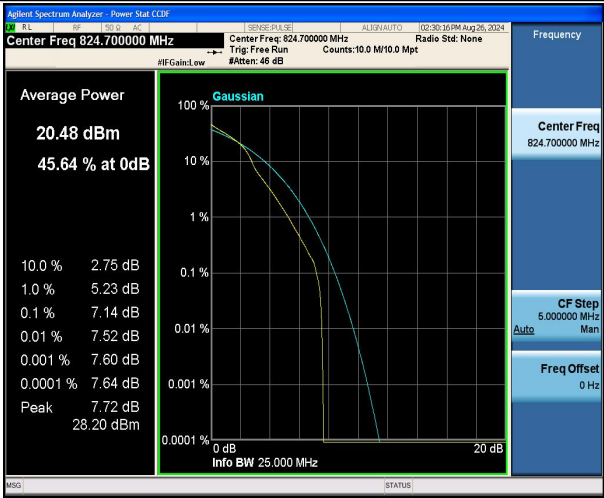
Band5-1.4MHz-16QAM-20407-1RB#0-PASS
