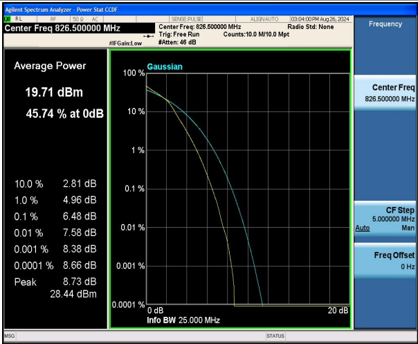
Band5-5MHz-16QAM-20425-25RB#0-PASS
