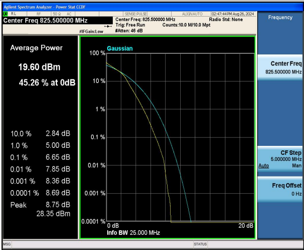
Band5-3MHz-16QAM-20415-15RB#0-PASS
