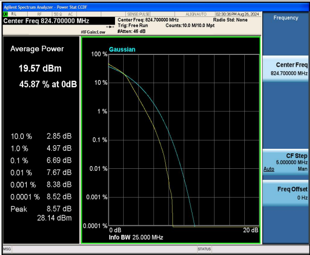
Band5-1.4MHz-16QAM-20407-6RB#0-PASS
