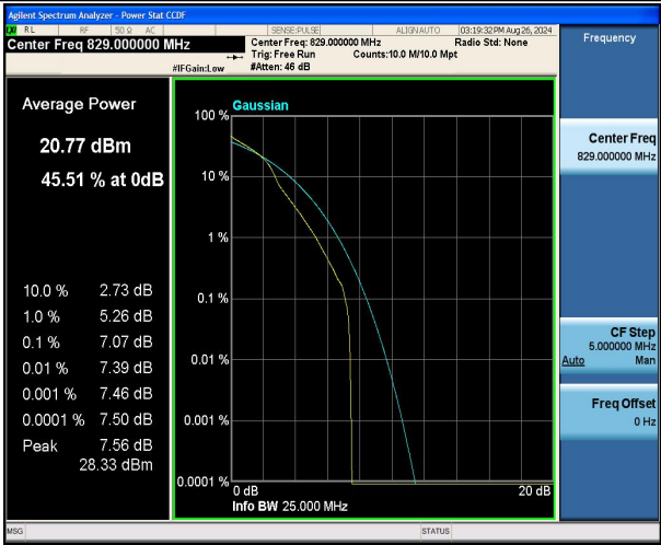
Band5-10MHz-16QAM-20450-1RB#0-PASS
