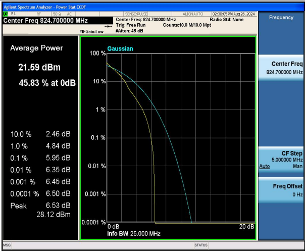
Band5-1.4MHz-QPSK-20407-1RB#0-PASS
