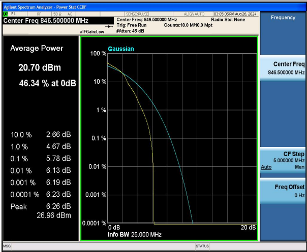
Band5-5MHz-16QAM-20625-1RB#0-PASS
