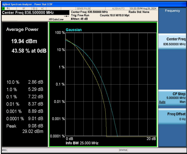
Band5-10MHz-16QAM-20525-50RB#0-PASS
