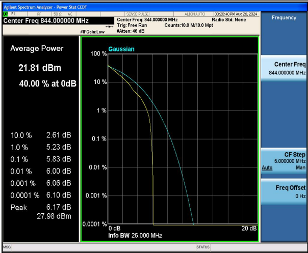
Band5-10MHz-QPSK-20600-1RB#0-PASS
