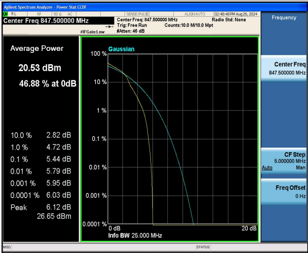
Band5-3MHz-16QAM-20635-1RB#0-PASS
