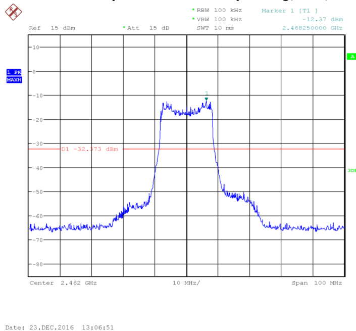
Fig.47 Conducted Spurious Emission (802.11g, Ch11)
