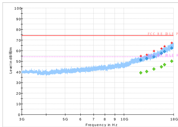
Fig.77 Radiated Spurious Emission (802.11 n-20MHz,Ch11,3GHz~18GHz)
