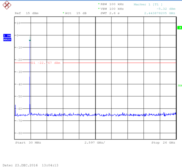
Fig.42 Conducted Spurious Emission (802.11b, Ch11, 30MHz~26GHz)
