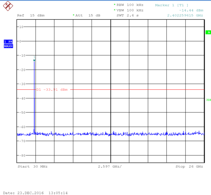
Fig.44 Conducted Spurious Emission (802.11g, Ch1, 30MHz~26GHz)
