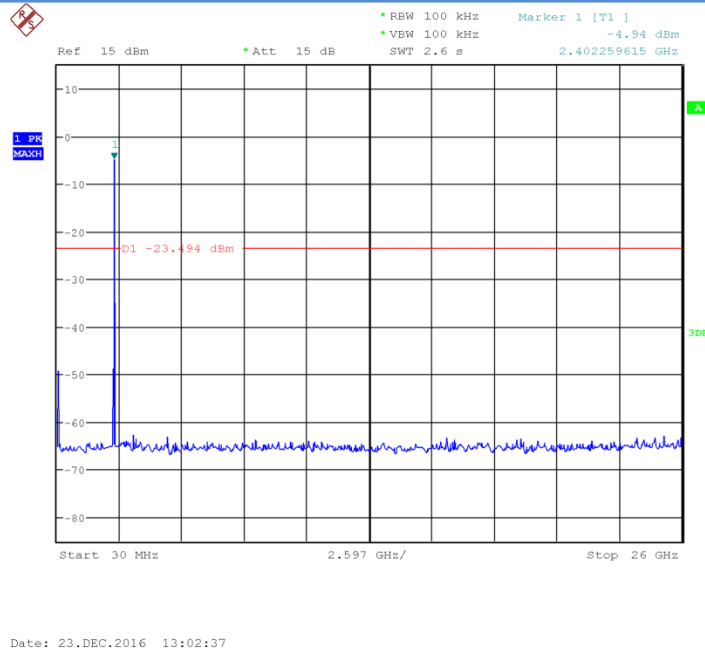
Fig.38 Conducted Spurious Emission (802.11b, Ch1, 30MHz~26GHz)
