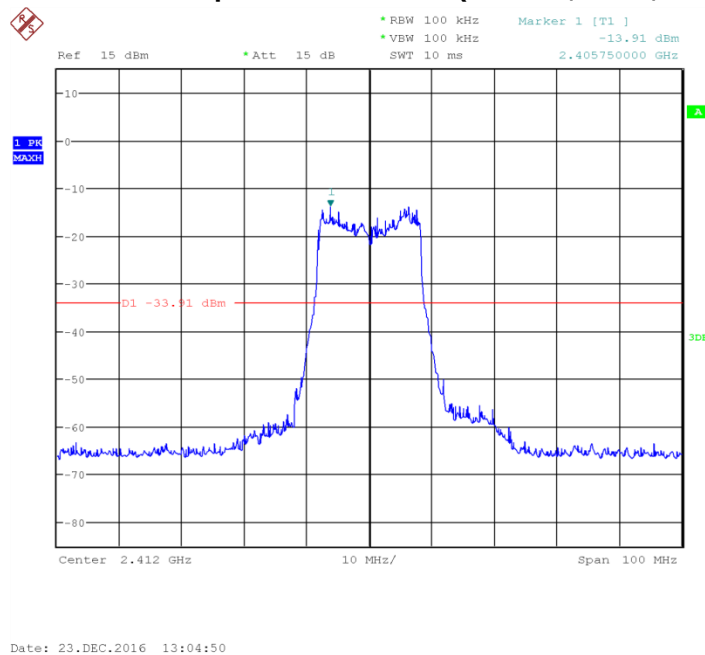
Fig.43 Conducted Spurious Emission (802.11g, Ch1)
