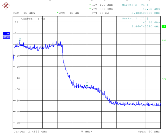
Fig.30 Band Edges (802.11g, Ch11)
