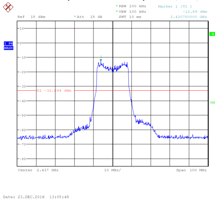
Fig.39 Conducted Spurious Emission (802.11b, Ch6)
