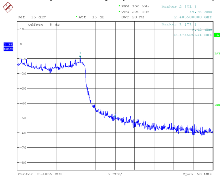
Fig.34 Band Edges (802.11b-20MHz, Ch11)
