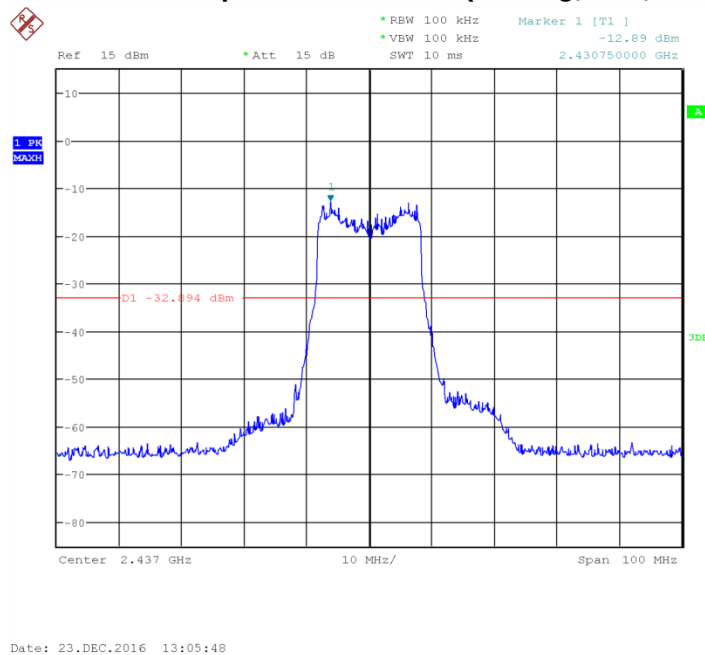
Fig.45 Conducted Spurious Emission (802.11g, Ch6)
