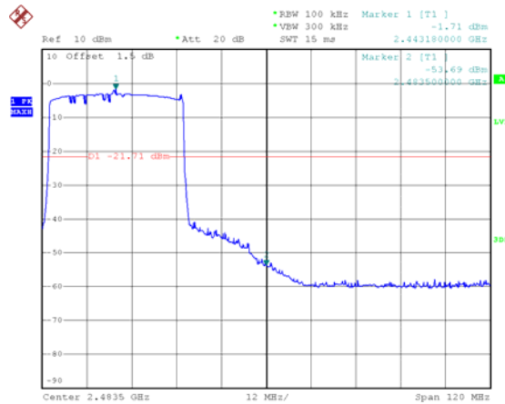
2443.5 MHz
