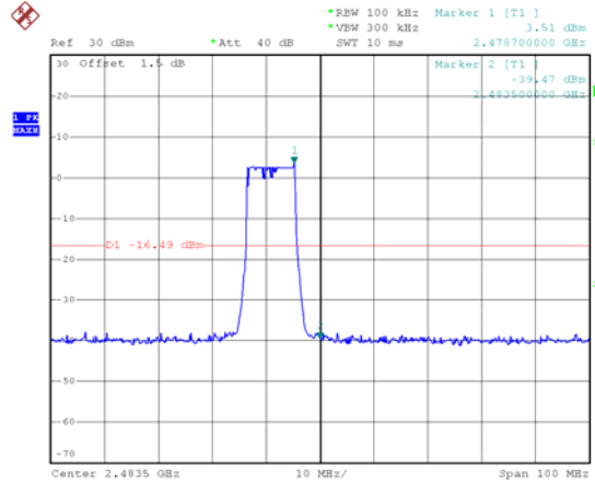
2474.5 MHz
