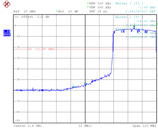
2441.5 MHz
