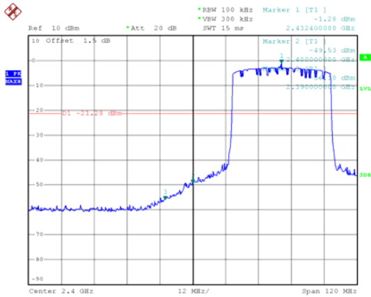
2432.5 MHz
