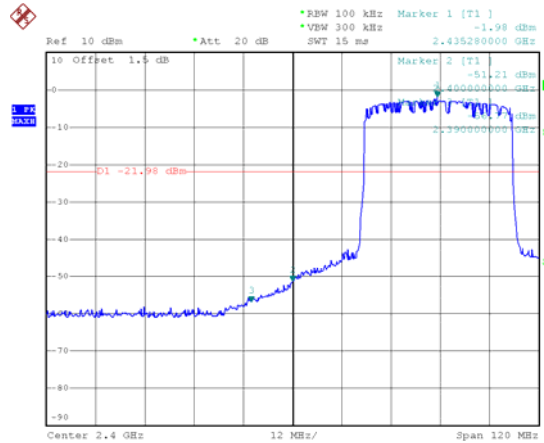
2435.5 MHz
