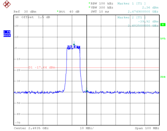
2474.5 MHz
