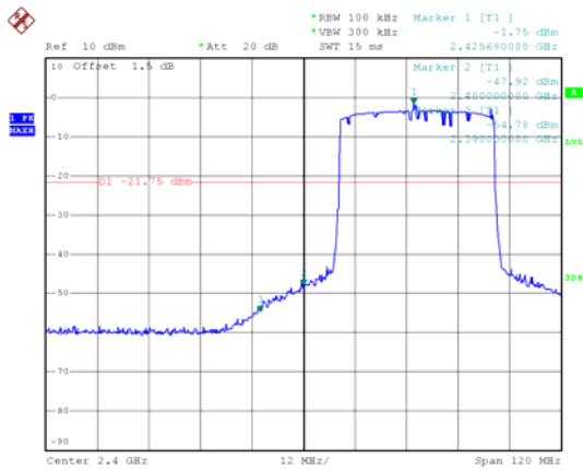
2426.5 MHz
