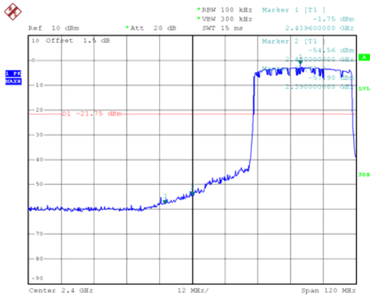
2440.5 MHz
