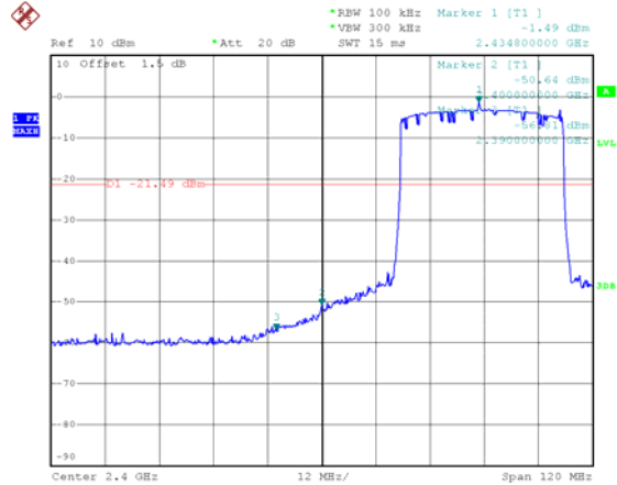
2435.5 MHz
