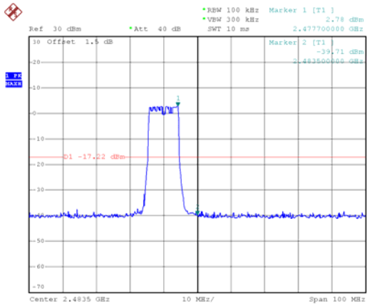
2473.5 MHz
