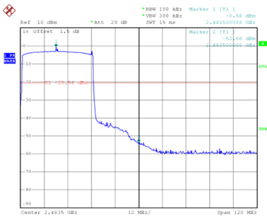
2442.5 MHz
