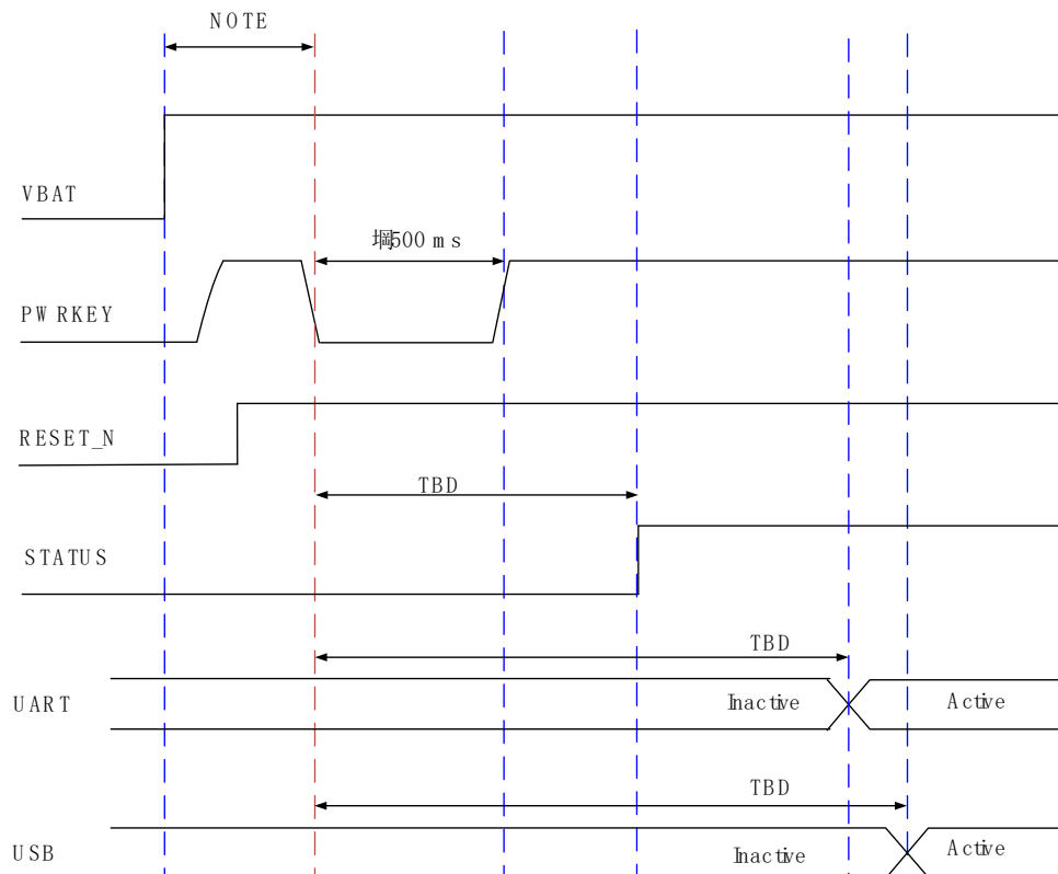
Figure 13: Turn-on Timing
