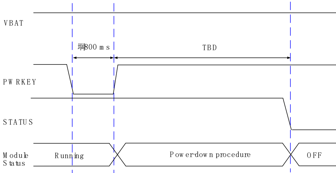
Figure 14: Turn-off Timing
