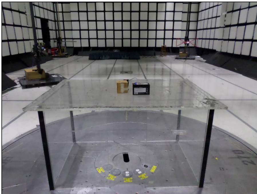
Photograph 4. Spurious Emissions, Outside the Band 13.110 - 14.010 MHz, 30 – 135.6 MHz, Rear View
