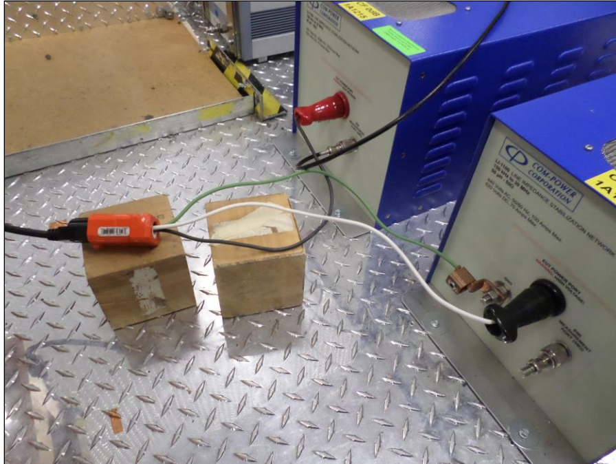
Photograph 1. Conducted Emissions, LISN Connections
