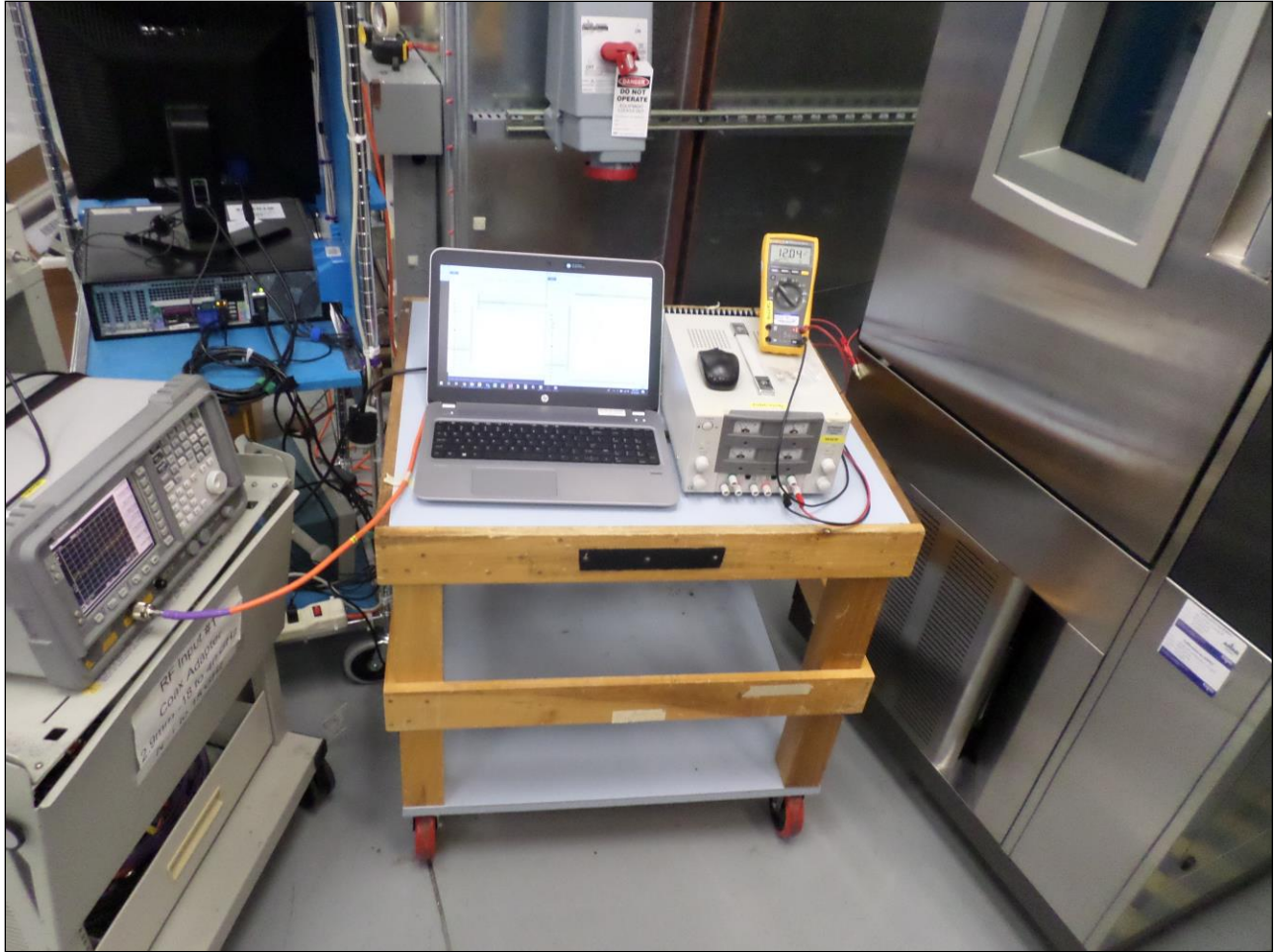
Photograph 8. Frequency Stability, Test Setup
