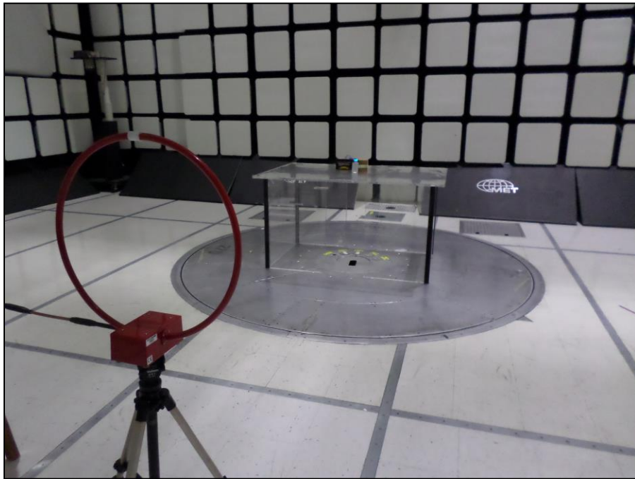
Photograph 6. Spurious Emissions, Outside the Band 13.110 - 14.010 MHz, 9 kHz – 30 MHz, Antenna View
