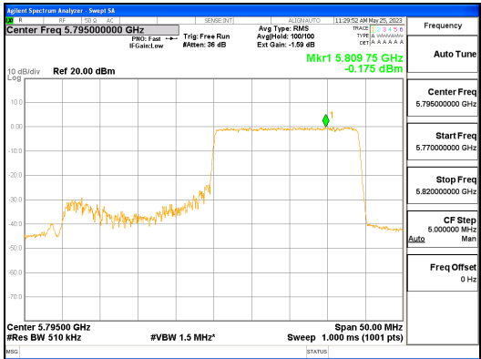
ANT_R_802.11ax_HE40_242T_High_UNII 3
