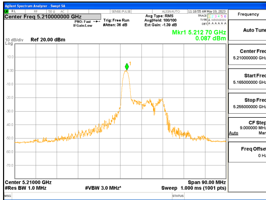
ANT L_802.11ax_HE80_26T_Mid_UNII 1
