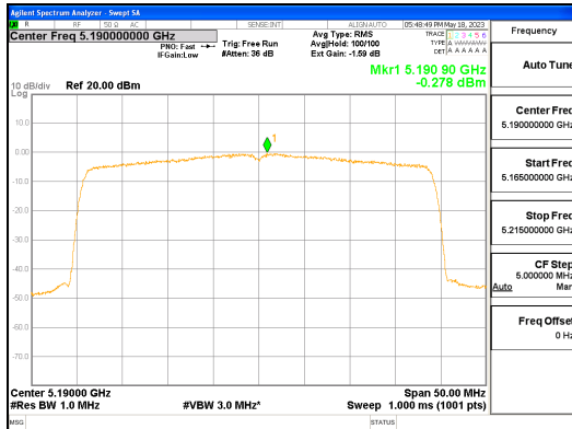
ANT R_802.11ax_HE40_484T_UNII 1
