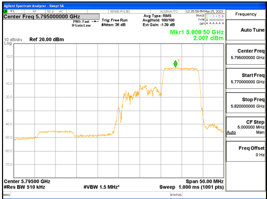
ANT L_802.11ax_HE40_106T_High_UNII 3
