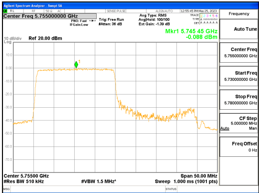
ANT L_802.11ax_HE40_242T_Low_UNII 3
