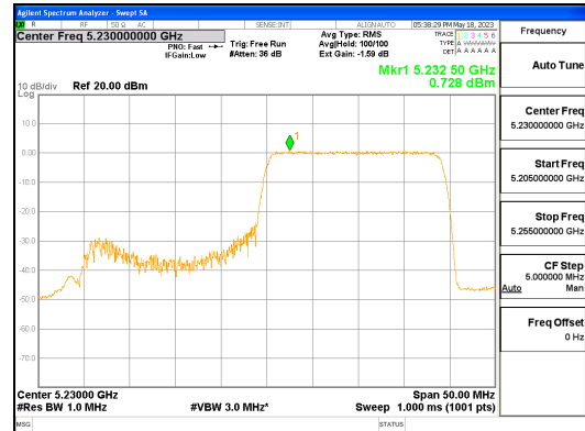
ANT R_802.11ax_HE40_242T_High_UNII 1
