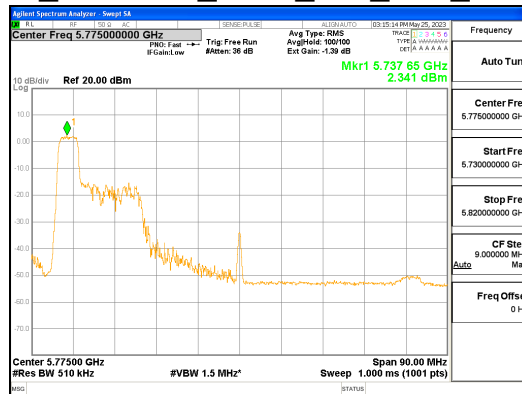
ANT L_802.11ax_HE80_52T_Low_UNII 3
