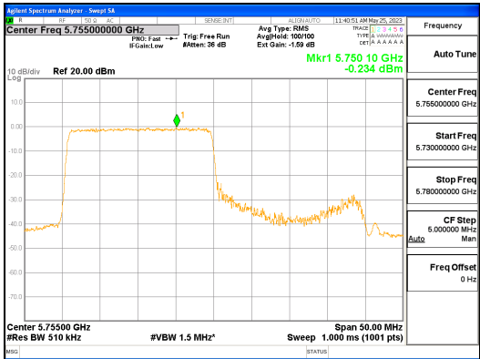
ANT R_802.11ax_HE40_242T_Low_UNII 3
