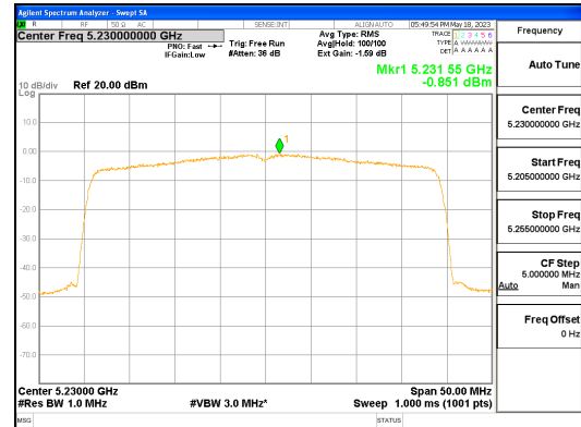
ANT R_802.11ax_HE40_484T_UNII 1
