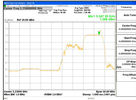
ANT L_802.11ax_HE40_106T_High_UNII 1
