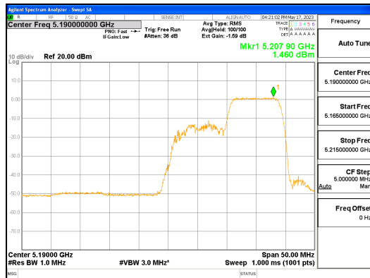
ANT R_802.11ax_HE40_106T_High_UNII 1
