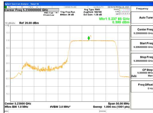
ANT L_802.11ax_HE40_242T_High_UNII 1
