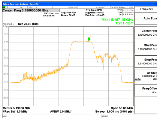
ANT R_802.11ax_HE40_106T_Mid_UNII 1
