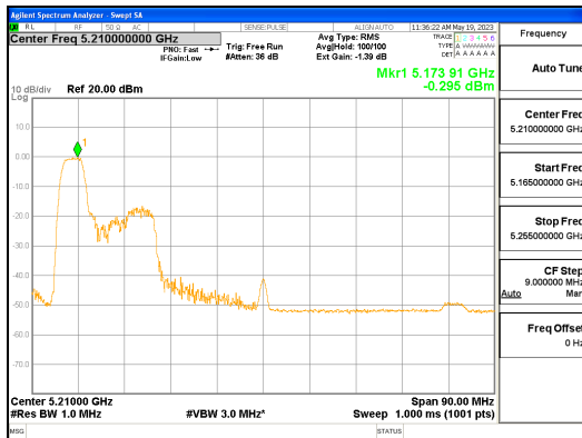
ANT L_802.11ax_HE80_52T_Low_UNII 1
