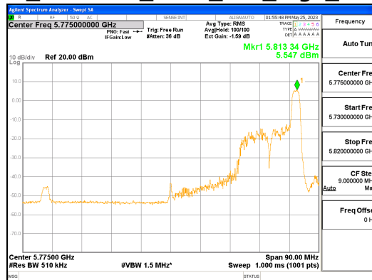
ANT R_802.11ax_HE80_26T_High_UNII 3
