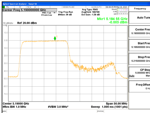
ANT L_802.11ax_HE40_242T_Low_UNII 1
