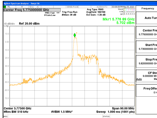
ANT L_802.11ax_HE80_26T_Mid_UNII 3
