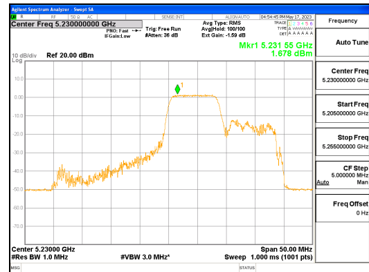
ANT R_802.11ax_HE40_106T_Mid_UNII 1
