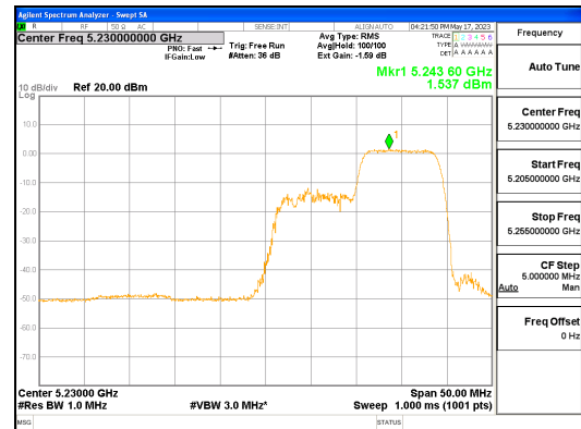
ANT R_802.11ax_HE40_106T_High_UNII 1
