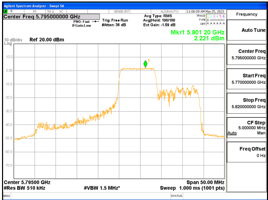
ANT R_802.11ax_HE40_106T_Mid_UNII 3
