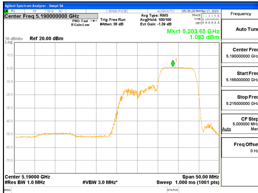
ANT L_802.11ax_HE40_106T_High_UNII 1
