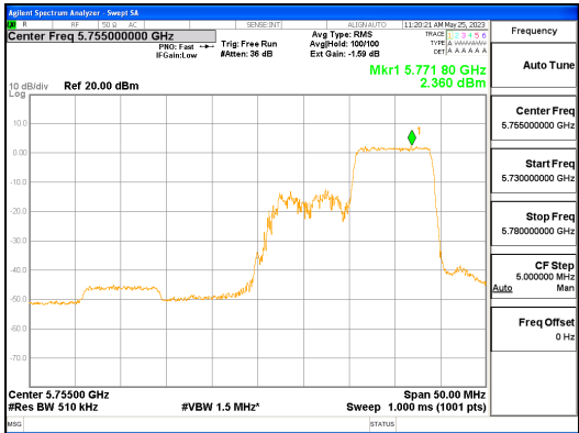
ANT_R_802.11ax_HE40_106T_High_UNII 3
