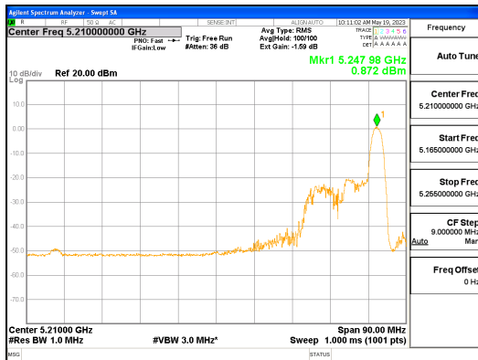
ANT R_802.11ax_HE80_26T_High_UNII 1
