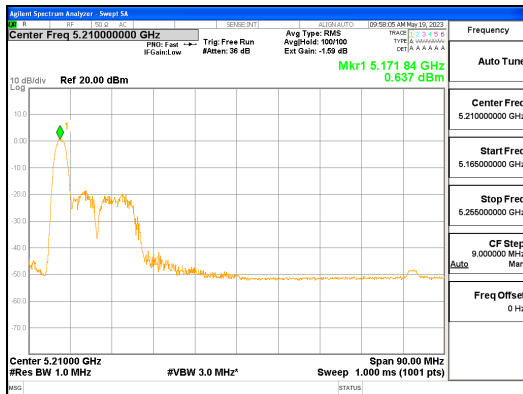
ANT R_802.11ax_HE80_26T_Low_UNII 1
