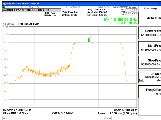
ANT R_802.11ax_HE40_242T_High_UNII 1
