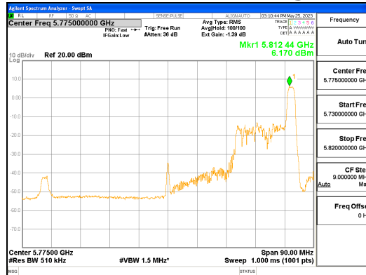
ANT L_802.11ax_HE80_26T_High_UNII 3
