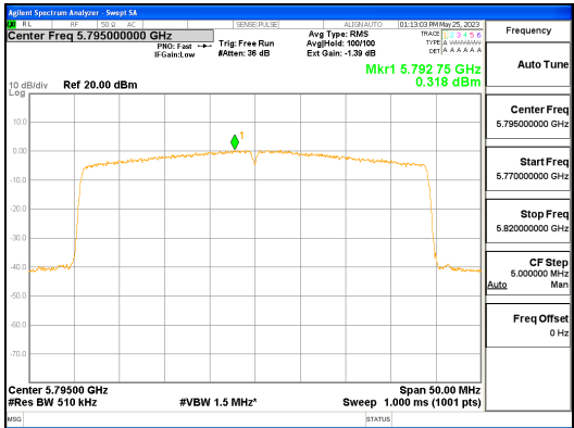
ANT L_802.11ax_HE40_484T_UNII 3
