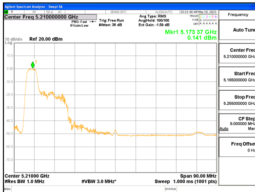
ANT R_802.11ax_HE80_52T_Low_UNII 1
