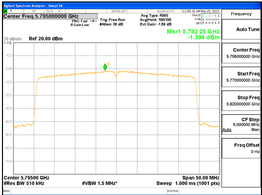
ANT R_802.11ax_HE40_484T_UNII 3
