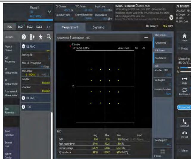
41-41-20MHz-20MHz-16QAM-16QAM-40521-40719-100RB#0-100RB#0
