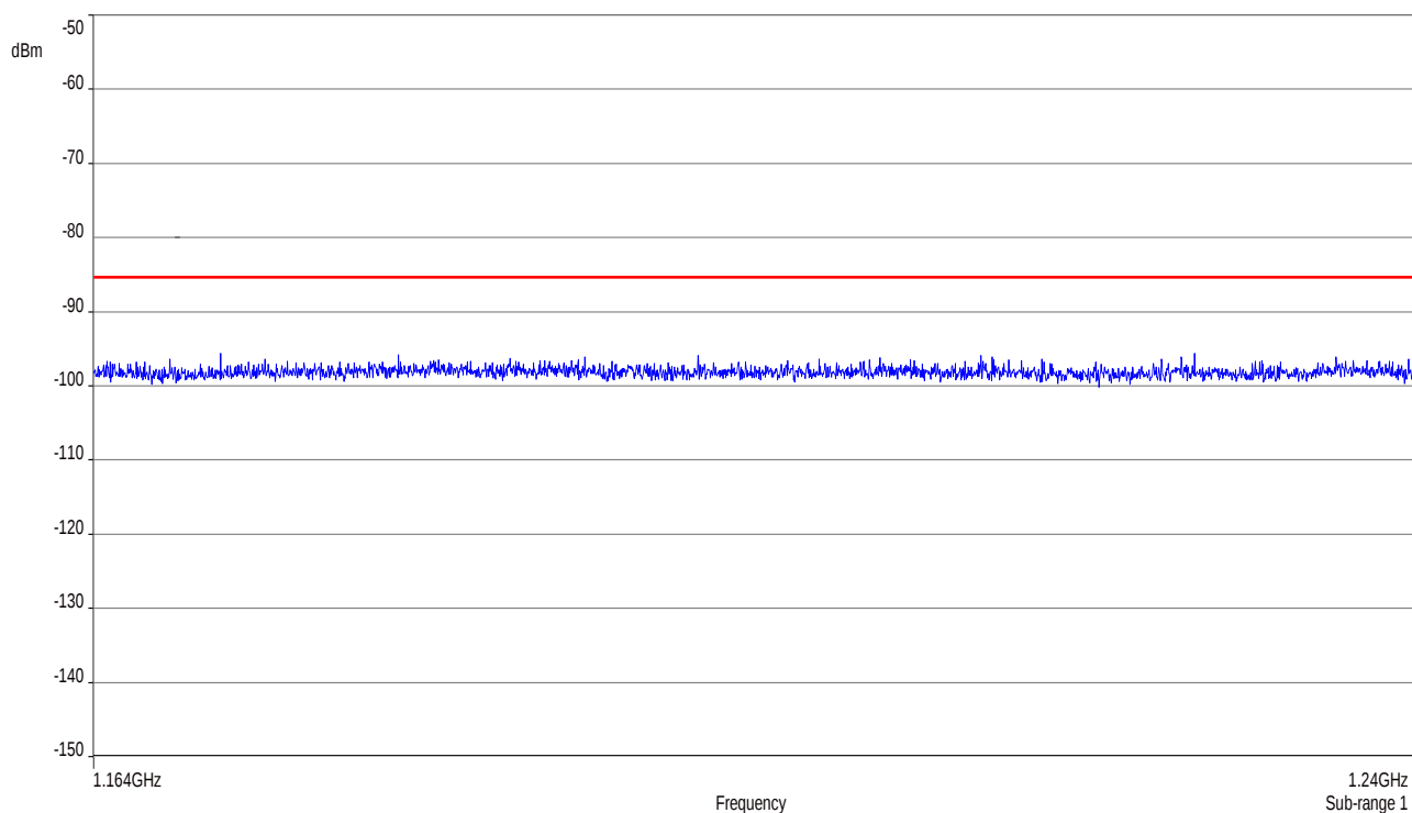
Plot 15: Channel 7, 1.164 GHz – 1.240 GHz
