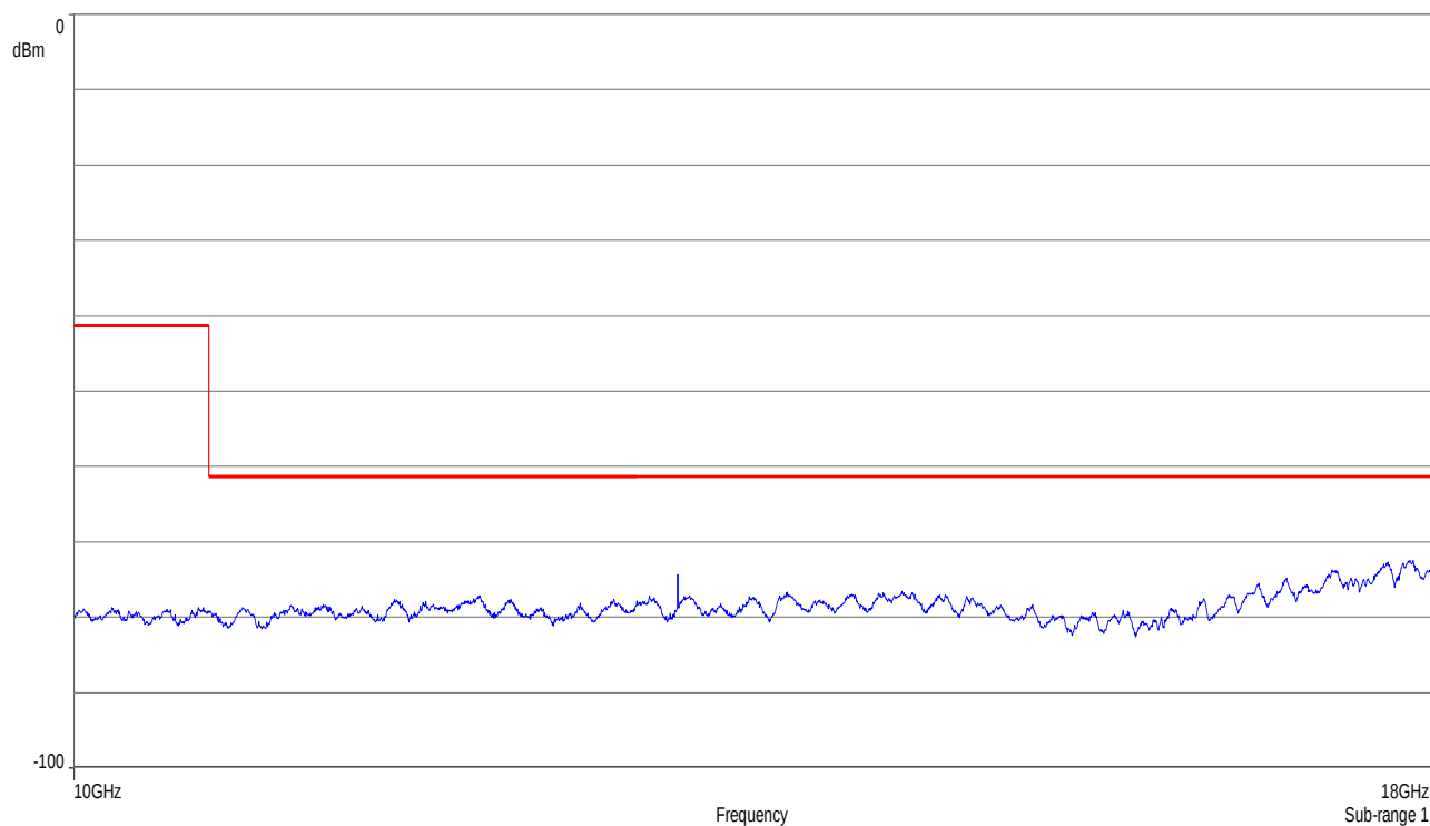
Plot 14: Channel 7, 10 GHz – 18 GHz
