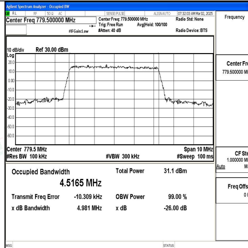
Band13-5MHz-16QAM-23205-25RB#0-PASS
