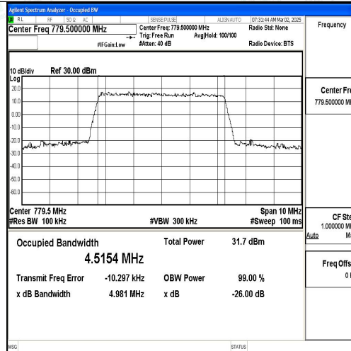
Band13-5MHz-QPSK-23205-25RB#0-PASS
