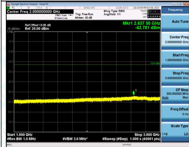
Band2_20MHz_QPSK_18900_100RB#0_1000~3000_100
