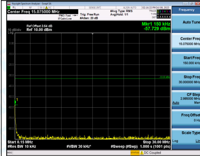
Band2_20MHz_16QAM_19100_1RB#99_0.15~30_0.15~3 0
