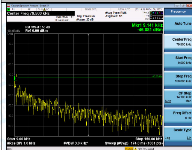
Band2_20MHz_QPSK_19100_100RB#0_0.009~0.15_0.00
