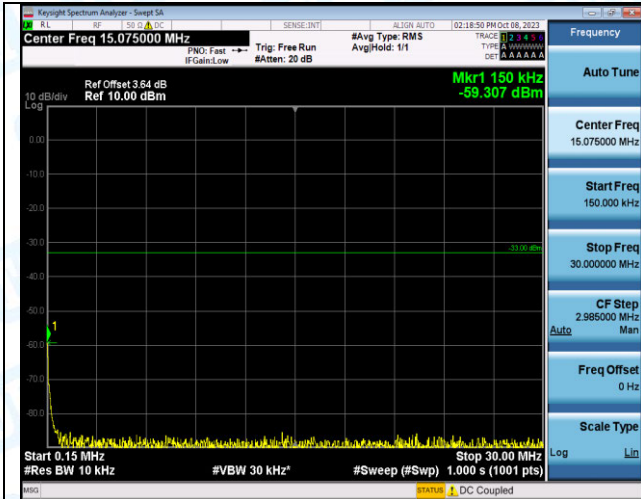
Band2_20MHz_QPSK_18900_100RB#0_0.15~30_0.15~3
