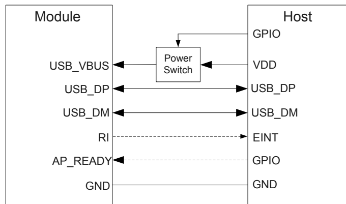
Figure 6: Sleep Application without Suspend Function
