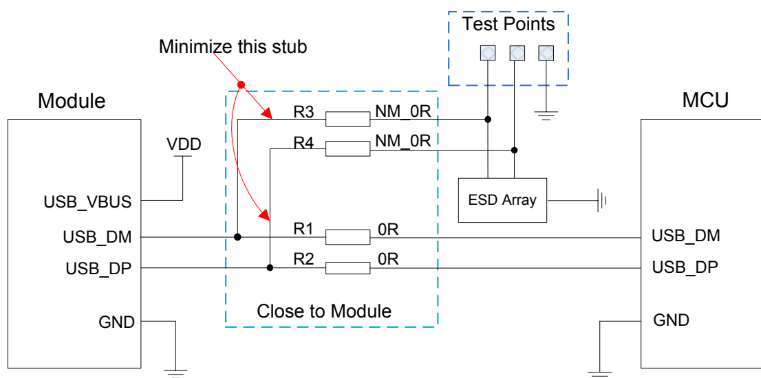
Figure 19: Reference Circuit of USB Application
