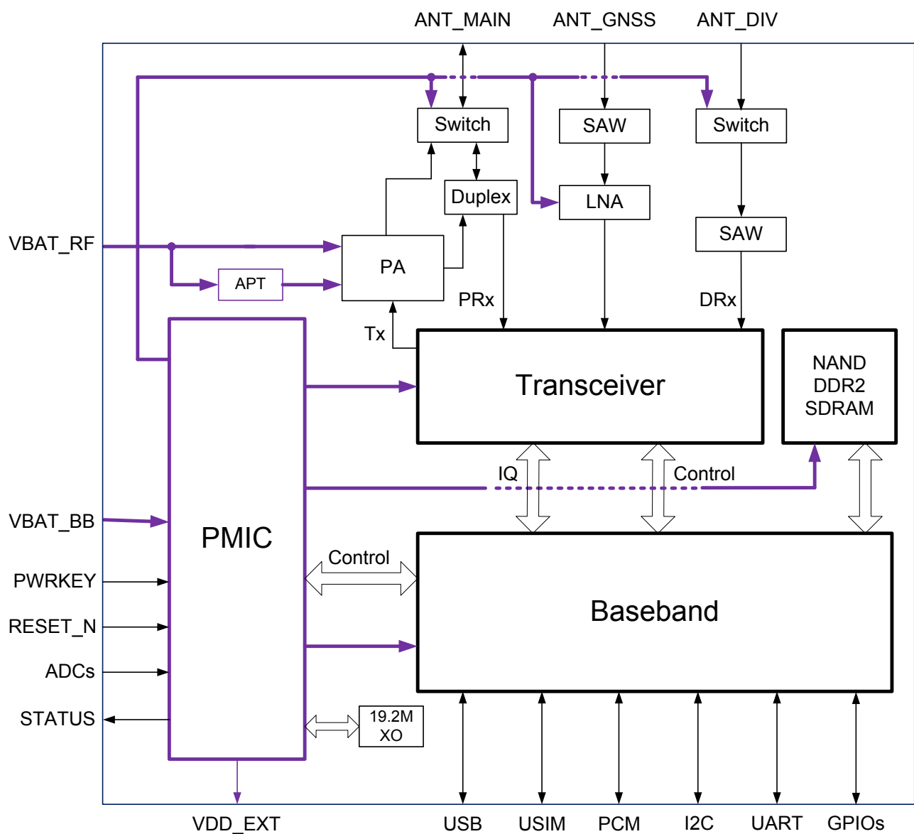
Figure 1: Functional Diagram
