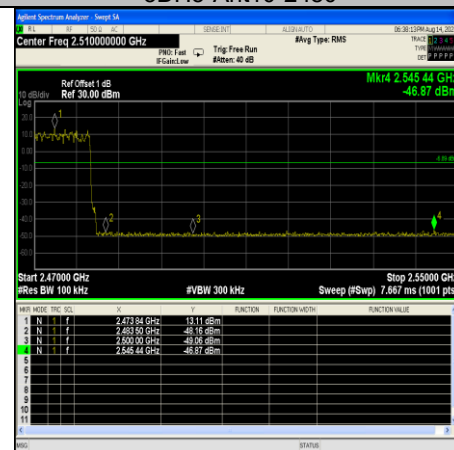
3DH5-Ant10-Hop_2480
