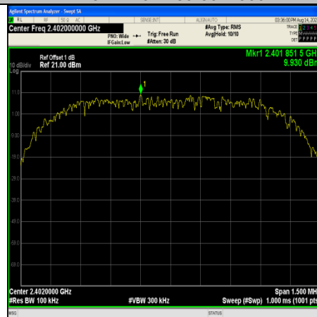
2DH5-Ant10-2402-0~Reference
