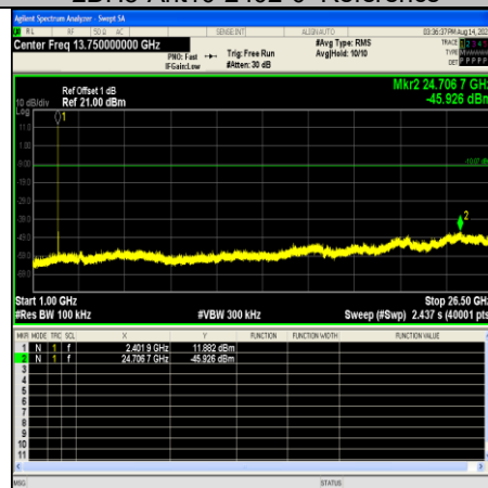
2DH5-Ant10-2402-1000~26500
