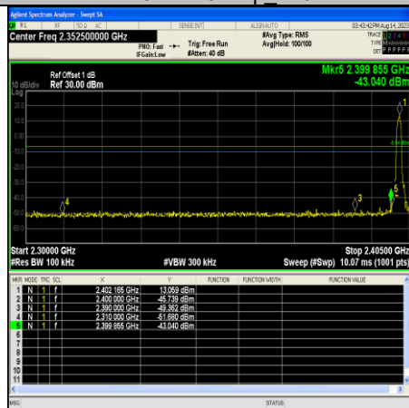
3DH5-Ant10-2402
