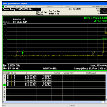
2DH5-Ant10-Hop_2402
