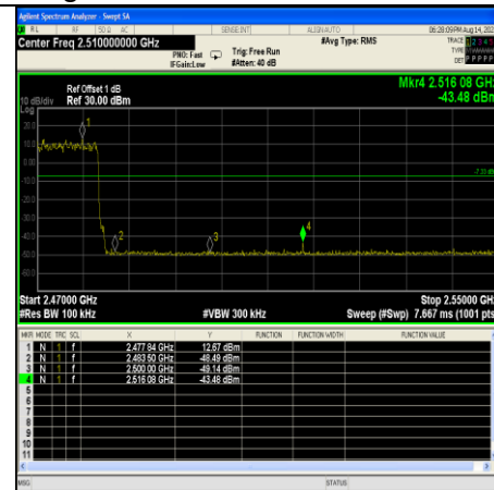
2DH5-Ant10-Hop_2480
