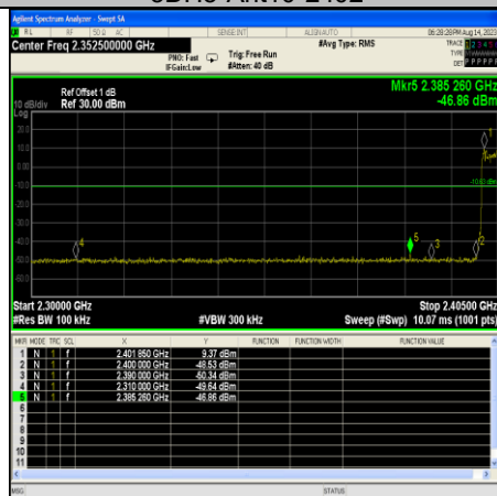
3DH5-Ant10-Hop_2402
