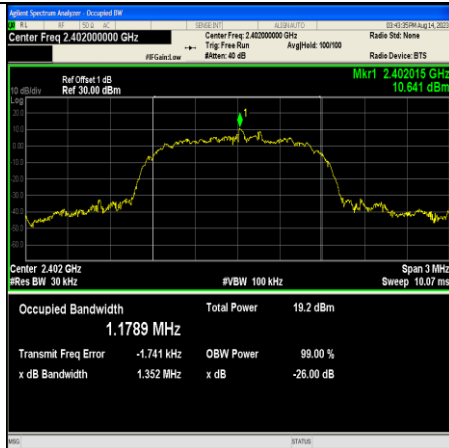
3DH5-Ant10-2402
