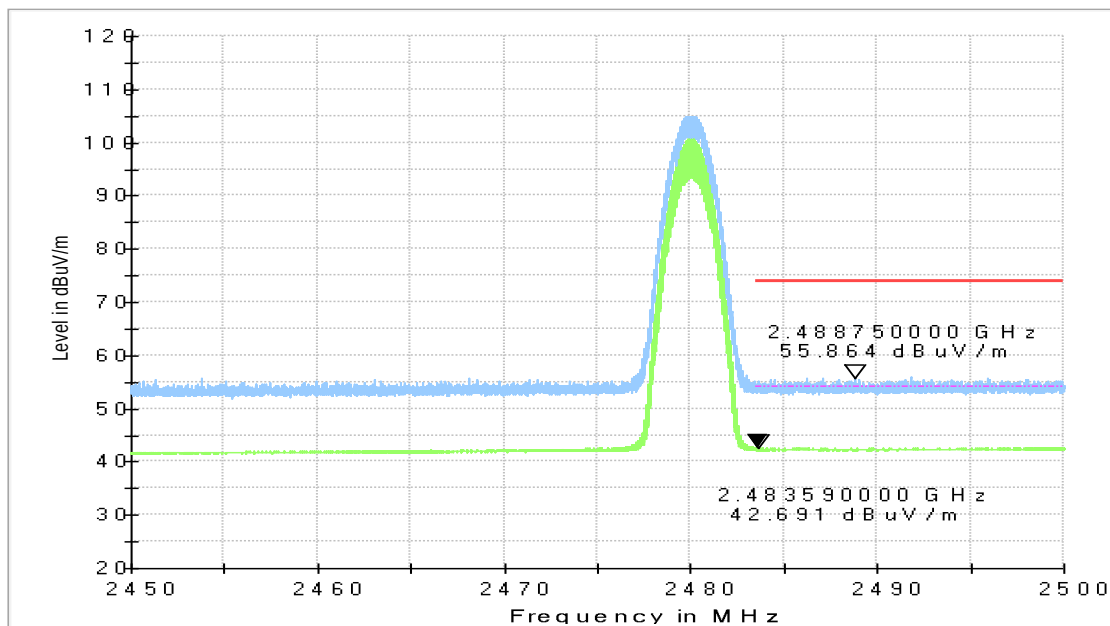
Fig.18. Frequency Band Edges: 8DPSK, Channel 78, 2.45 GHz - 2.50GHz
