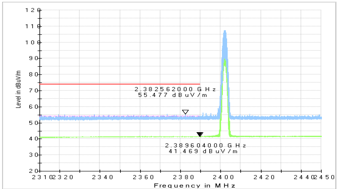
Fig.13. Frequency Band Edges: GFSK, Channel 0, 2.31 GHz – 2.45GHz
