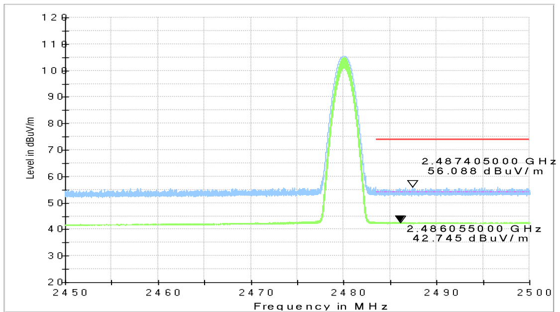
Fig.14. Frequency Band Edges: GFSK, Channel 78, 2.45 GHz - 2.50GHz
