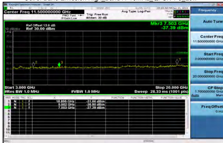
Out of Band Emission High_Band41 10MHz_QPSK 1_0_Low
