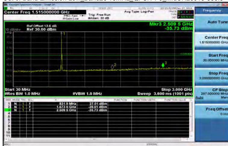
Out of Band Emission Low_Band26 10MHz_QPSK 1 0_MidCH26915-836.5
