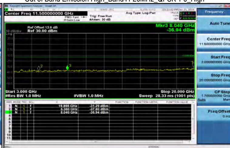
Out of Band Emission High_Band41 20MHz_QPSK 1_0_High
