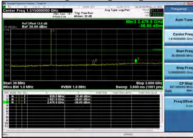
Out of Band Emission Low_Band26 3MHz_QPSK 1 0_LowCH26805-825.5
