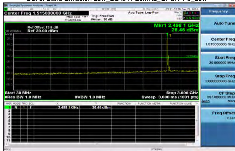
Out of Band Emission Low_Band41 20MHz_QPSK 1_0_Low
