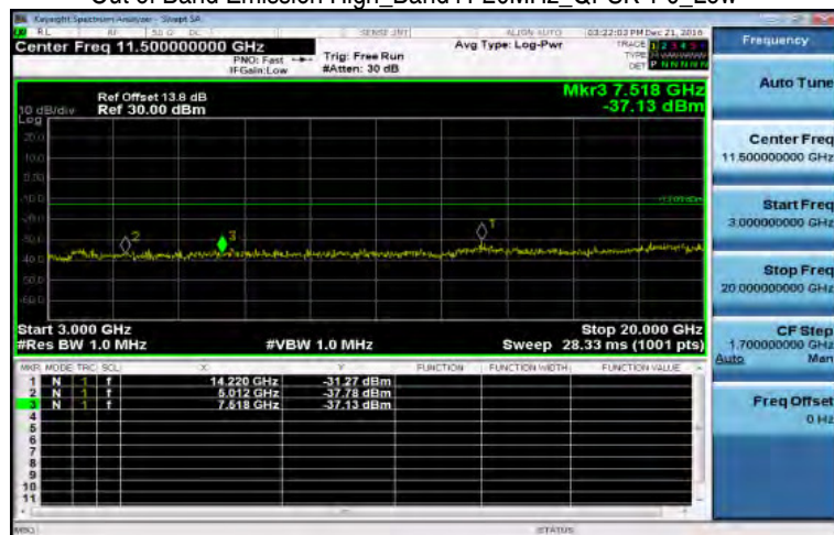
Out of Band Emission High_Band41 20MHz_QPSK 1_0_Low
