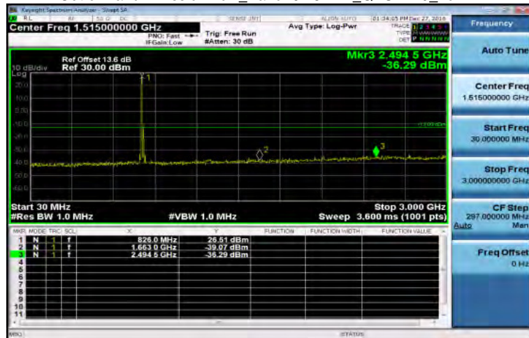
Out of Band Emission Low_Band26 15MHz_QPSK 1_0_Low
