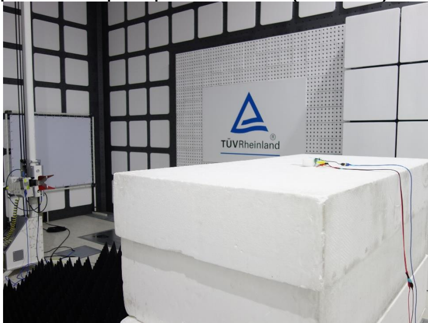
Photograph 5: Test Setup for Spurious Emissions (Back View 3)
