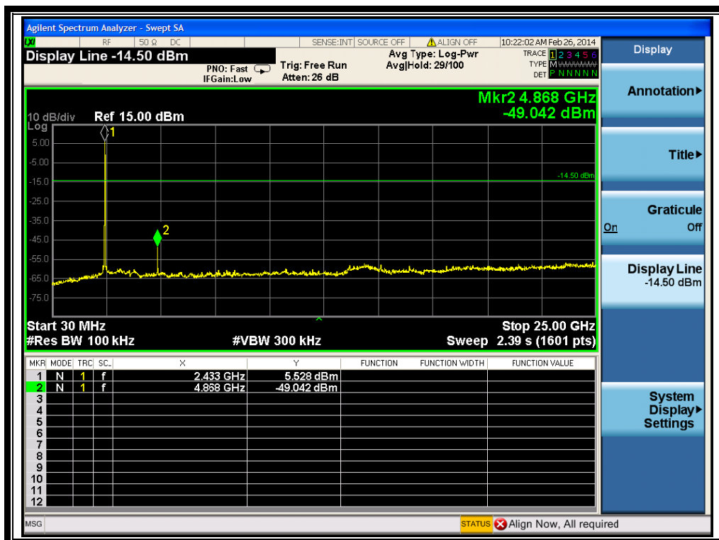
(Plot B.1: Channel = 6, 30MHz to 25GHz)
