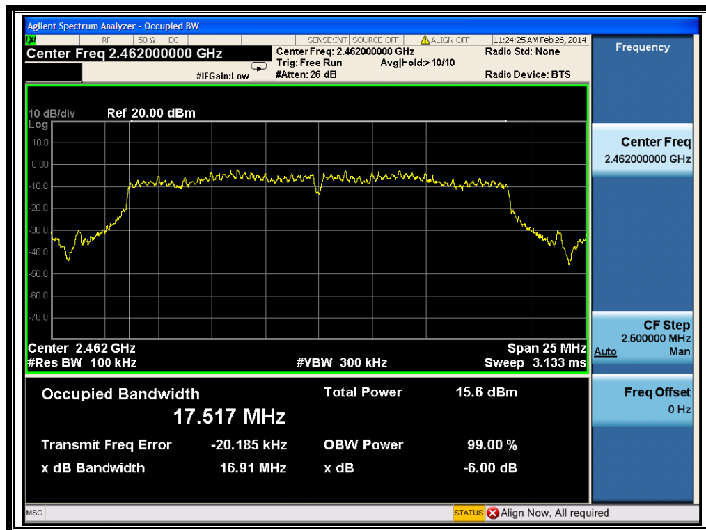
(Plot I: Channel 11: 2462MHz @ 802.11n-20)
