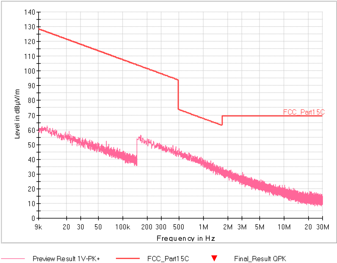
Fig. 16: All Mode. Frequency range: 9 kHz – 30 MHz – Axis Z FINAL MEASUREMENTS
