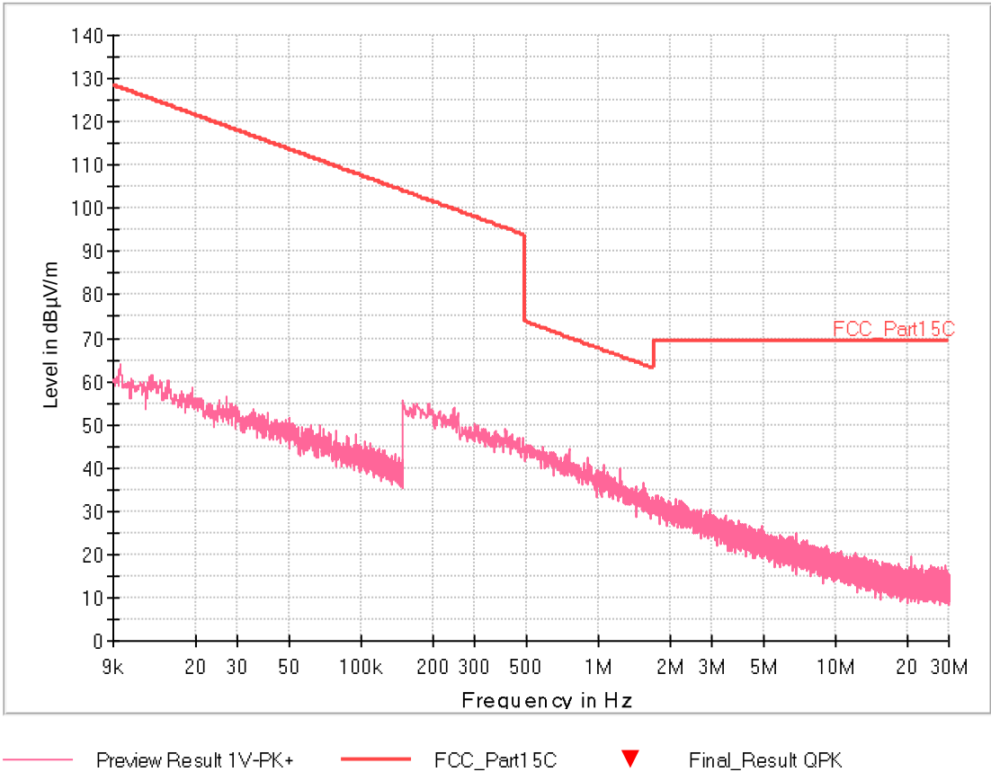
Fig. 15: All Mode. Frequency range: 9 kHz – 30 MHz – Axis Y FINAL MEASUREMENTS
