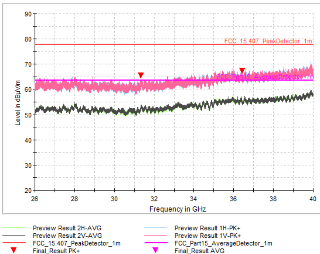
Fig. 26: All mode. Frequency range: 26 GHz – 40 GHz
