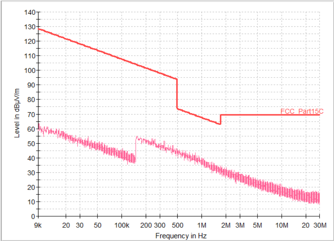
Fig. 6: Ambient level. All Mode. Frequency range: 9 kHz – 30 MHz - Axis Y
