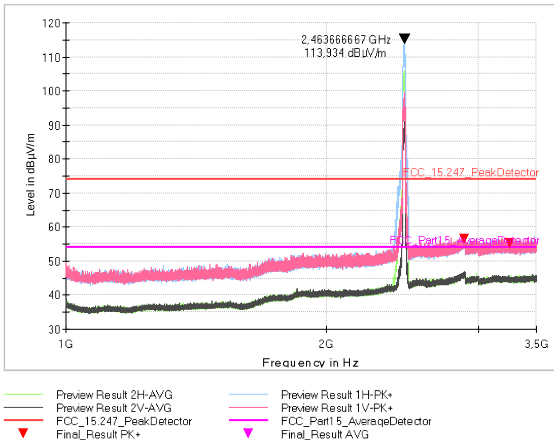
Fig. 18: Mode 1. Frequency range: 1 GHz – 3.5 GHz
