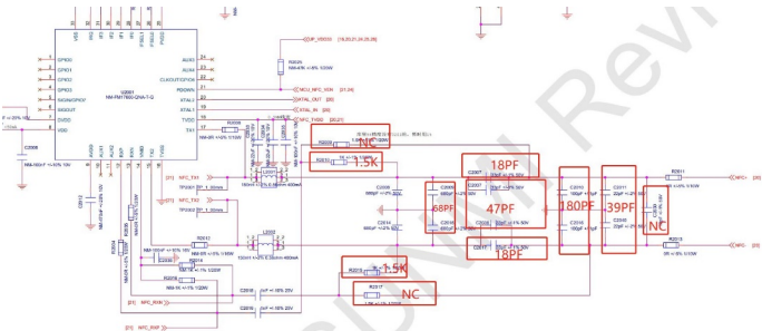
Matching Circuit, Switch Logic Schematic(CAD and Tag Number Diagram)
