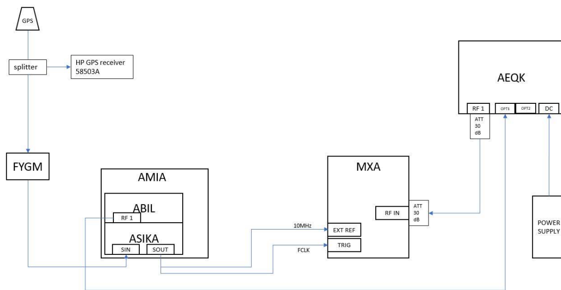
Test Setup for Frequency Stability
