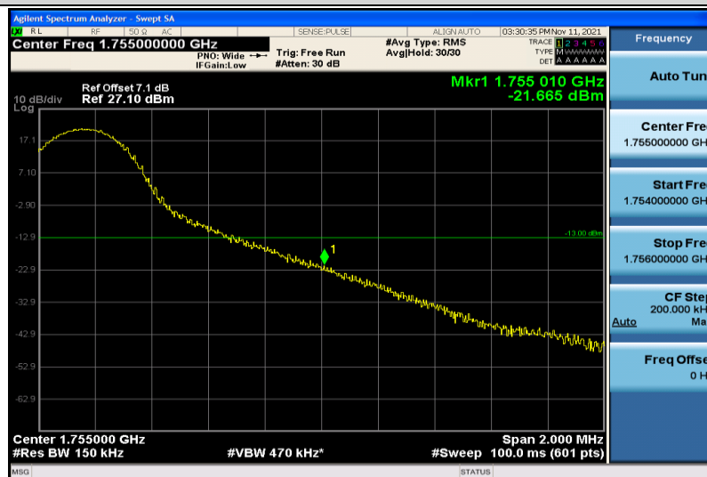
Band4-15MHz-QPSK-20325-1RB#74
