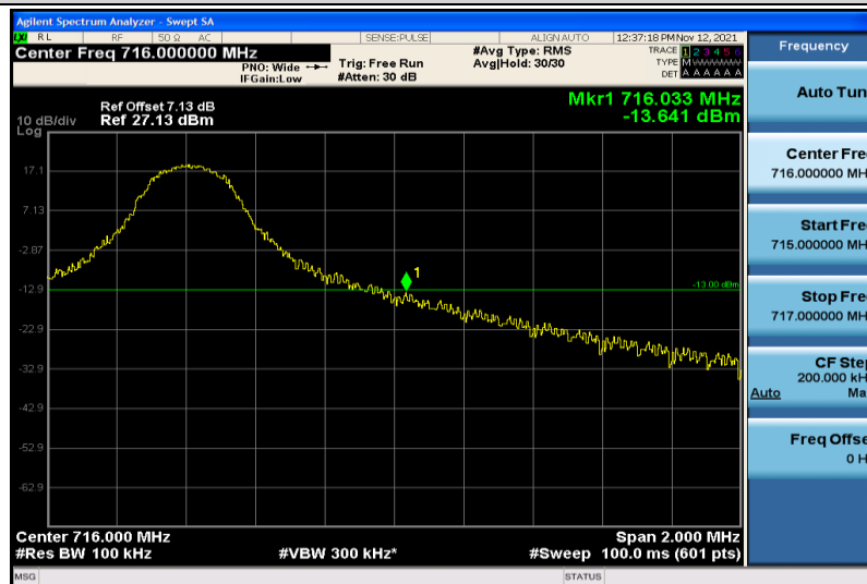
Band17-10MHz-QPSK-23800-1RB#49
