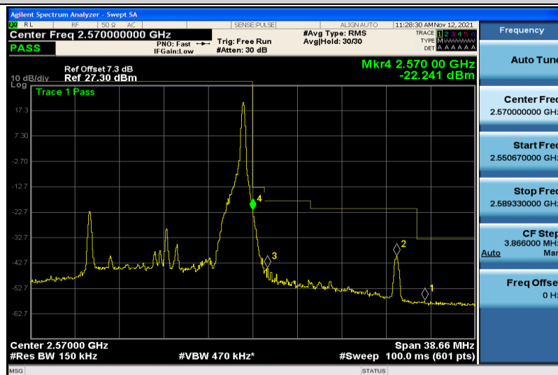
Band7-15MHz-16QAM-21375-1RB#74
