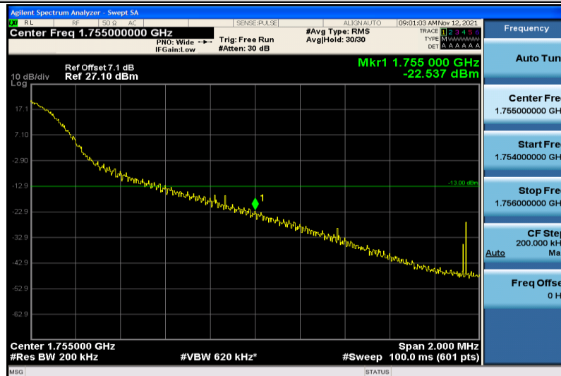
Band4-20MHz-16QAM-20300-1RB#99
