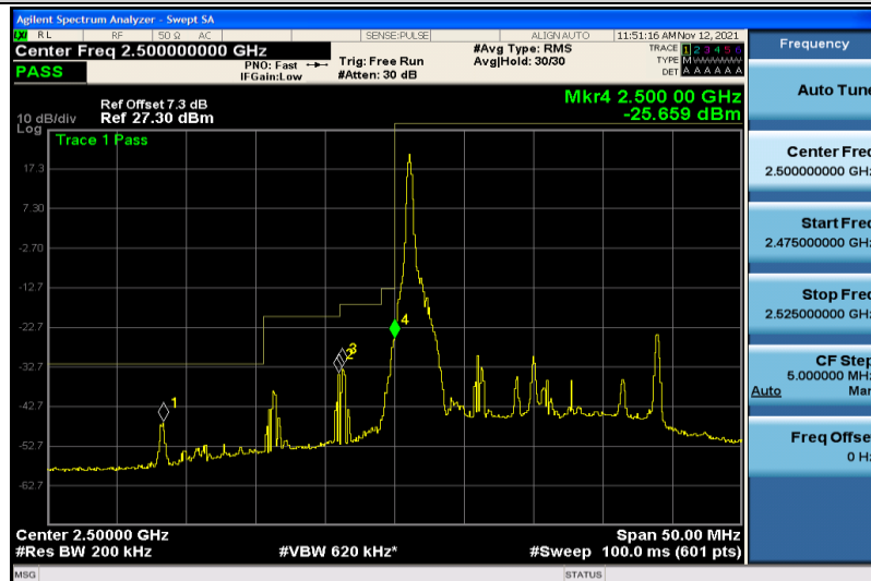
Band7-20MHz-16QAM-20850-1RB#0
