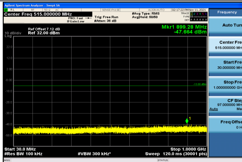
Band4-1.4MHz-16QAM-19957-1RB#0-30~1000MHz
