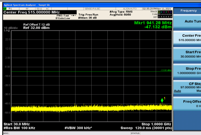
Band4-3MHz-QPSK-20175-1RB#0-30~1000MHz
