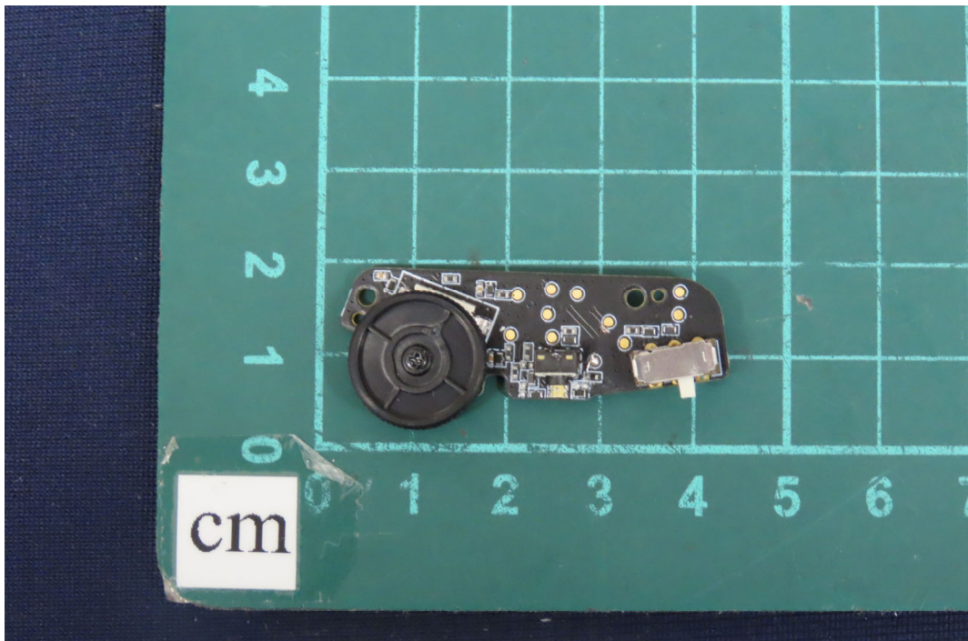
(12) EUT Photo - Brand Name: ASUS, Model No.: A701
