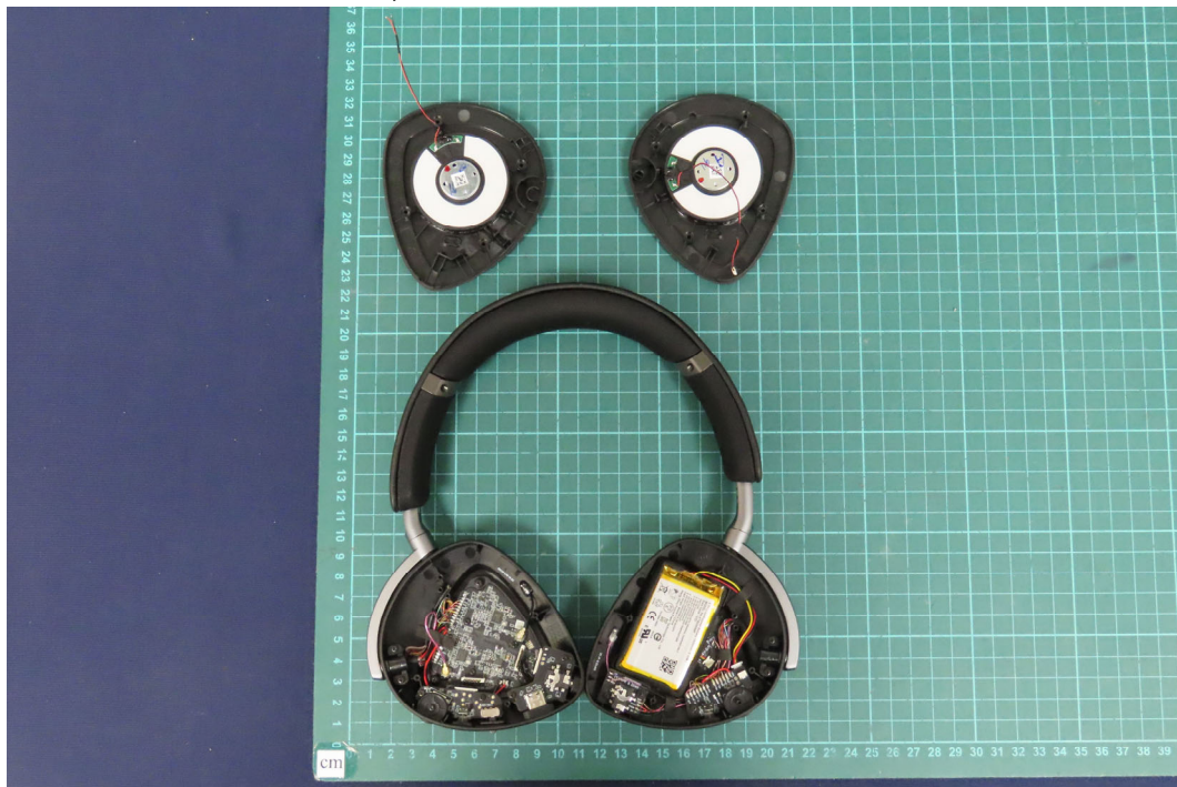
(9) EUT Photo - Brand Name: ASUS, Model No.: A701
