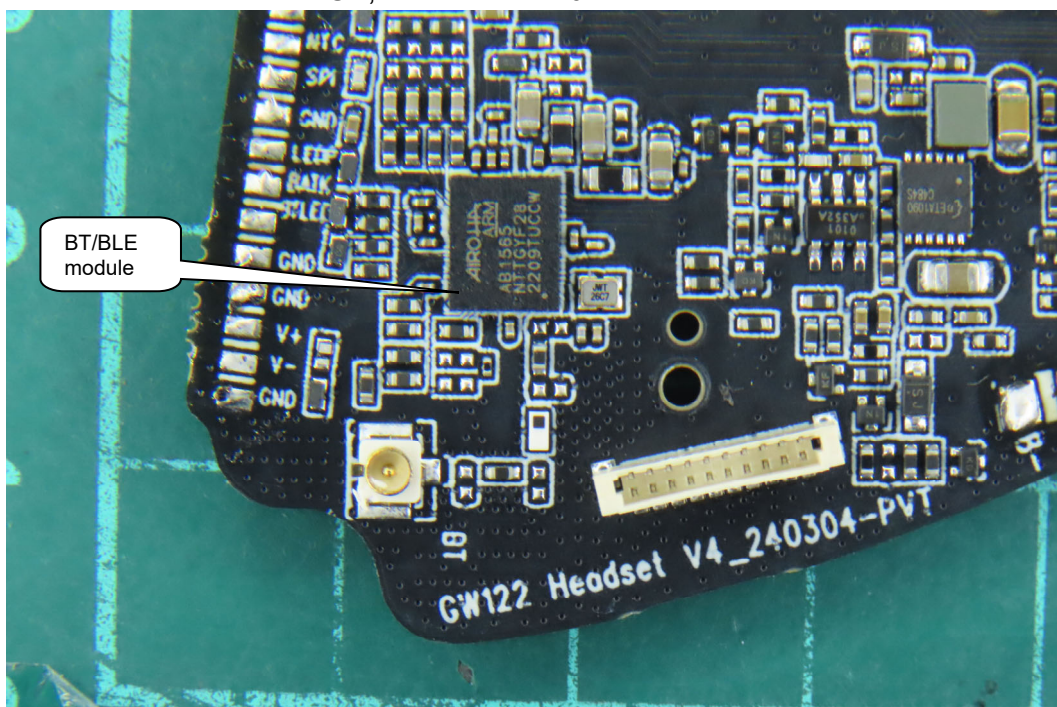
(26) EUT Photo - Brand Name: ASUS, Model No.: A701
