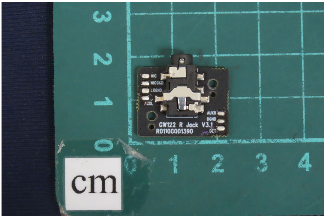
(20) EUT Photo - Brand Name: ASUS, Model No.: A701
