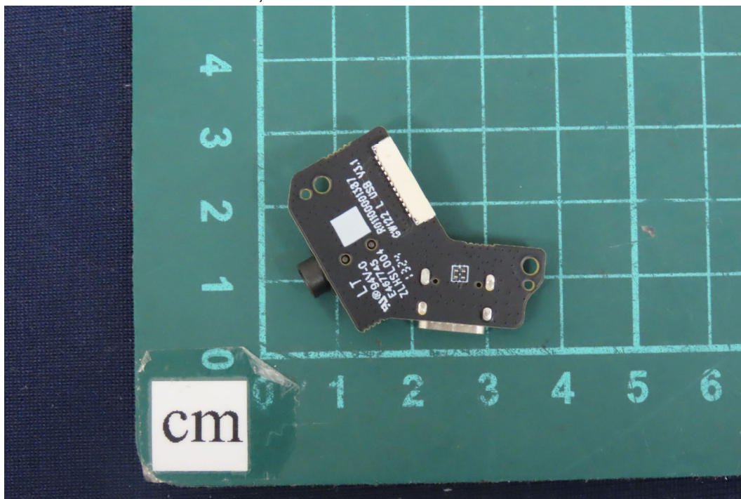
(15) EUT Photo - Brand Name: ASUS, Model No.: A701
