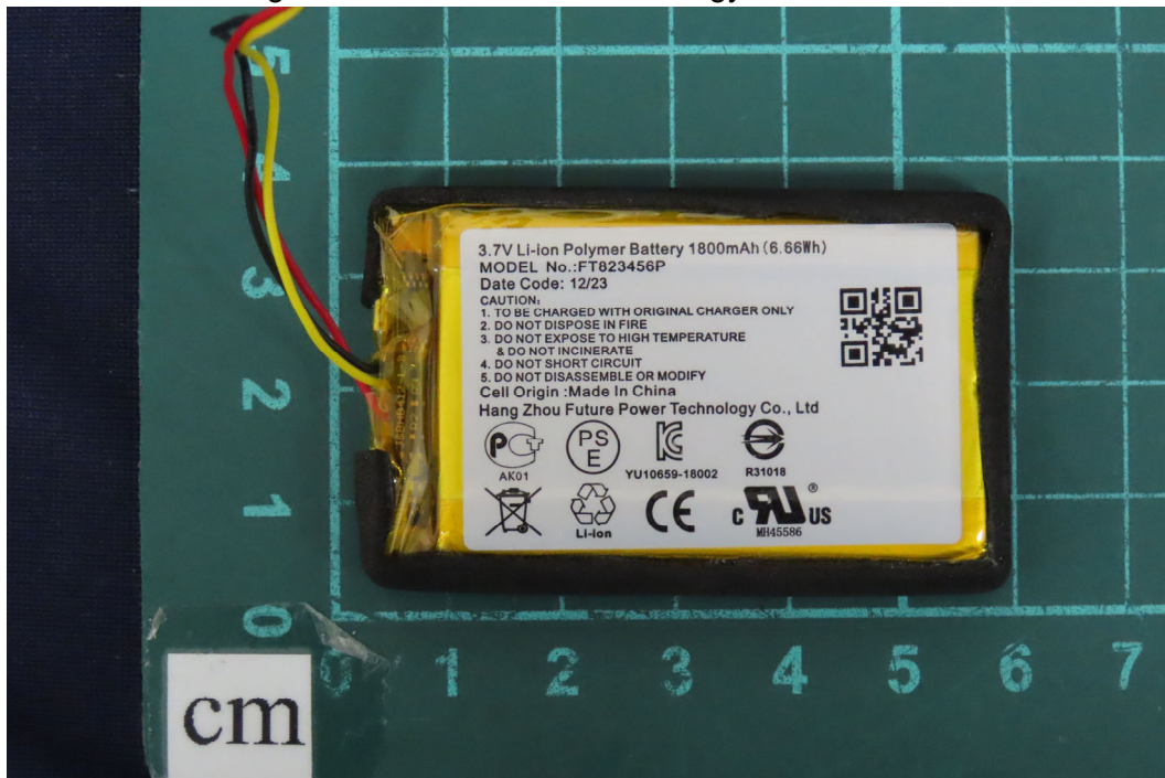
(16) EUT Photo - MFR: Hang Zhou Future Power Technology Co., Ltd, Model No.: FT823456P
