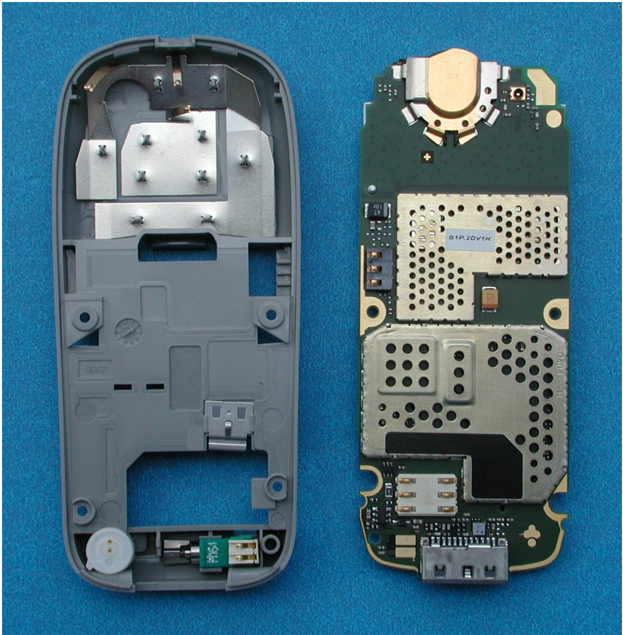
A65 Disassembly step 2
