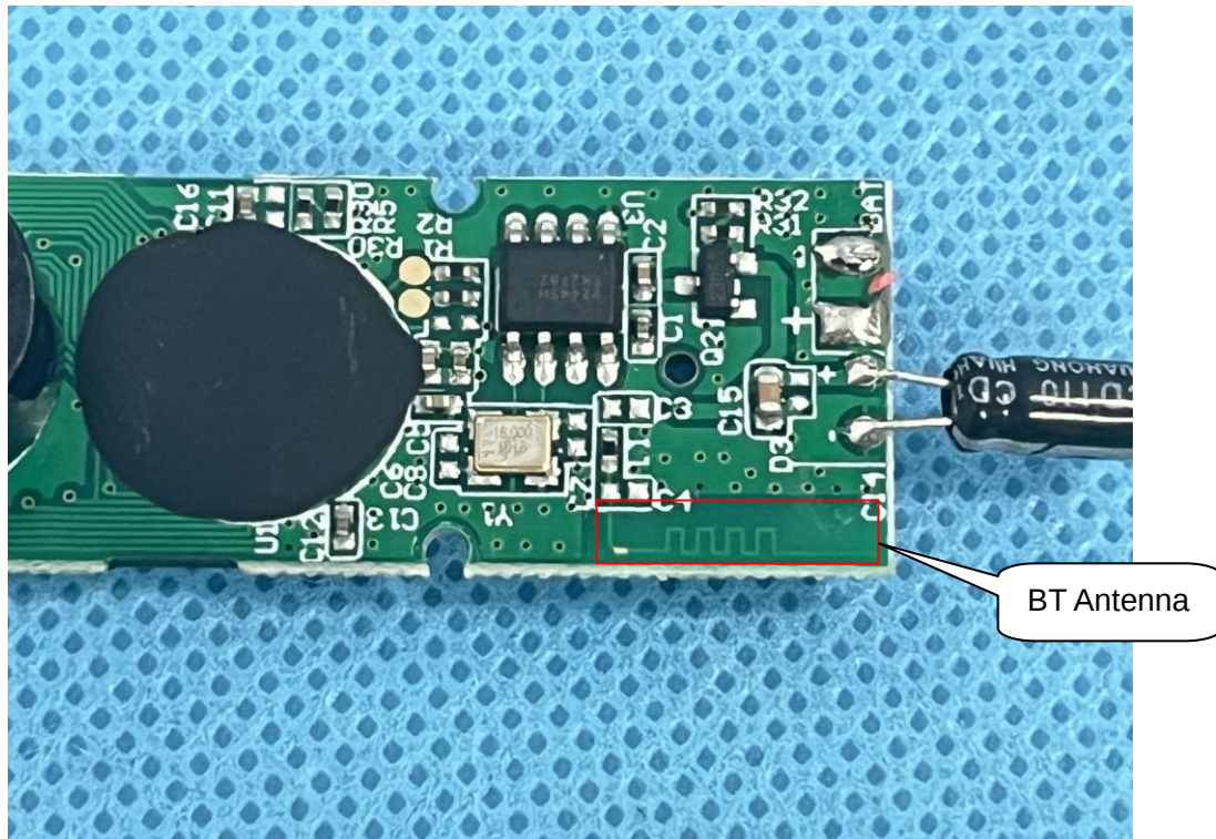
INTERNAL VIEW OF EUT (FIGURE 3)
