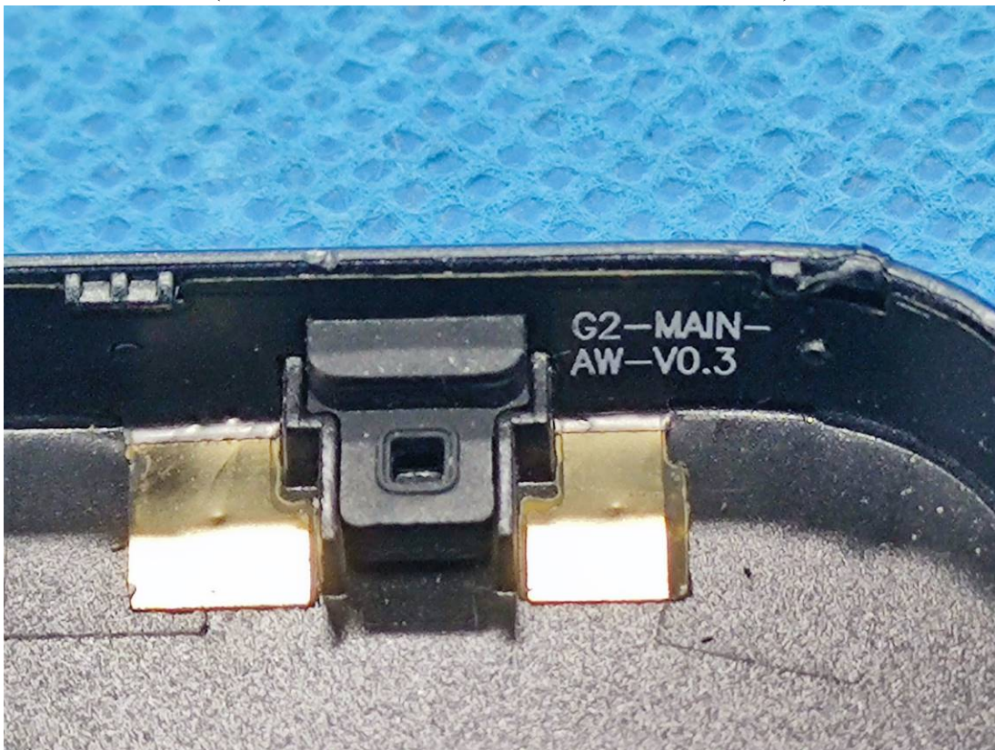
WWAN Main Antenna (TX Band: GSM 850, WCDMA B5, LTE B5/7/12/41)
