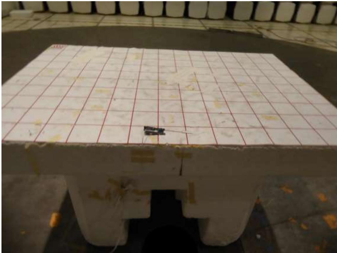
Figure 6 – Radiated Emissions, EUT on Table
