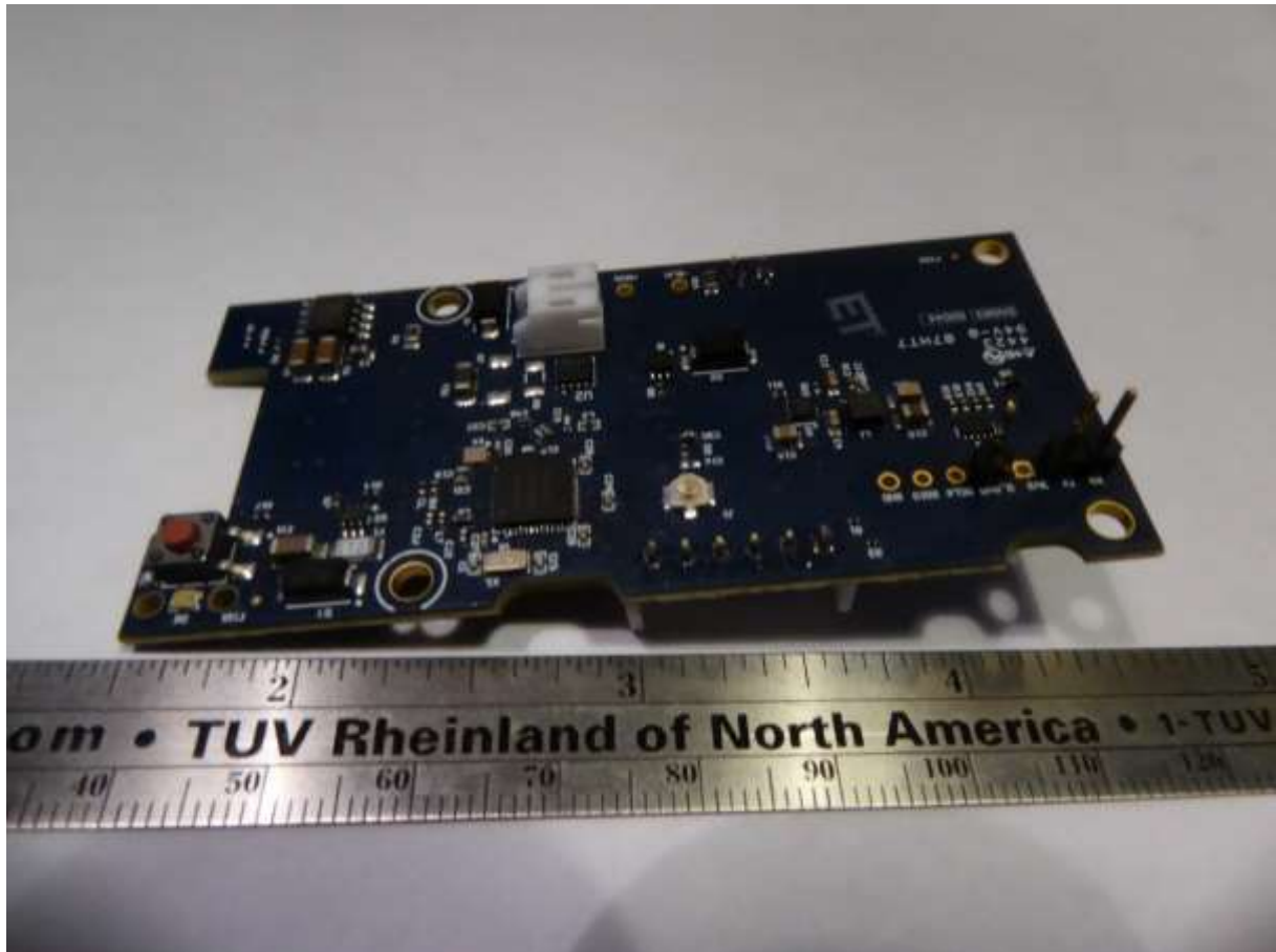
Figure 2 – EUT Top Detail
