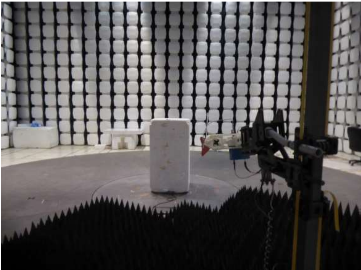
Figure 9 – Radiated Emissions Above 1GHz
