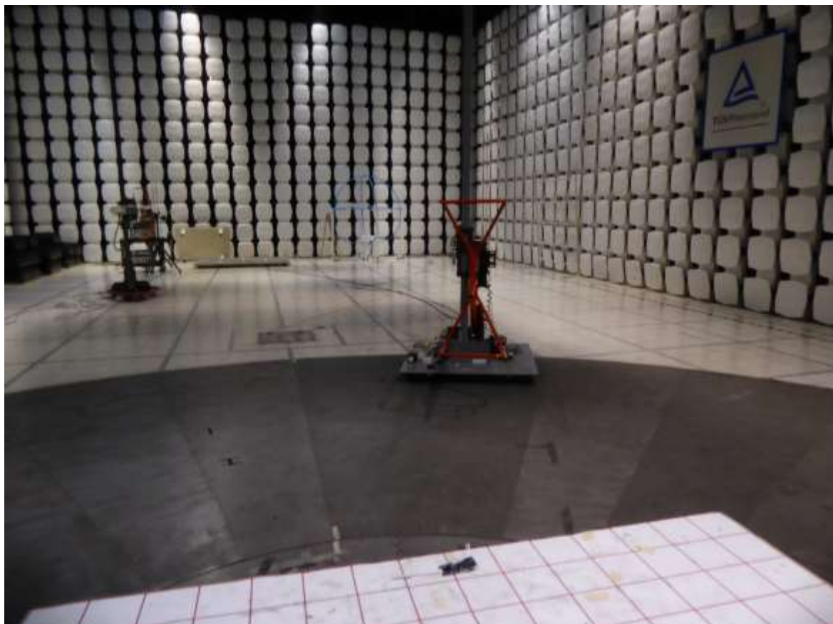
Figure 7 – Radiated Emissions Below 1GHz
