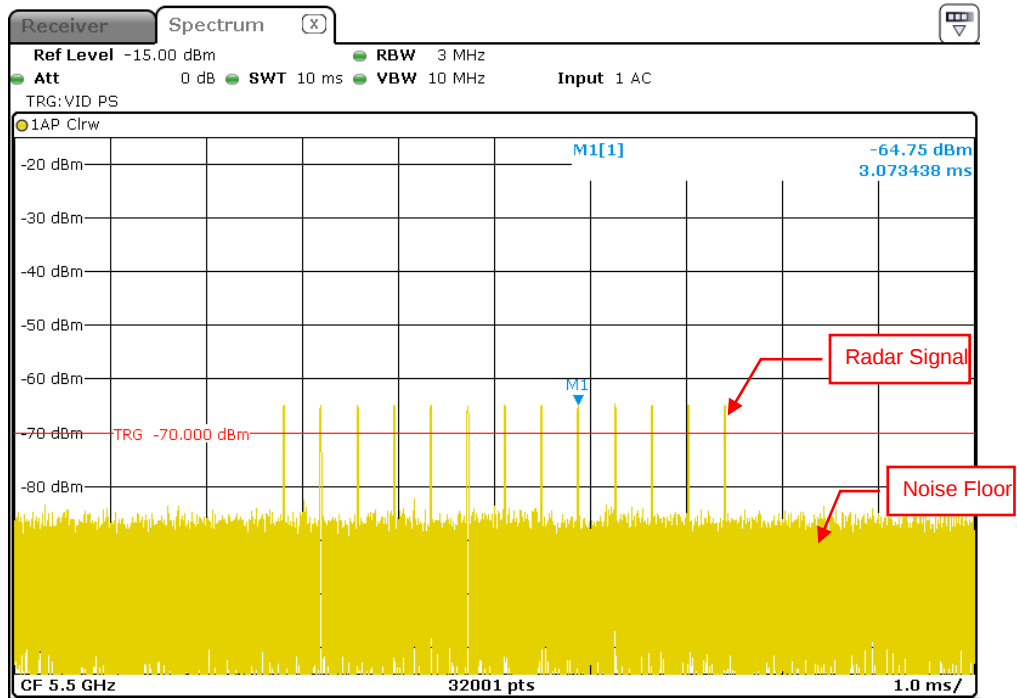
Radar Signal 4
