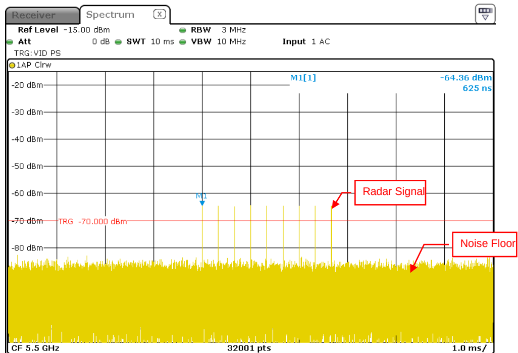
Radar Signal 6
