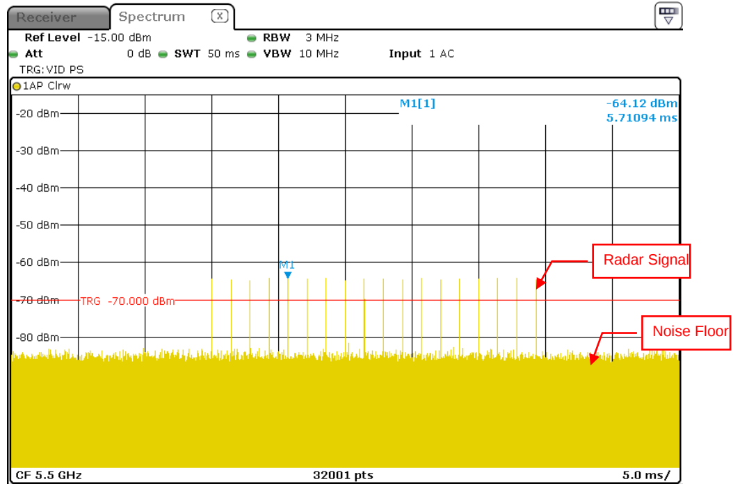
Radar Signal 0
