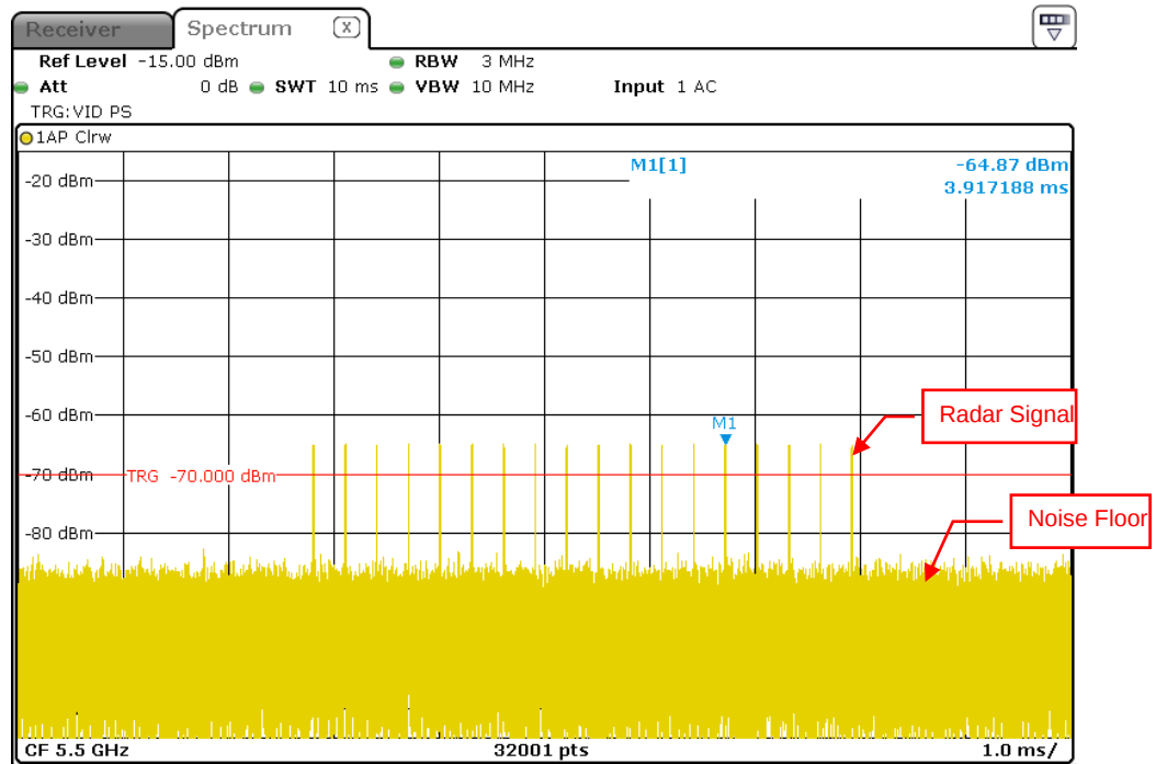
Radar Signal 3
