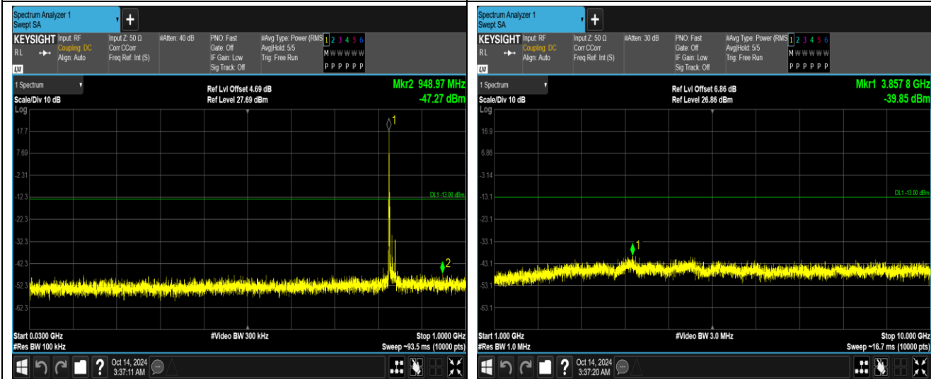
Band26-15MHz-64QAM-26915-1RB#0-Range1:30~1000MHz
