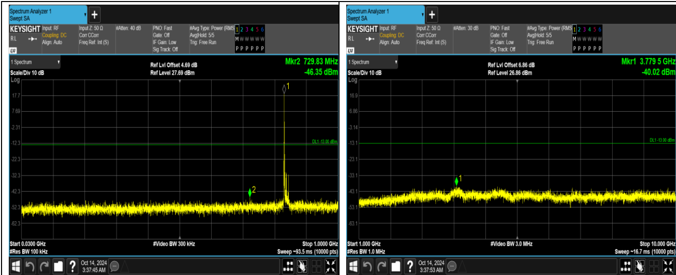
Band26-15MHz-64QAM-26865-1RB#0-Range1:30~1000MHz
