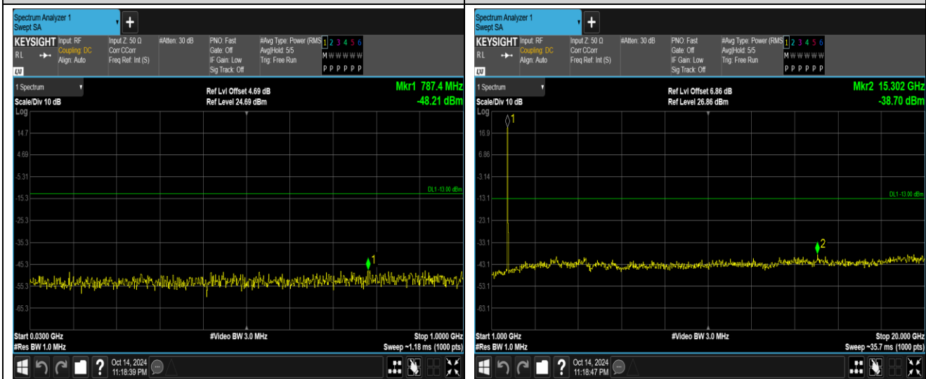
Band66-20MHz-64QAM-132072-1RB#0-Range1:30~1000MHz
