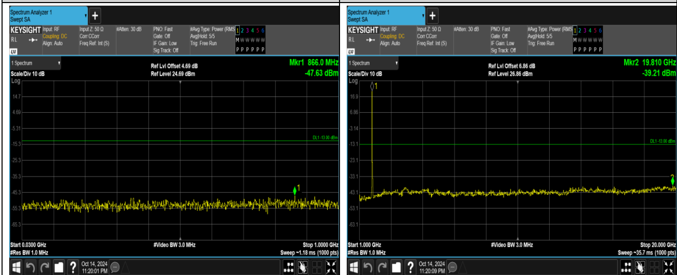
Band66-20MHz-64QAM-132072-1RB#0-Range1:30~1000MHz
