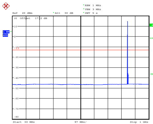
NB-IOT Band 5 CH-High 30MHz-1GHz
