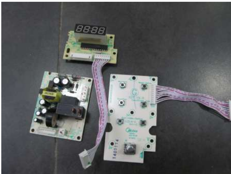
Mother board(Power board+LED display board+ Electronic Keyboard board) - Top View
