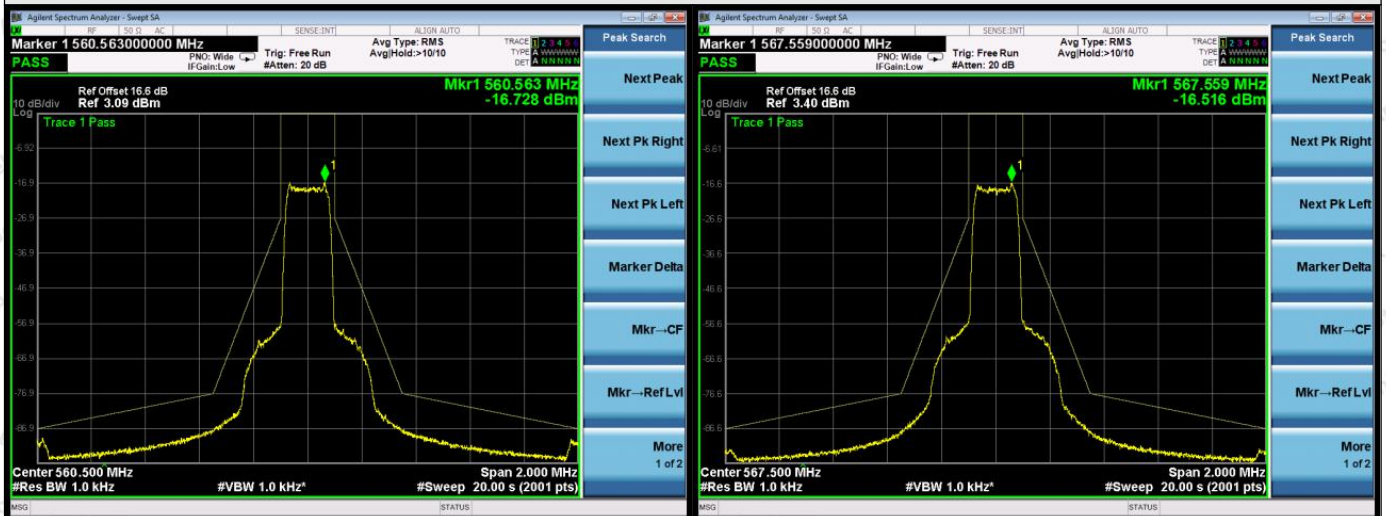
Channel: 560.5MHz
