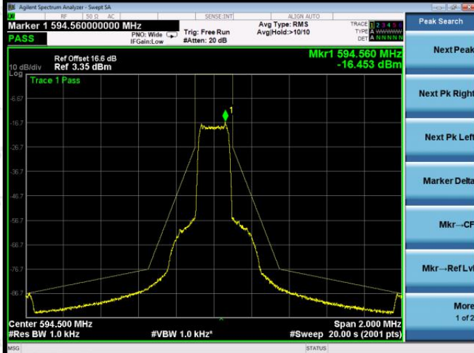
Channel: 594.5MHz
