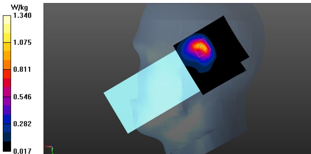
Fig.4 WCDMA Band 4 Head
