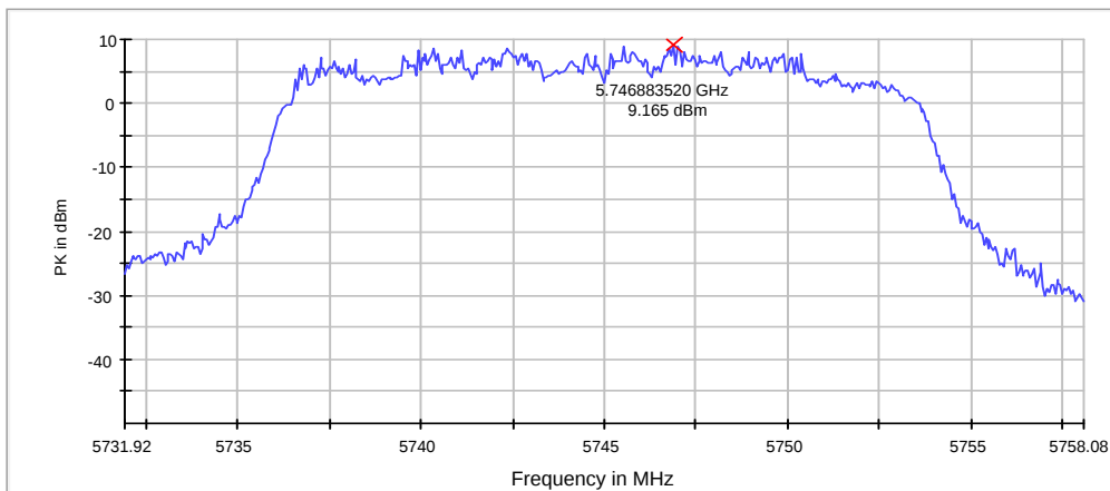
Channel 149 / 5745MHz (RBW: 500 kHz, VBW: 3 MHz)
