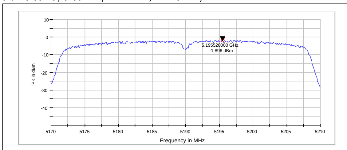
Channel 36+40 / 5190MHz (RBW: 1 MHz, VBW: 3 MHz)
