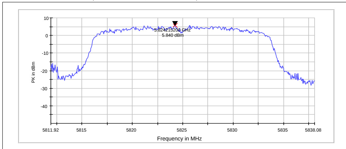
Channel 165 / 5825MHz (RBW: 500 kHz, VBW: 3 MHz)
