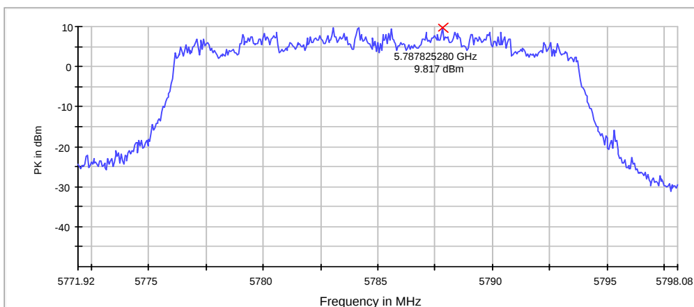
Channel 157 / 5785MHz (RBW: 500 kHz, VBW: 3 MHz)
