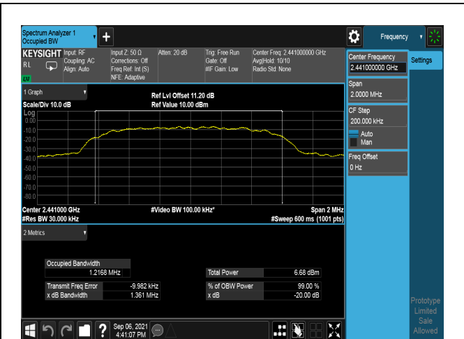
Modulation: 8DPSK 2441MHz
