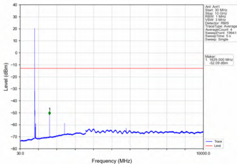
Band26a_10MHz_16QAM_HCH_819MHz_RB_1_0_NTNV
