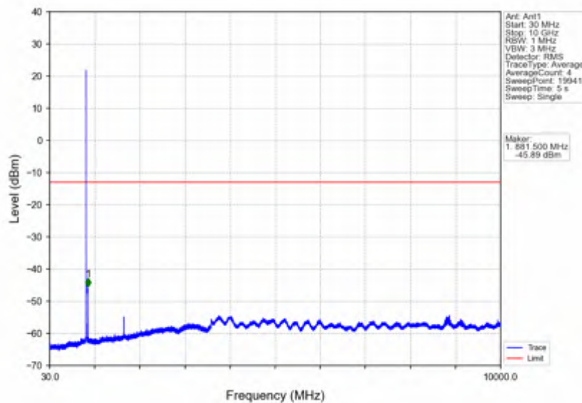
Band26b_5MHz_64QAM_MCH_836.5MHz_RB_1_0_NTNV
