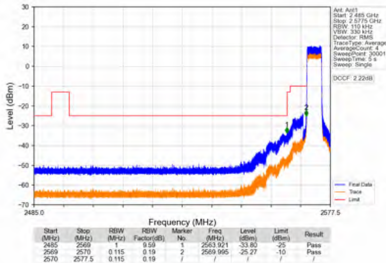
Band38_5MHz_QPSK_LCH_2572.5MHz_RB_25_0_NTNV
