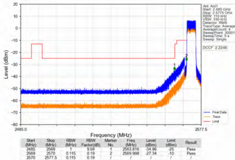
Band38_5MHz_256QAM_LCH_2572.5MHz_RB_25_0_NTNV
