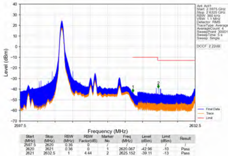
Band38_15MHz_QPSK_HCH_2612.5MHz_RB_1_74_NTNV
