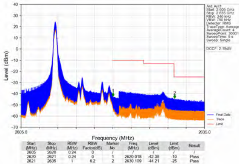
Band38_10MHz_64QAM_HCH_2615MHz_RB_1_49_NTNV
