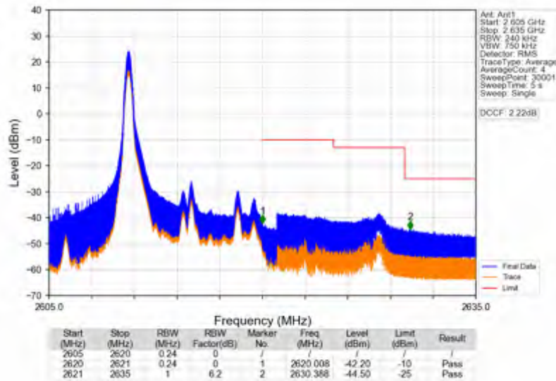
Band38_10MHz_64QAM_HCH_2615MHz_RB_50_0_NTNV
