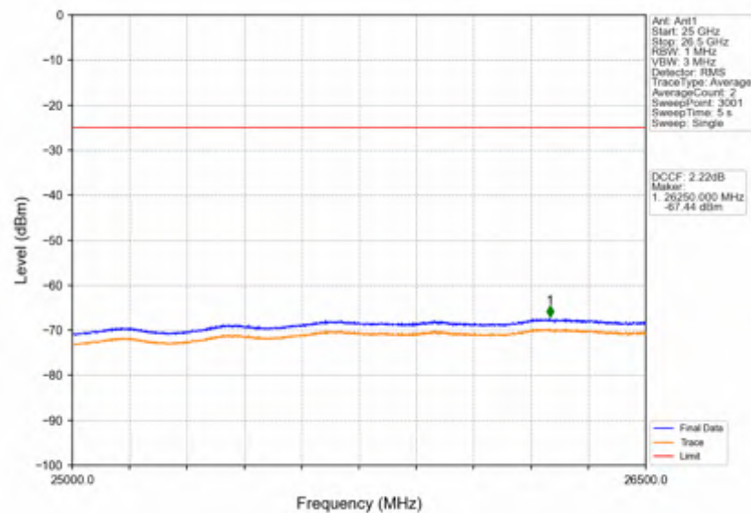
Band38_5MHz_64QAM_HCH_2617.5MHz_RB_1_24_NTNV
