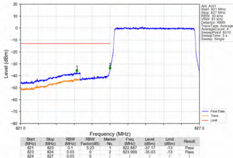
Band26b_3MHz_256QAM_LCH_825.5MHz_RB_15_0_NTNV
