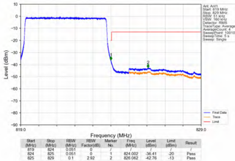
Band26a_5MHz_256QAM_HCH_821.5MHz_RB_25_0_NTNV
