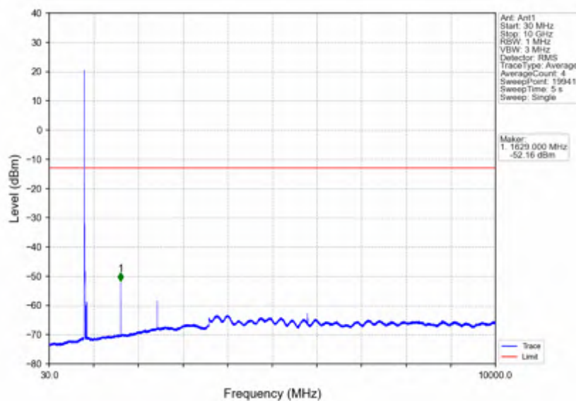
Band26a_10MHz_64QAM_MCH_819MHz_RB_1_0_NTNV
