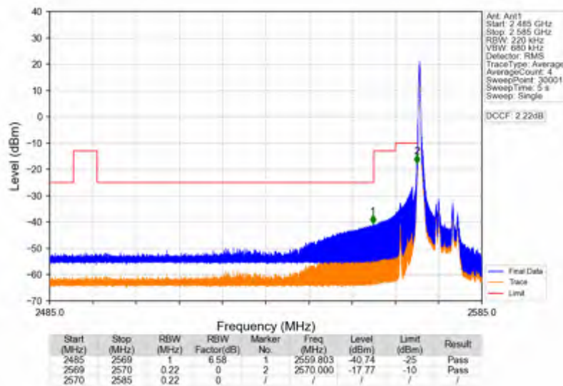
Band38 10MHz 256QAM LCH 2575MHz RB 1 0 NTNV
