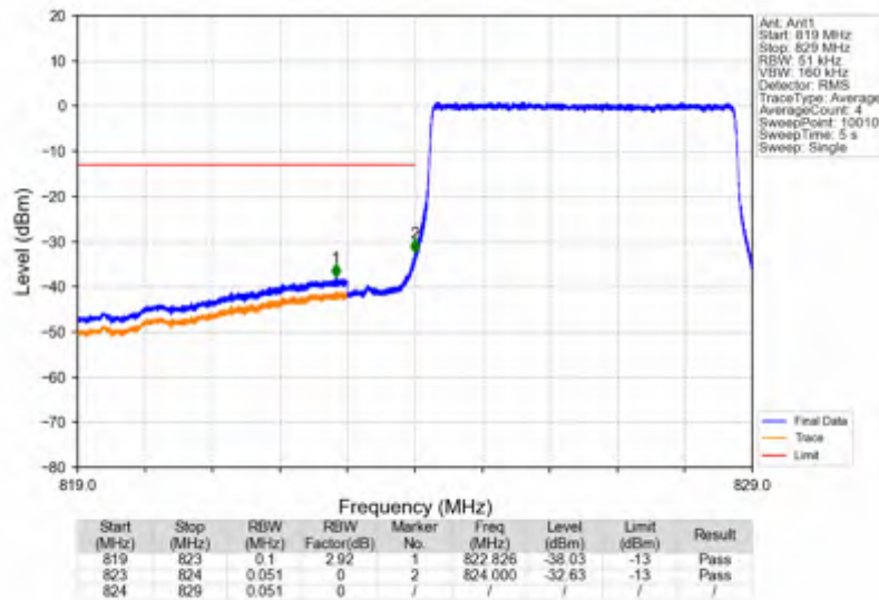
Band26b_5MHz_256QAM_LCH_826.5MHz_RB_25_0_NTNV
