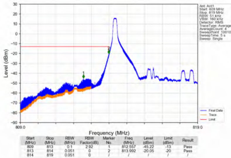
Band26a_5MHz_QPSK_LCH_816.5MHz_RB_25_0_NTNV
