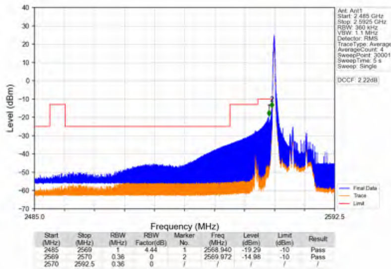
Band38_15MHz_QPSK_LCH_2577.5MHz_RB_1_0_NTNV
