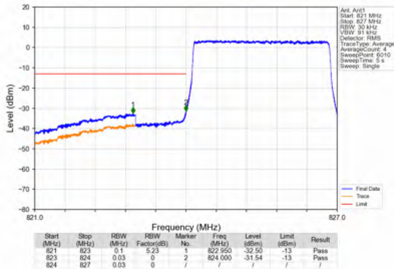
Band26b_3MHz_16QAM_LCH_825.5MHz_RB_15_0_NTNV
