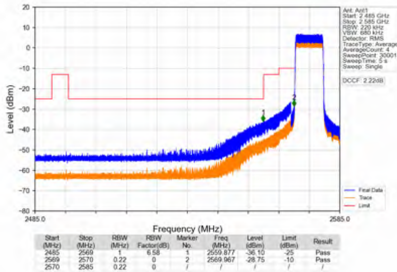
Band38_10MHz_256QAM_LCH_2575MHz_RB_50_0_NTNV
