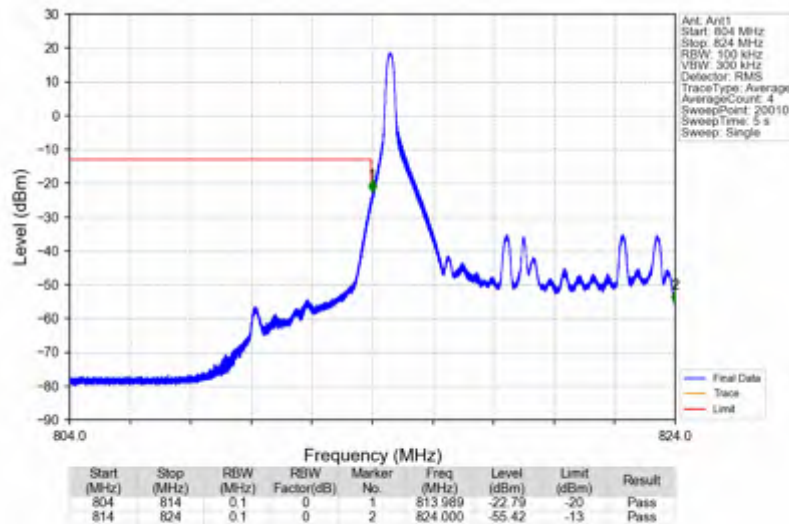
Band26a_10MHz_16QAM_LCH_819MHz_RB_50_0_NTNV
