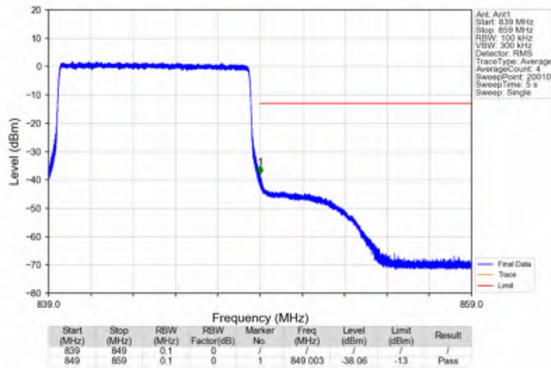
Band26b_10MHz_256QAM_HCH_844MHz_RB_50_0_NTNV
