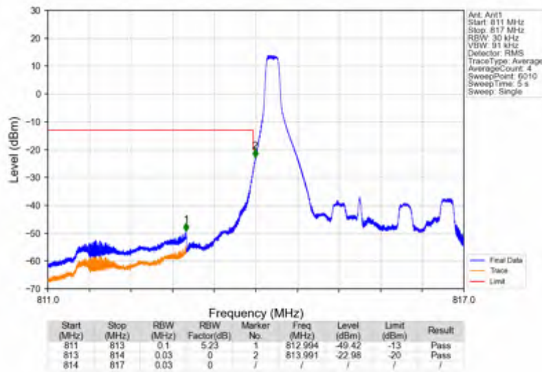
Band26a_3MHz_QPSK_LCH_815.5MHz_RB_1_0_NTNV
