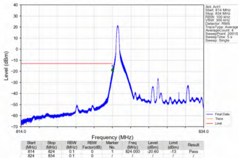
Band26b_10MHz_16QAM_LCH_829MHz_RB_1_0_NTNV
