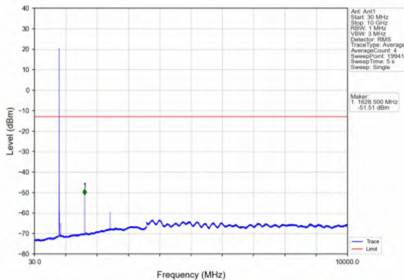
Band26a 3MHz 64QAM LCH 815.5MHz RB_1_0 NTNv
