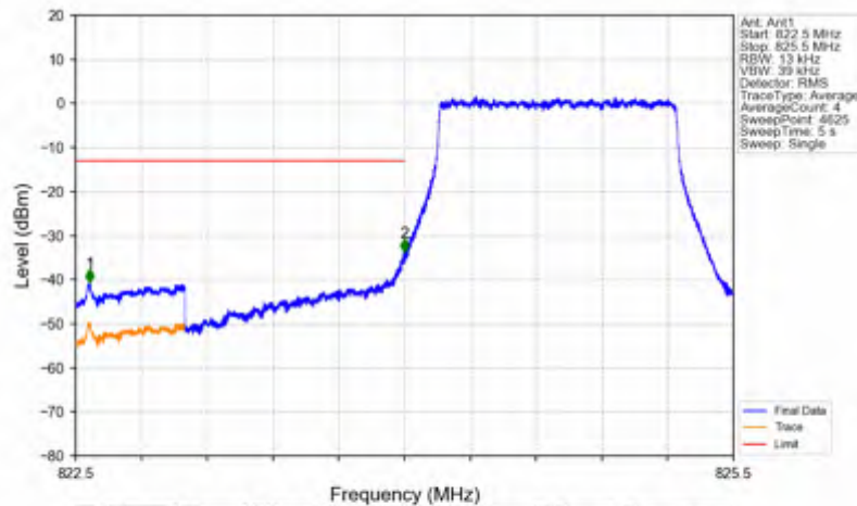
Band26b_1.4MHz_256QAM_LCH_824.7MHz_RB_6_0_NTNV
