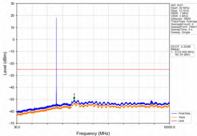
Band38_5MHz_256QAM_HCH_2617.5MHz_RB_1_0_NTNV
