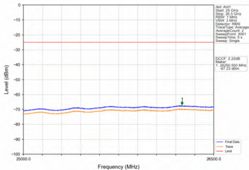
Band38_10MHz_64QAM_HCH_2615MHz_RB_1_49_NTNV
