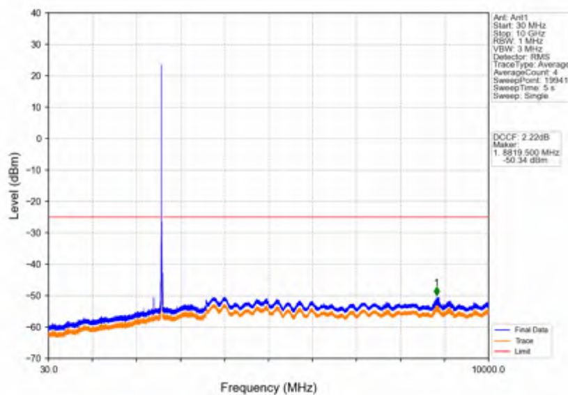
Band38_15MHz_QPSK_MCH_2595MHz_RB_1_0_NTNV
