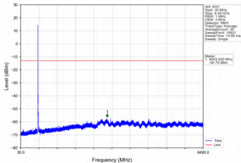
Band26c_15MHz_64QAM_LCH_831.5MHz_RB_1_0_NTNV
