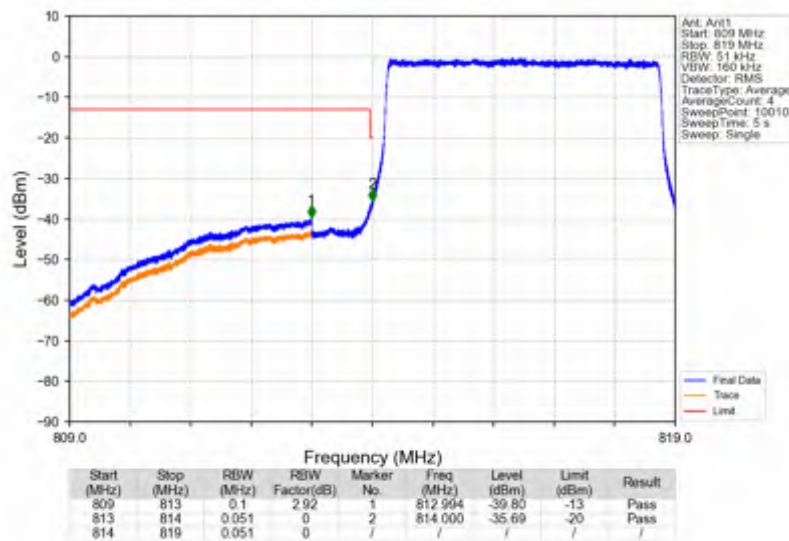
Band26a_5MHz_256QAM_LCH_816.5MHz_RB_25_0_NTNV
