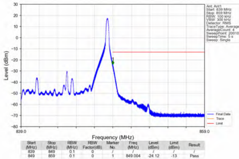
Band26b_10MHz_256QAM_HCH_844MHz_RB_1_49_NTNV
