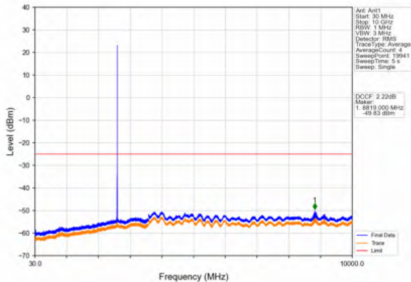
Band38_5MHz_16QAM_HCH_2617.5MHz_RB_1_0_NTNV
