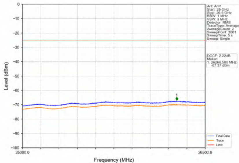
Band38_5MHz_16QAM_HCH_2617.5MHz_RB_1_0_NTNV
