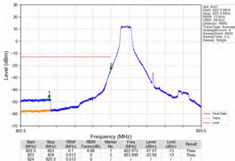
Band26b_1.4MHz_16QAM_LCH_824.7MHz_RB_1_0_NTNV
