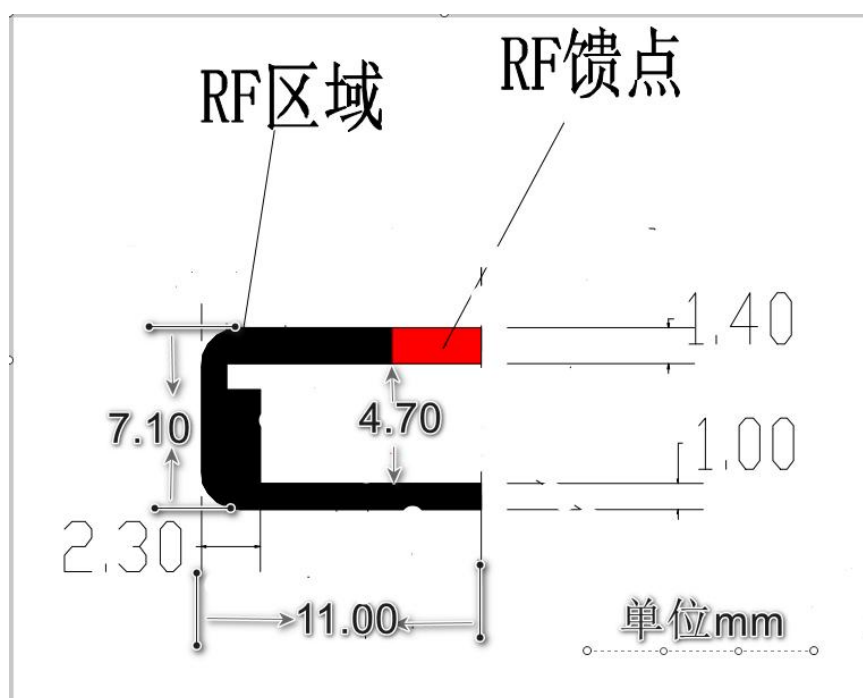
(a) FPC antenna
