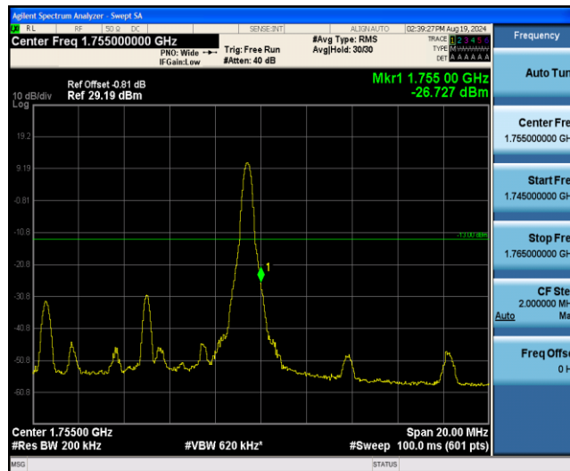
Band4-10MHz-QPSK-20350-27RB#0
