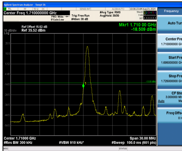
Band4-15MHz-16QAM-20025-27RB#0
