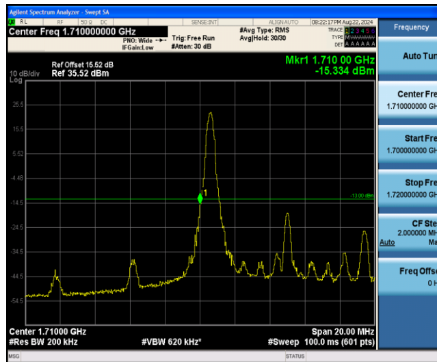
Band4-10MHz-16QAM-20000-1RB#49
