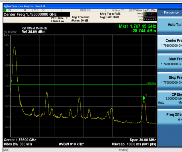
Band4-15MHz-16QAM-20325-27RB#0
