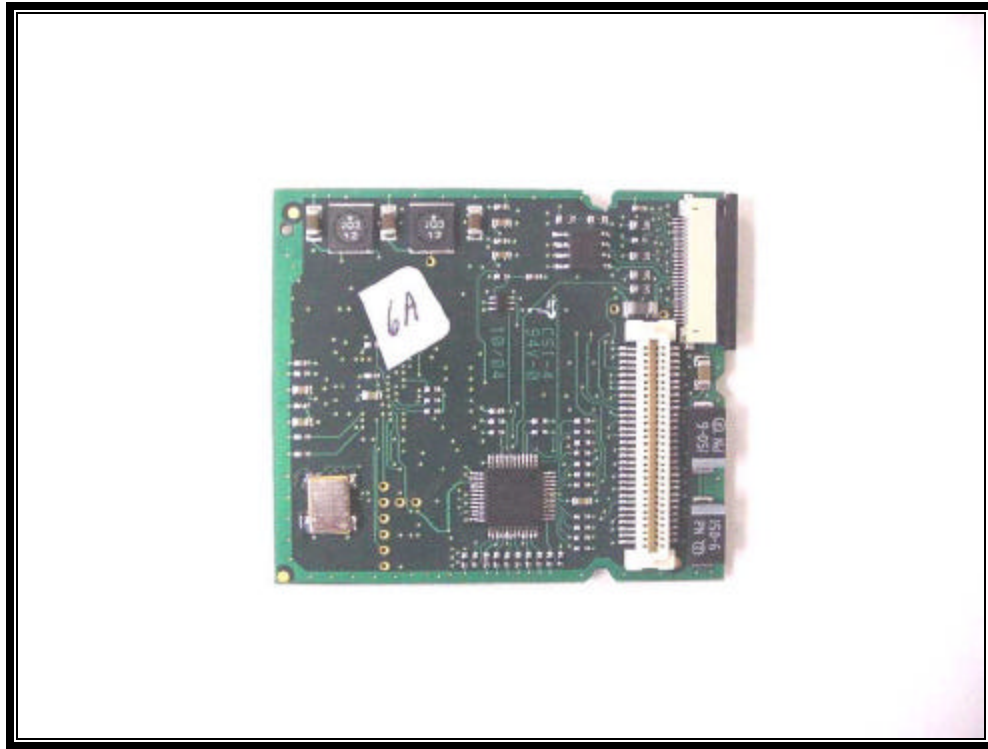
PHOTOGRAPH 23: LOGIC PCB FRONT
