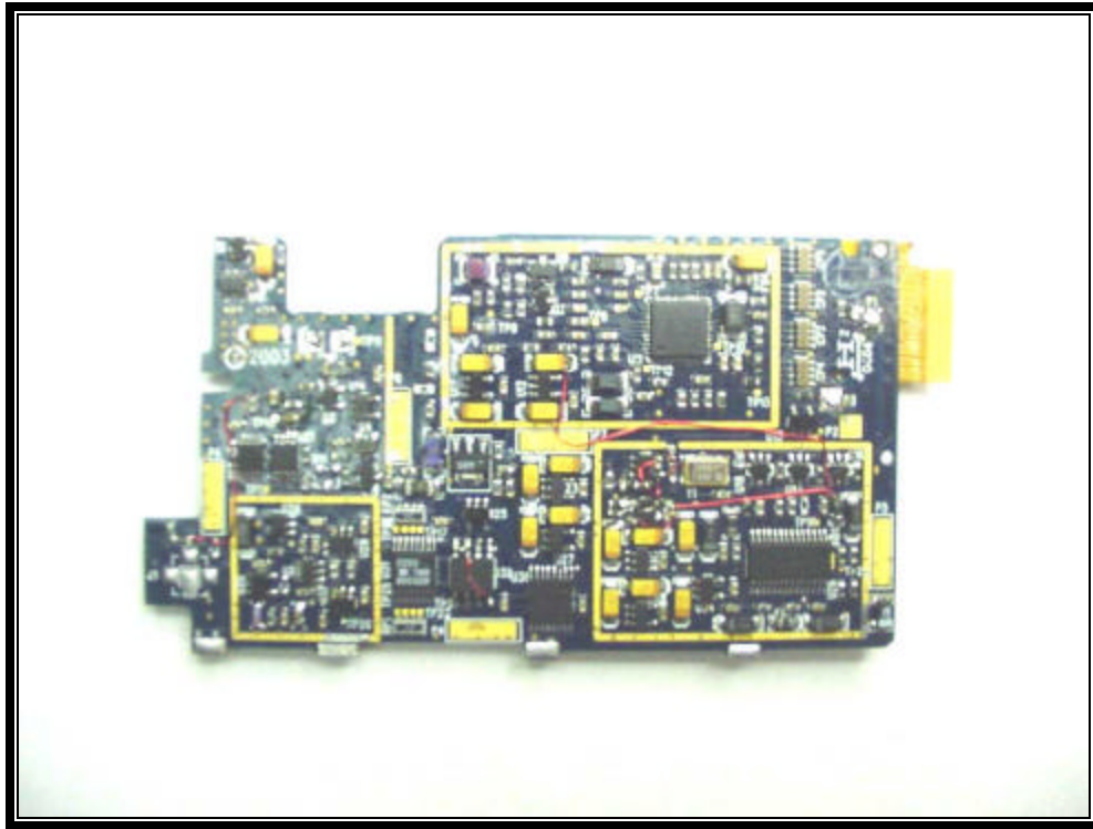
PHOTOGRAPH 26: RF BOARD BACK WITHOUT SHIELDS
