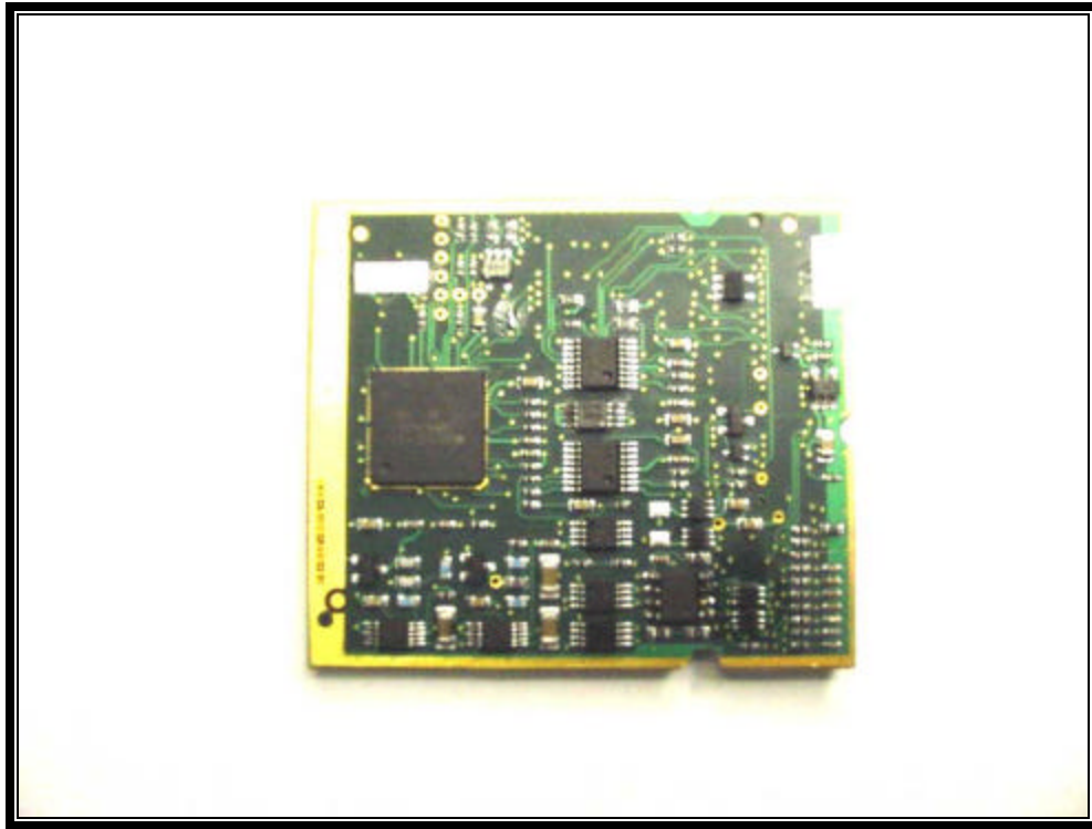
PHOTOGRAPH 24: LOGIC PCB BACK
