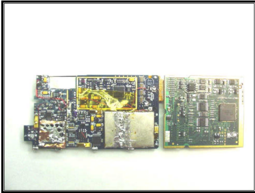
PHOTOGRAPH 27: RF LOGIC WITH SHIELDS
