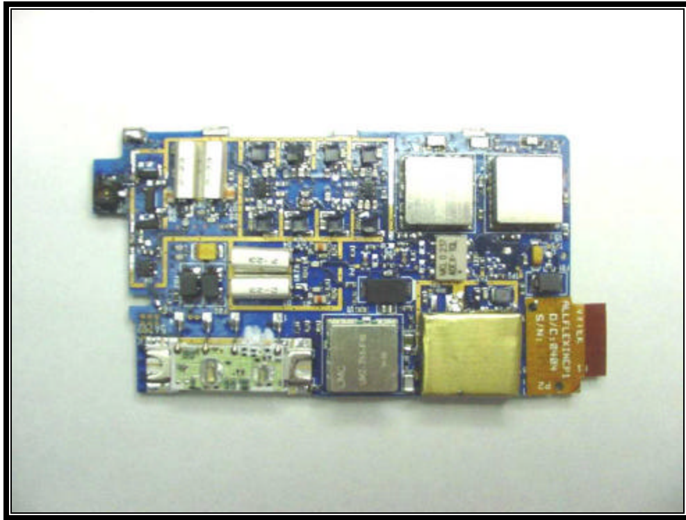
PHOTOGRAPH 25: RF BOARD FRONT WITHOUT SHIELDS
