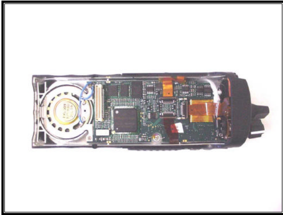
PHOTOGRAPH 28: UI IN HOUSING
