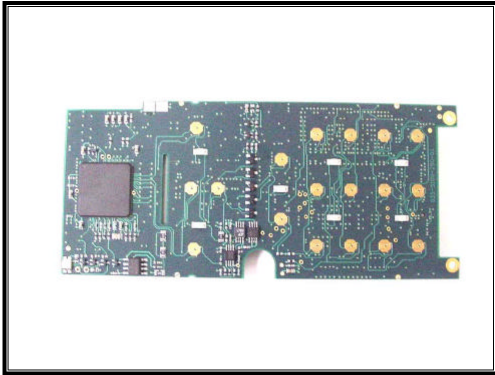
PHOTOGRAPH 29: UI FRONT
