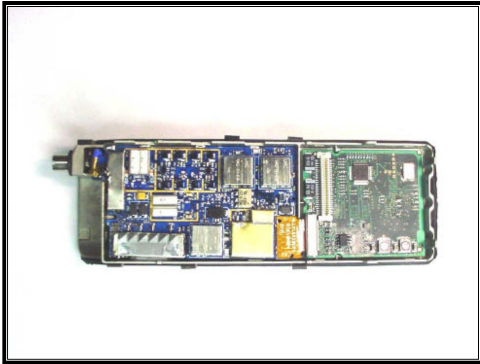
PHOTOGRAPH 22: CHASSIS WITHOUT SHIELDS
