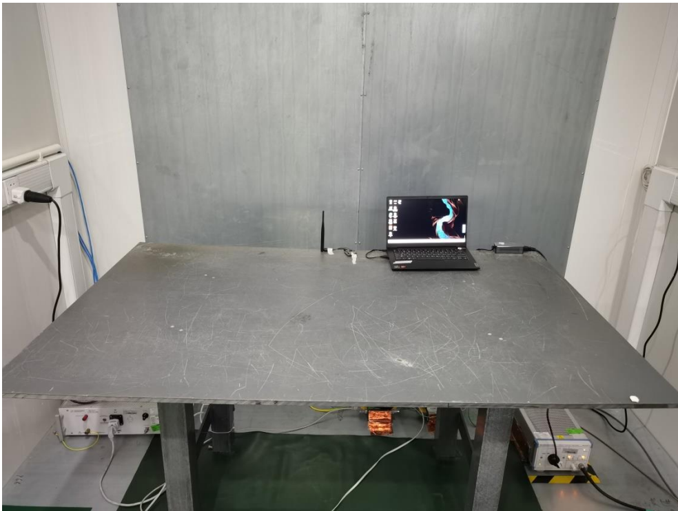
AC Power Line Conducted Emissions Test Photos (BT)
