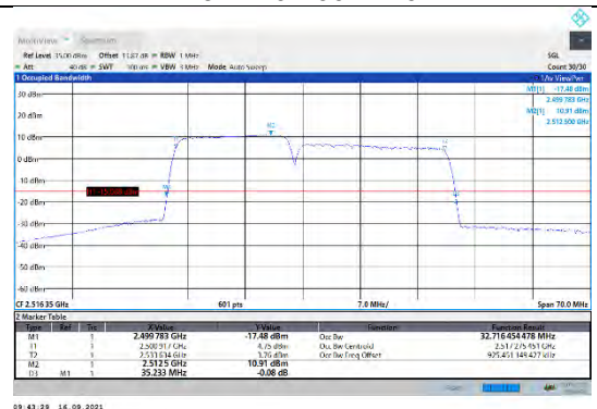
CA_7C-15MHz-20MHz-16QAM-16QAM-20828-20999-75RB#0-100RB#0
