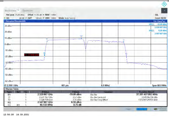
CA_7C-20MHz-20MHz-16QAM-16QAM-21152-21350-100RB#0-100RB#0
