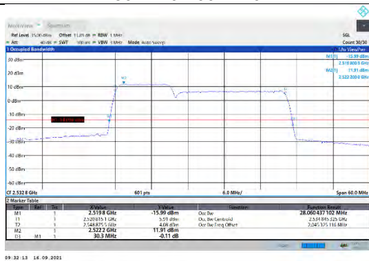
CA_7C-10MHz-20MHz-QPSK-QPSK-21006-21150-50RB#0-100RB#0
