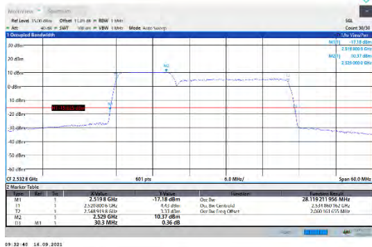
CA_7C-10MHz-20MHz-16QAM-16QAM-21006-21150-50RB#0-100RB#0
