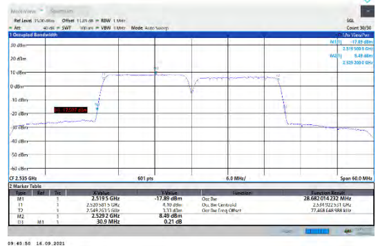
CA_7C-15MHz-15MHz-16QAM-16QAM-21025-21175-75RB#0-75RB#0
