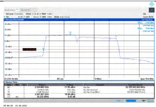
CA_7C-15MHz-20MHz-16QAM-16QAM-21179-21350-75RB#0-100RB#0
