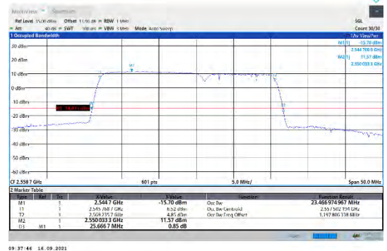
CA_7C-15MHz-10MHz-QPSK-QPSK-21277-2139CA_7C5RB#0-50RB#0
