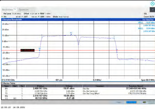
CA_7C-20MHz-20MHz-QPSK-QPSK-20850-21048-100RB#0-100RB#0
