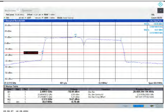
CA_7C-15MHz-15MHz-16QAM-16QAM-20825-20975-75RB#0-75RB#0
