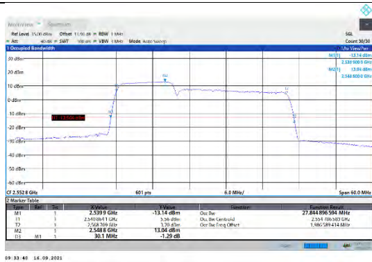
CA_7C-10MHz-20MHz-QPSK-QPSK-21206-21350-50RB#0-100RB#0
