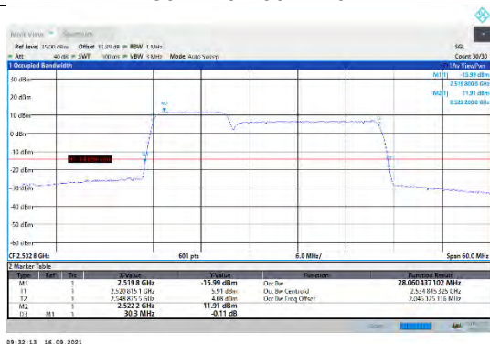
CA_7C-10MHz-20MHz-QPSK-QPSK-21006-21150-50RB#0-100RB#0
