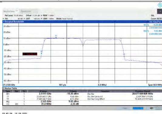
CA_7C-15MHz-15MHz-QPSK-QPSK-21025-21175-75RB#0-75RB#0
