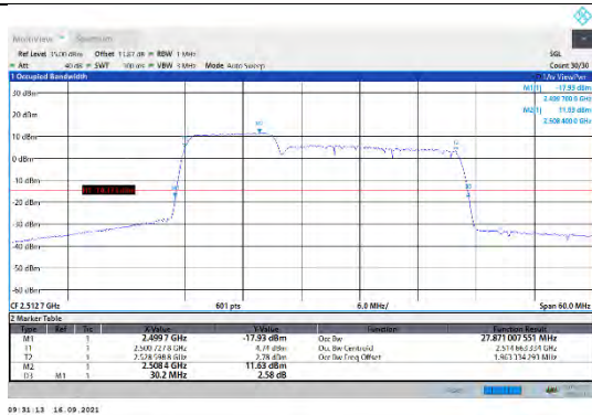
CA_7C-10MHz-20MHz-16QAM-16QAM-20805-20949-50RB#0-100RB#0
