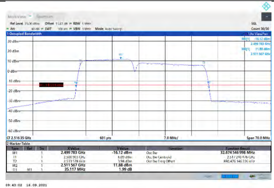
CA_7C-15MHz-20MHz-QPSK-QPSK-20828-20999-75RB#0-100RB#0
