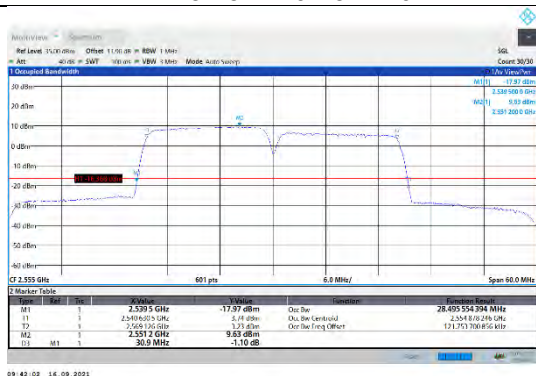
CA_7C-15MHz-15MHz-16QAM-16QAM-21225-21375-75RB#0-75RB#0
