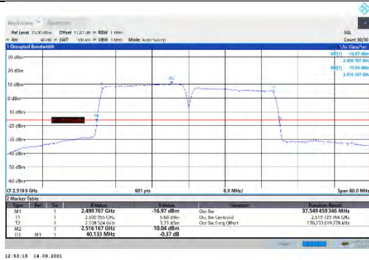
CA_7C-20MHz-20MHz-QPSK-QPSK-20850-21048-100RB#0-100RB#0
