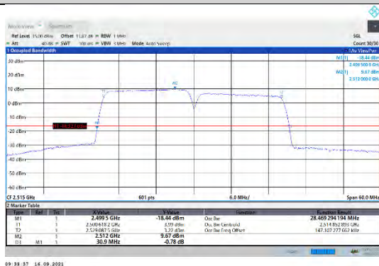
CA_7C-15MHz-15MHz-16QAM-16QAM-20825-20975-75RB#0-75RB#0
