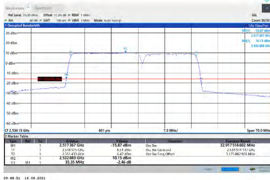
CA_7C-20MHz-15MHz-16QAM-16QAM-21026-21197-100RB#0-75RB#0
