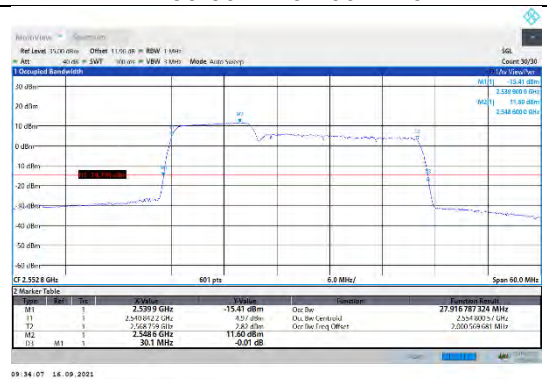
CA_7C-10MHz-20MHz-16QAM-16QAM-21206-21350-50RB#0-100RB#0
