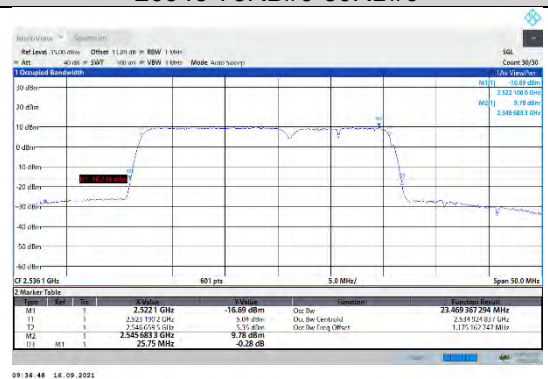
CA_7C-15MHz-10MHz-16QAM-16QAM-21051-21171-75RB#0-50RB#0
