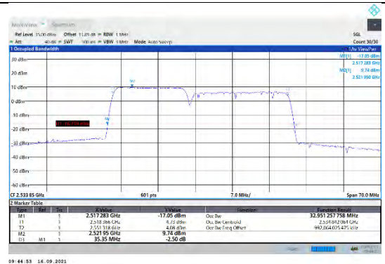
CA_7C-15MHz-20MHz-16QAM-16QAM-21003-21174-75RB#0-100RB#0
