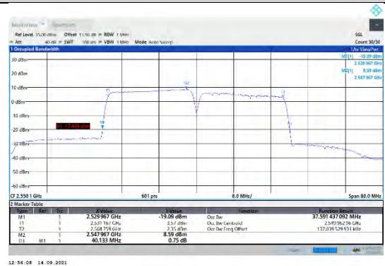
CA_7C-20MHz-20MHz-16QAM-16QAM-21152-21350-100RB#0-100RB#0
