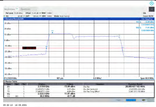
CA_7C-10MHz-20MHz-QPSK-QPSK-21006-21150-50RB#0-100RB#0
