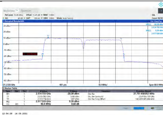
CA_7C-20MHz-20MHz-QPSK-QPSK-21001-21199-100RB#0-100RB#0
