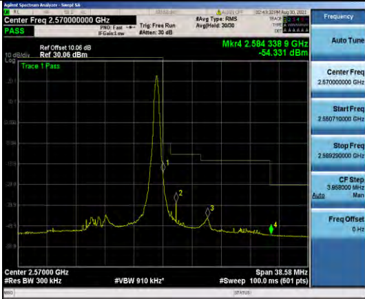
Band7-15MHz-16QAM-21375-75RB#0
