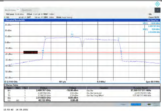
CA_7C-20MHz-20MHz-16QAM-16QAM-20850-21048-100RB#0-100RB#0
