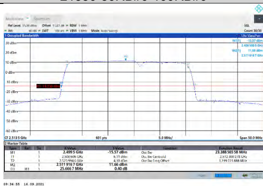
CA_7C-15MHz-10MHz-QPSK-QPSK-20825-20945-75RB#0-50RB#0
