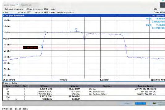
CA_7C-15MHz-15MHz-QPSK-QPSK-20825-20975-75RB#0-75RB#0
