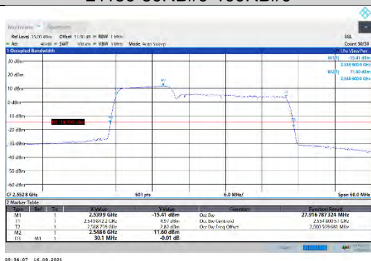
CA_7C-10MHz-20MHz-16QAM-16QAM-21206-21350-50RB#0-100RB#0
