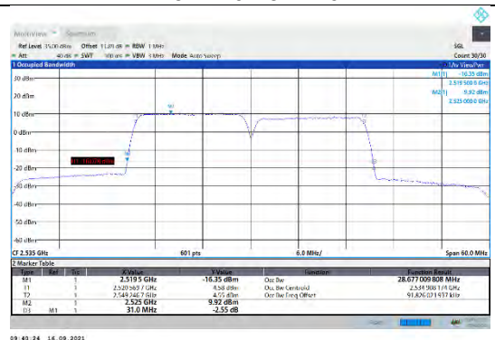
CA_7C-15MHz-15MHz-QPSK-QPSK-21025-21175-75RB#0-75RB#0
