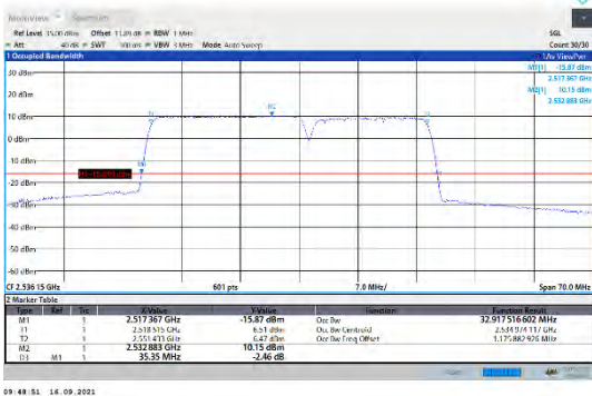
CA_7C-20MHz-15MHz-16QAM-16QAM-21026-21197-100RB#0-75RB#0
