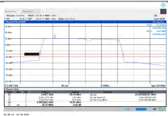
CA_7C-15MHz-10MHz-16QAM-16QAM-21277-2139CA_7C5RB#0-50RB#0
