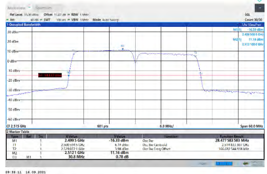
CA_7C-15MHz-15MHz-QPSK-QPSK-20825-20975-75RB#0-75RB#0
