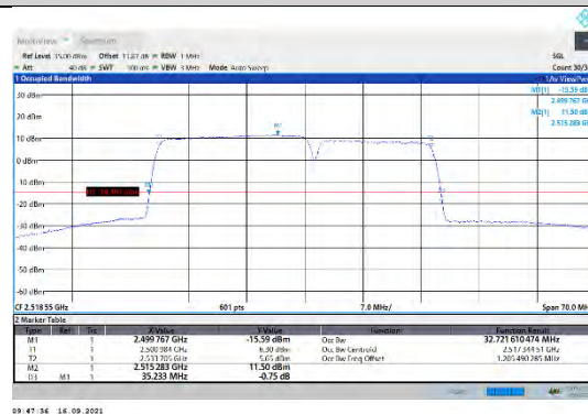
CA_7C-20MHz-15MHz-16QAM-16QAM-20850-21021-100RB#0-75RB#0
