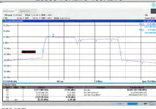
CA_7C-15MHz-20MHz-16QAM-16QAM-21003-21174-75RB#0-100RB#0
