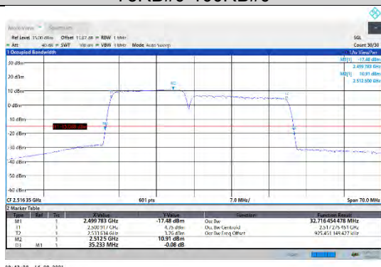
CA_7C-15MHz-20MHz-16QAM-16QAM-20828-20999-75RB#0-100RB#0
