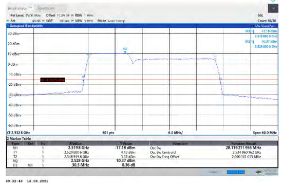
CA_7C-10MHz-20MHz-16QAM-16QAM-21150-50RB#0-100RB#0
