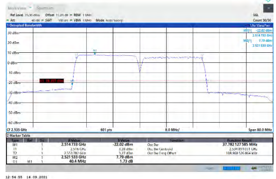
CA_7C-20MHz-20MHz-16QAM-16QAM-21001-21199-100RB#0-100RB#0
