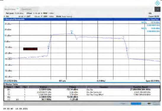
CA_7C-10MHz-20MHz-QPSK-QPSK-21206-21350-50RB#0-100RB#0
