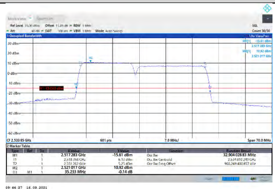
CA_7C-15MHz-20MHz-QPSK-QPSK-21003-21174-75RB#0-100RB#0
