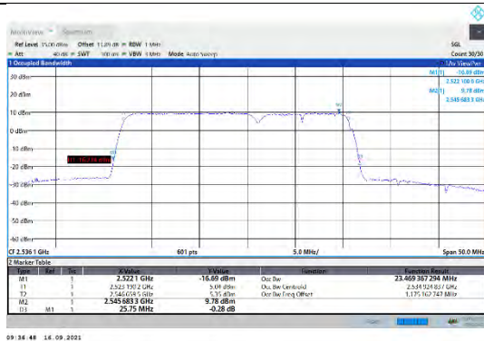
CA_7C-15MHz-10MHz-16QAM-16QAM-21051-21171-75RB#0-50RB#0
