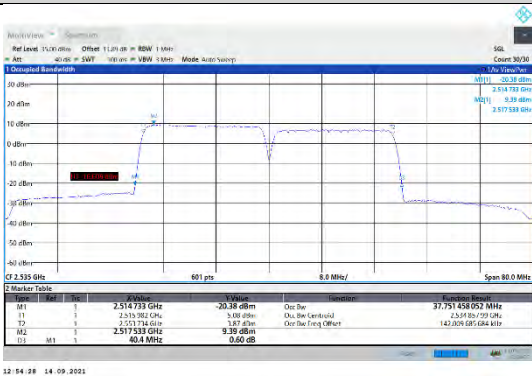
CA_7C-20MHz-20MHz-QPSK-QPSK-21001-21199-100RB#0-100RB#0
