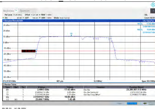
CA_7C-15MHz-10MHz-16QAM-16QAM-20825-20945-75RB#0-50RB#0
