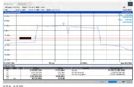
CA_7C-20MHz-20MHz-QPSK-QPSK-21152-21350-100RB#0-100RB#0
