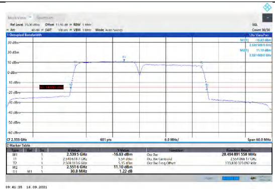
CA_7C-15MHz-15MHz-QPSK-QPSK-21225-21375-75RB#0-75RB#0
