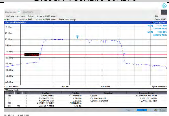
CA_7C-15MHz-10MHz-16QAM-16QAM-20825-20945-75RB#0-50RB#0
