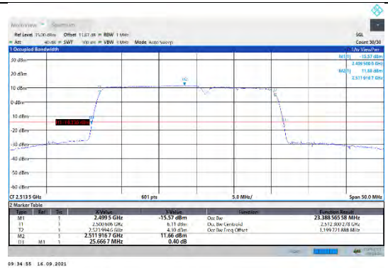
CA_7C-15MHz-10MHz-QPSK-QPSK-20825-20945-75RB#0-50RB#0
