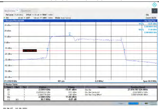
CA_7C-10MHz-20MHz-16QAM-16QAM-21206-21350-50RB#0-100RB#0
