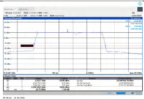
CA_7C-15MHz-10MHz-QPSK-QPSK-21051-21171-75RB#0-50RB#0
