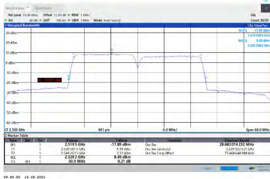
CA_7C-15MHz-15MHz-16QAM-16QAM-21025-21175-75RB#0-75RB#0
