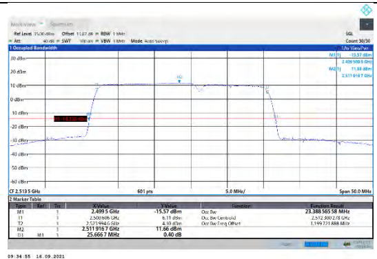
CA_7C-15MHz-10MHz-QPSK-QPSK-20825-20945-75RB#0-50RB#0
