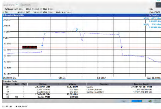
CA_7C-20MHz-20MHz-QPSK-QPSK-21152-21350-100RB#0-100RB#0
