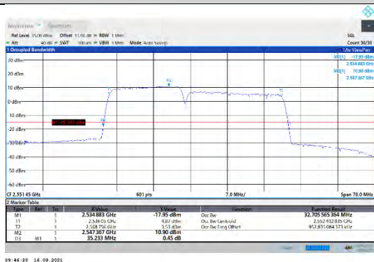
CA_7C-15MHz-20MHz-16QAM-16QAM-21179-21350-75RB#0-100RB#0
