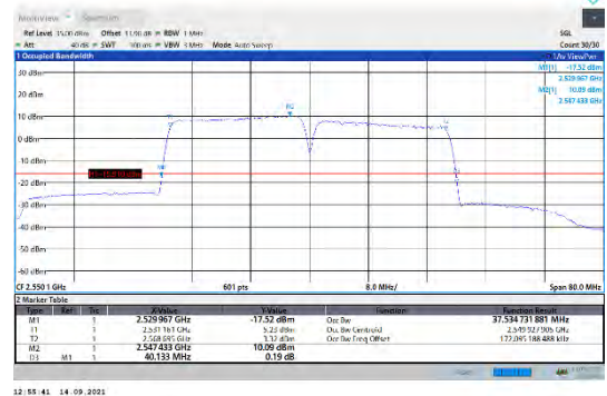
CA_7C-20MHz-20MHz-QPSK-QPSK-21152-21350-100RB#0-100RB#0
