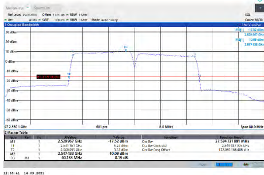
CA_7C-20MHz-20MHz-QPSK-QPSK-21152-21350-100RB#0-100RB#0
