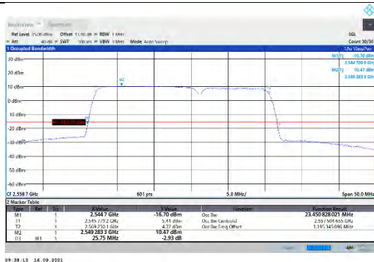
CA_7C-15MHz-10MHz-16QAM-16QAM-21277-2139CA_7C5RB#0-50RB#0
