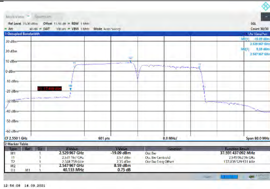
CA_7C-20MHz-20MHz-16QAM-16QAM-21152-21350-100RB#0-100RB#0
