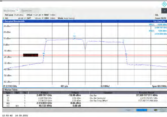
CA_7C-20MHz-20MHz-16QAM-16QAM-20850-21048-100RB#0-100RB#0
