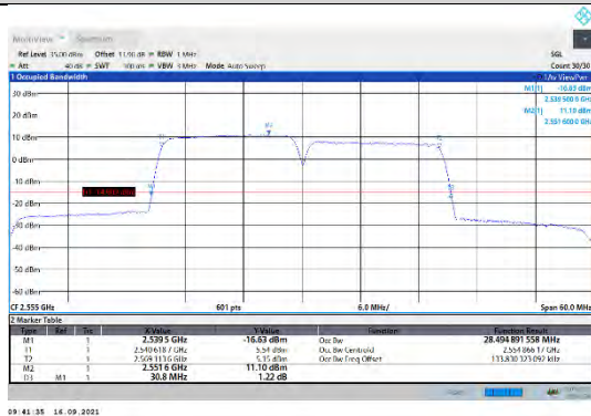
CA_7C-15MHz-15MHz-QPSK-QPSK-21225-21375-75RB#0-75RB#0
