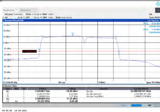
CA_7C-20MHz-15MHz-16QAM-16QAM-21201-21372-100RB#0-75RB#0
