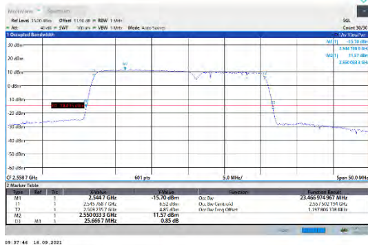
CA_7C-15MHz-10MHz-QPSK-QPSK-21277-2139CA_7C5RB#0-50RB#0
