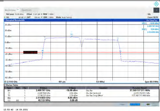
CA_7C-20MHz-20MHz-16QAM-16QAM-20850-21048-100RB#0-100RB#0
