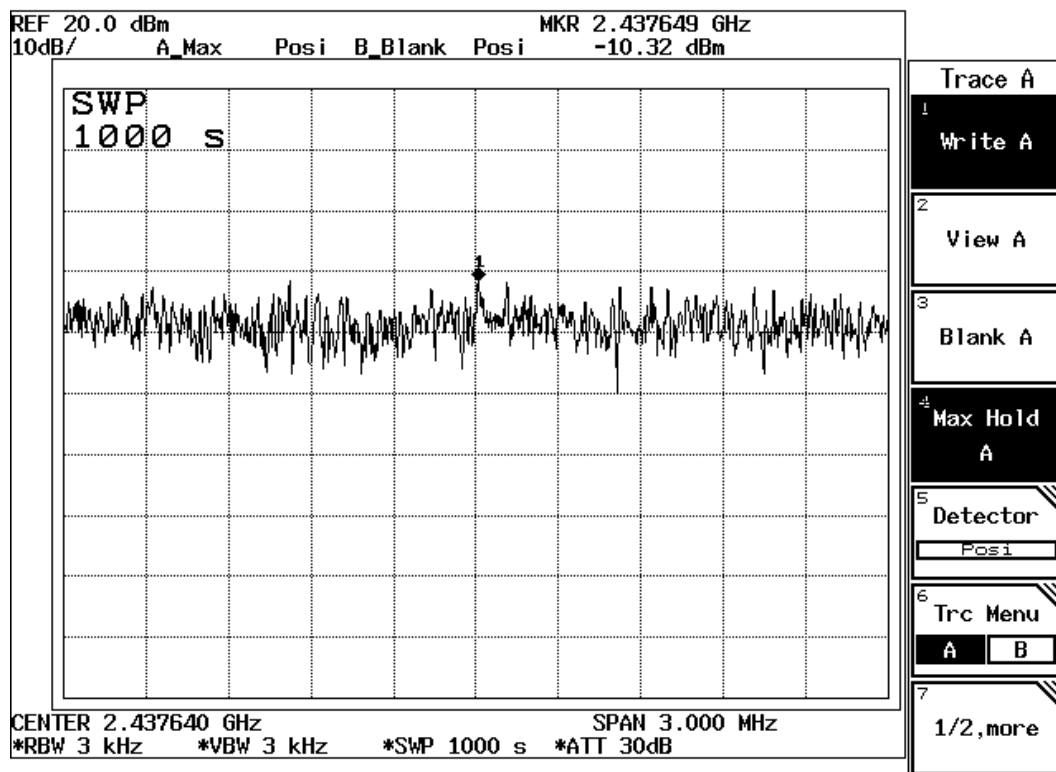
Figure Channel 6: 11Mbps
