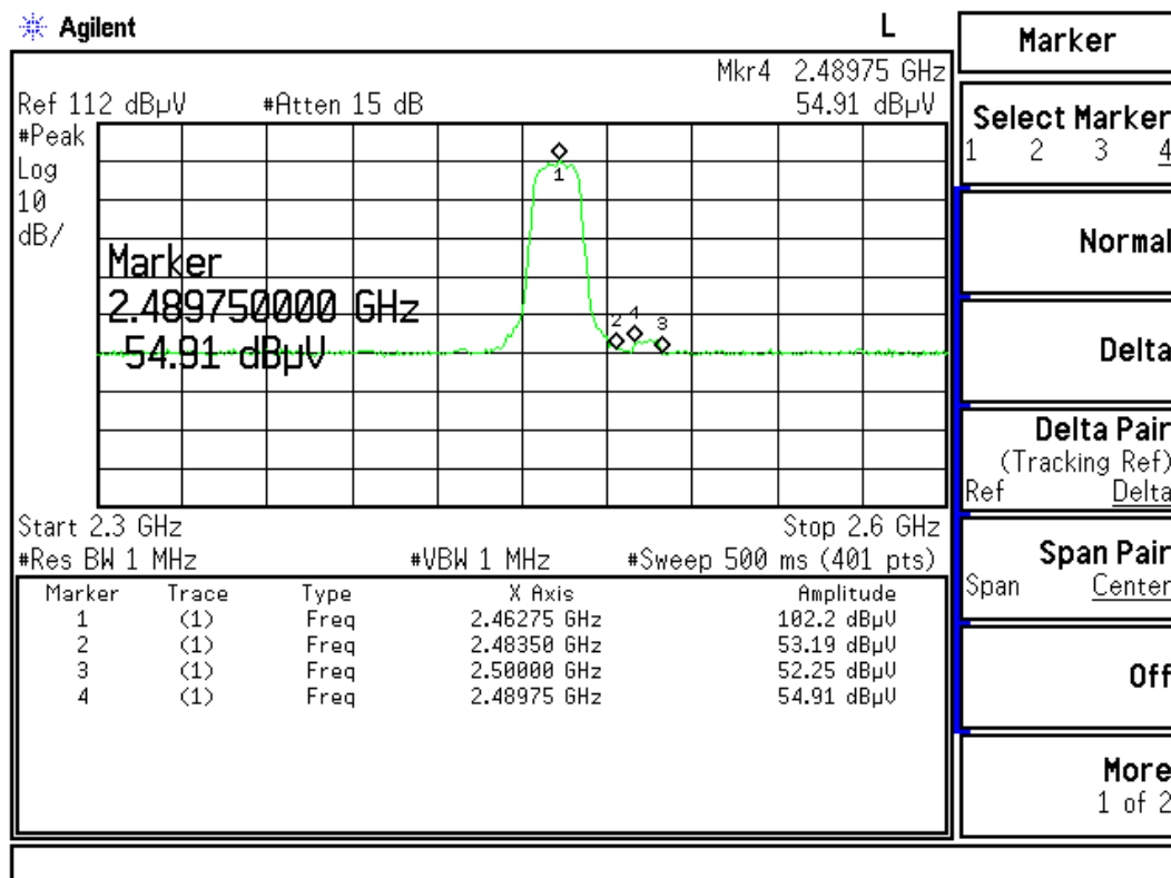
Figure Channel 11: (Vertical)
