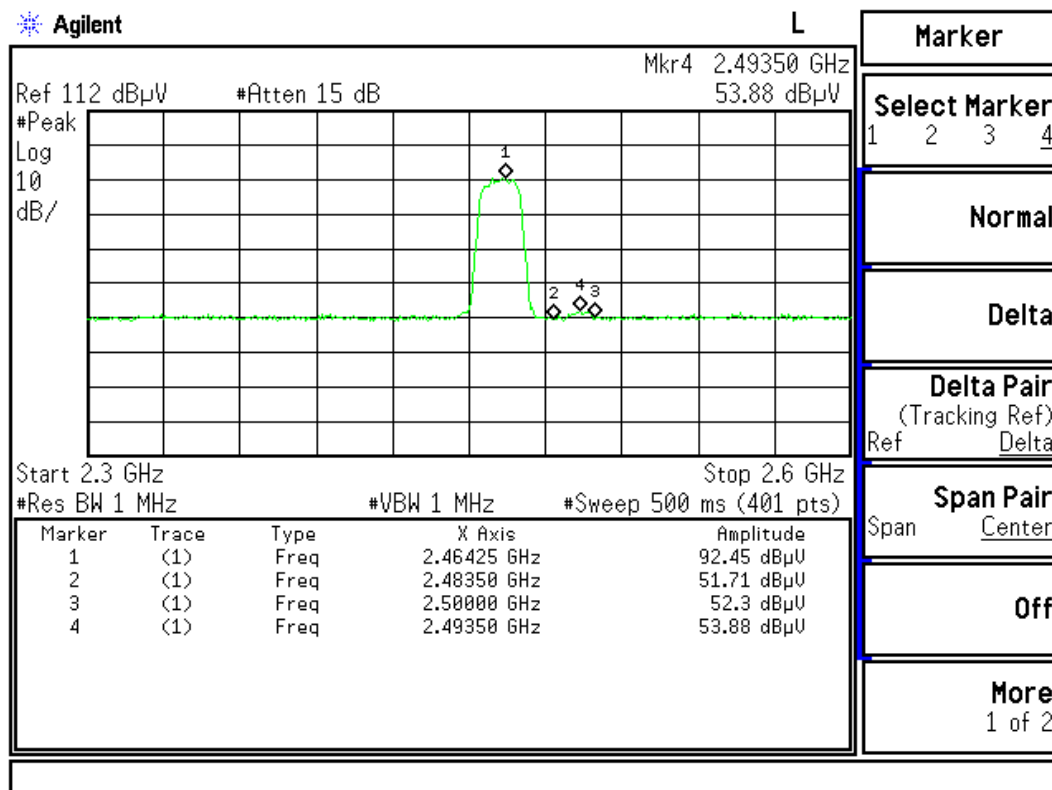
Figure Channel 11: (Horizontal)
