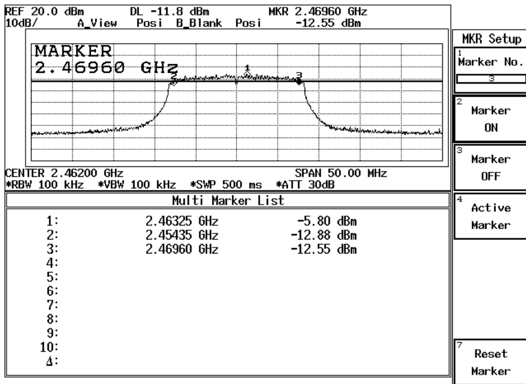
Figure Channel 11: 54Mbps
