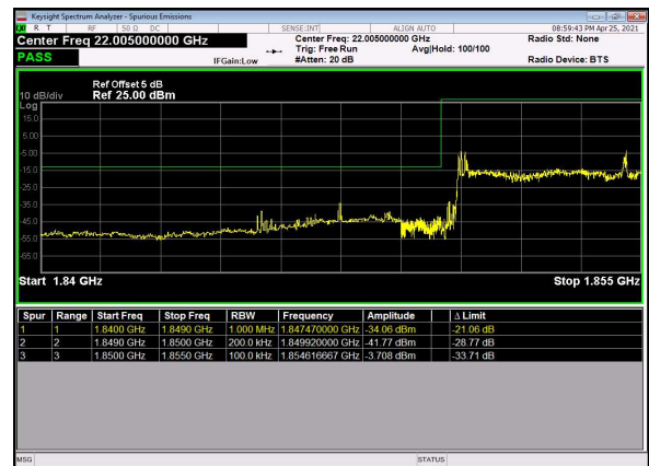
N2(20M)_DFT-s-OFDM_QPSK_Outer_Full_Lo w_CH
