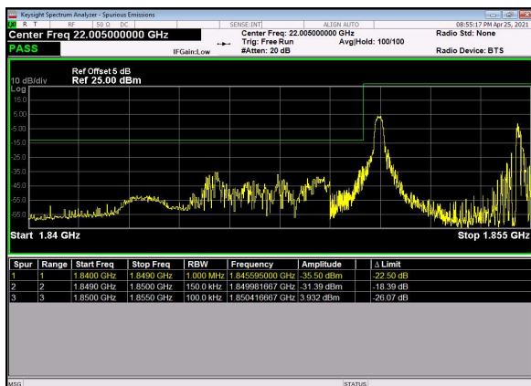
N2(15M)_DFT-s-OFDM_BPSK_Edge_1RB_Lef t_Low_CH
