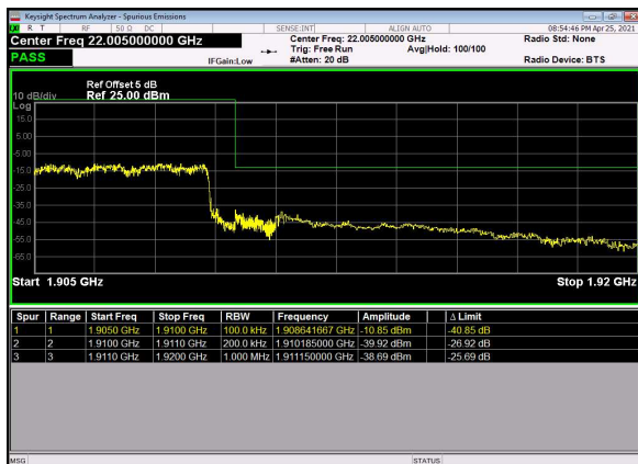
N2(10M)_DFT-s-OFDM_BPSK_Outer_Full_Hig h_CH
