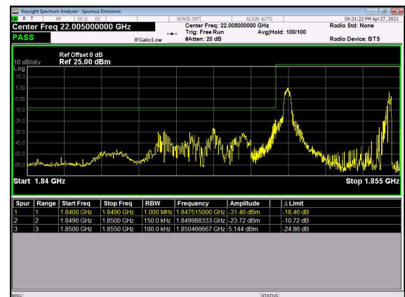
N2(15M)_DFT-s-OFDM_QPSK_Edge_1RB_Lef t_Low_CH
