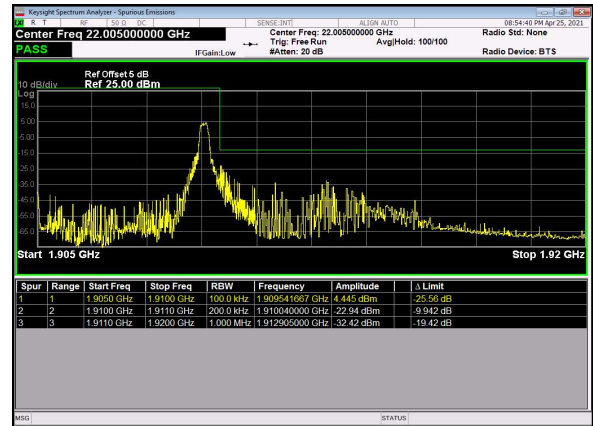
N2(10M)_DFT-s-OFDM_QPSK_Edge_1RB_Ri ght_High_CH
