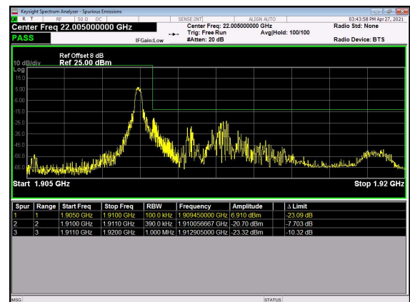
N2(20M)_DFT-s-OFDM_QPSK_Edge_1RB_Ri ght_High_CH
