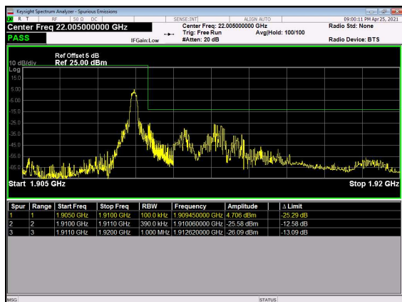
N2(20M)_DFT-s-OFDM_BPSK_Edge_1RB_Rig ht_High_CH
