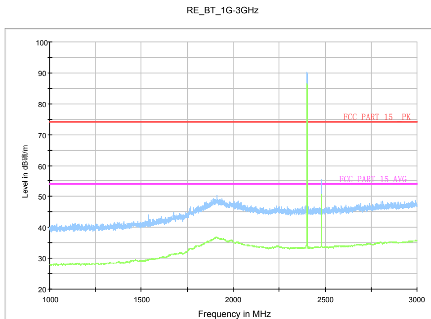
Fig.78. Radiated emission: 8DPSK, Channel 0, 1 GHz - 3 GHz
