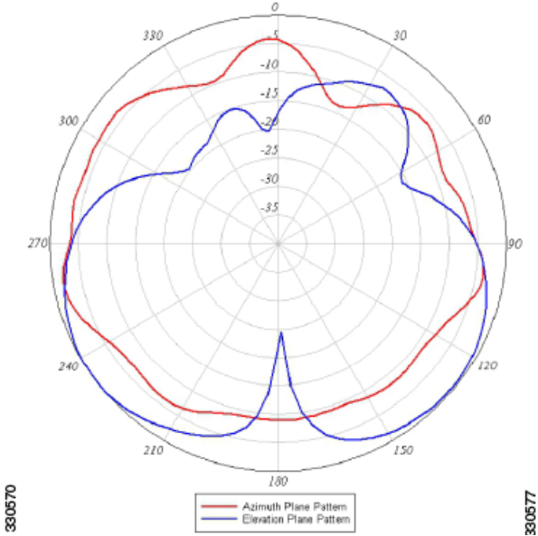
5 GHz Element 4 Azimuth and Elevation Plane Patterns
