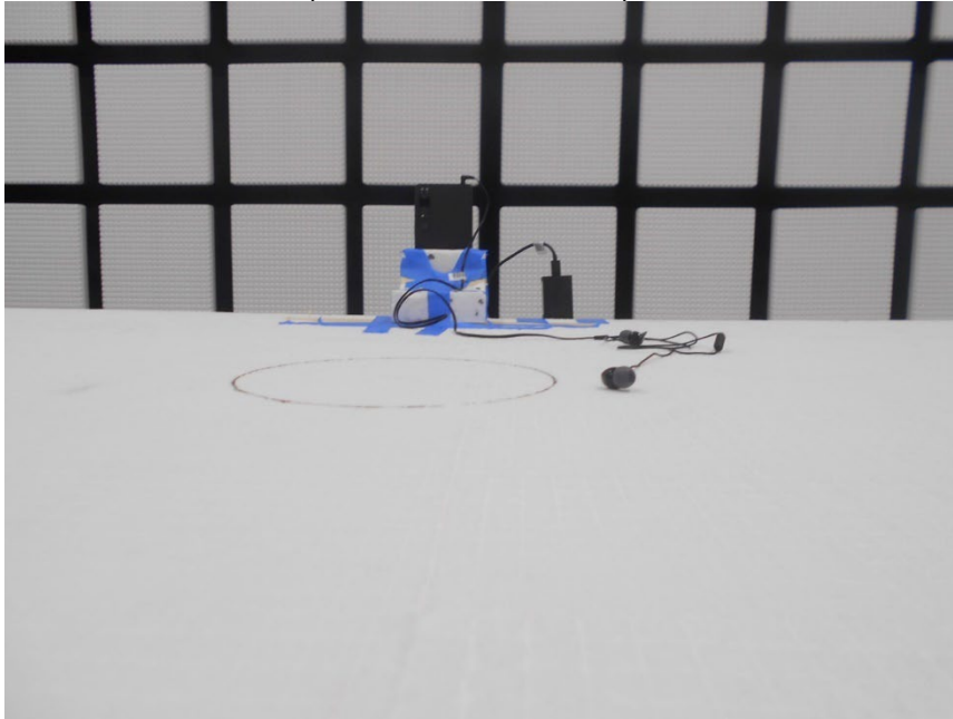
RADIATED PHOTO (>1GHz WLAN MIMO)
