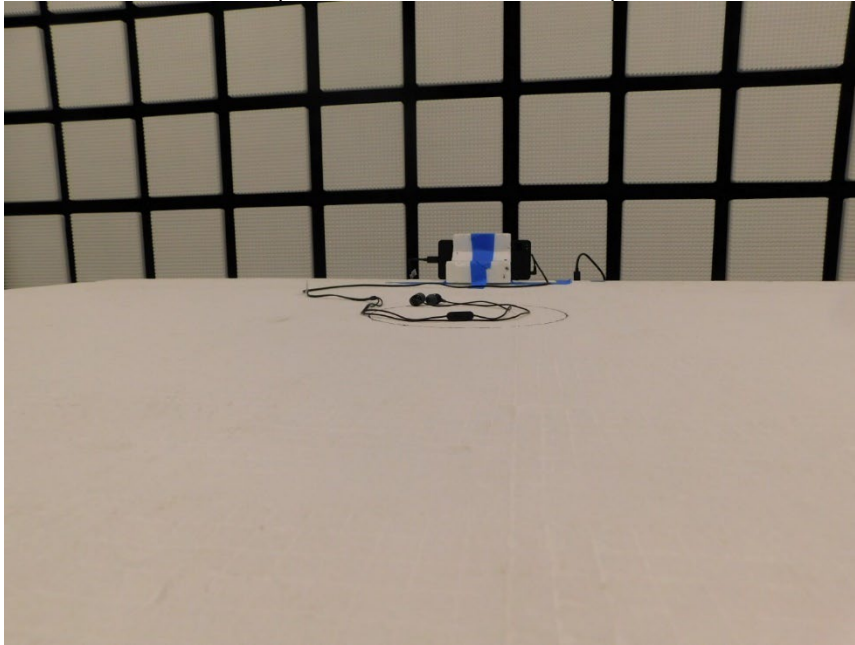
RADIATED PHOTO (>1GHz BT/BLE CHAIN 1)
