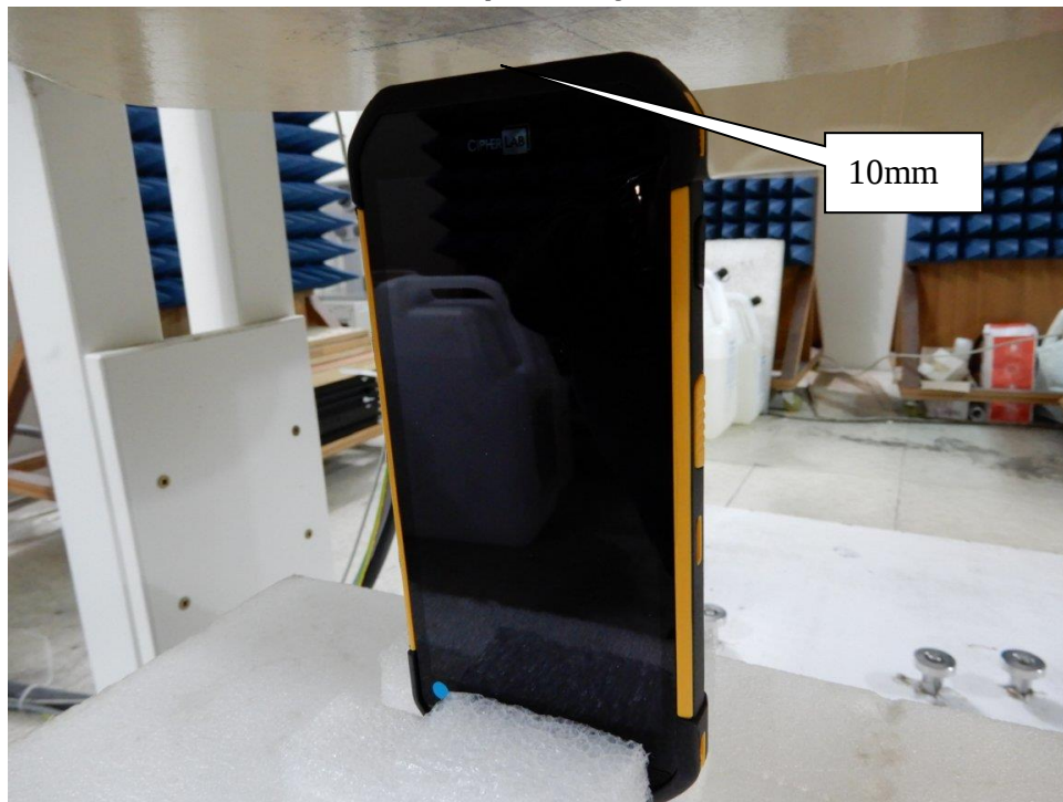
EUT Top – Body SAR
