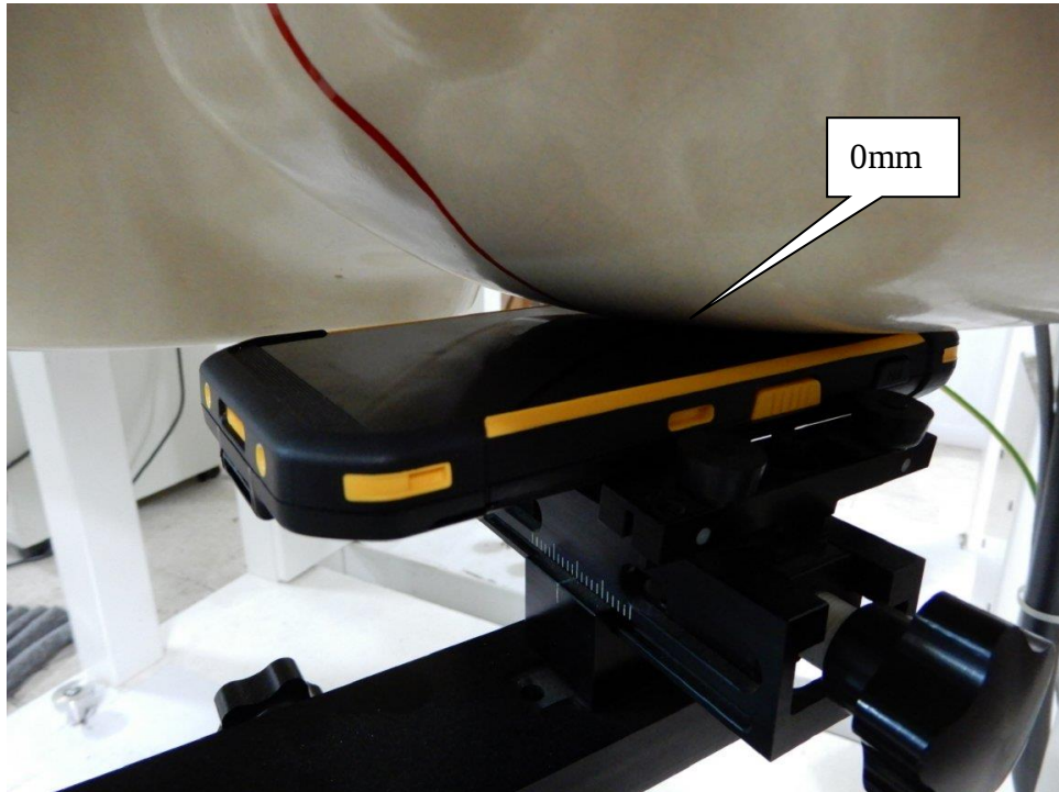
EUT Left-Cheek – Head SAR
