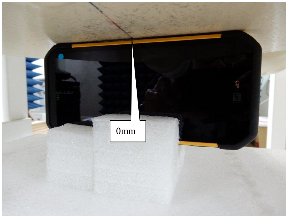
EUT Left-Side – Limb SAR
