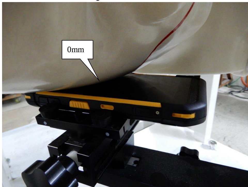
EUT Right-Cheek – Head SAR
