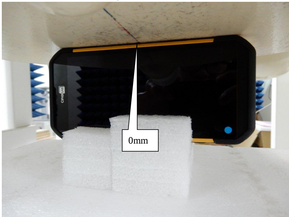
EUT Right-Side – Limb SAR
