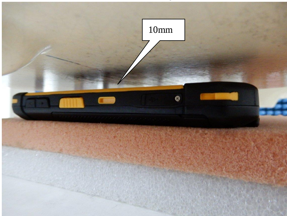
EUT Front – Body SAR
