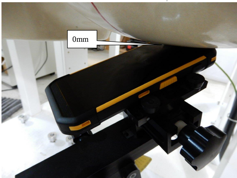
EUT Left-Tilt – Head SAR
