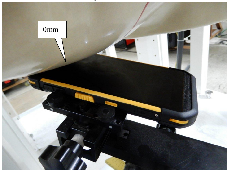
EUT Right-Tilt – Head SAR
