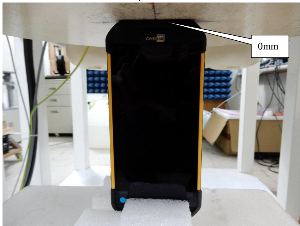
EUT Top – Limb SAR
