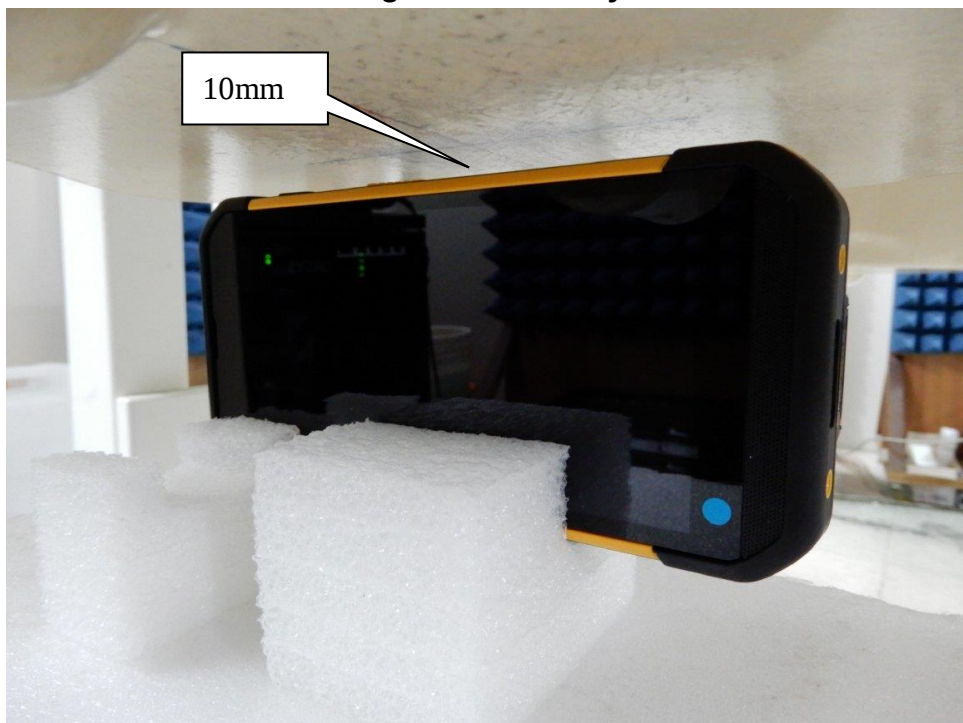
EUT Right-Side – Body SAR
