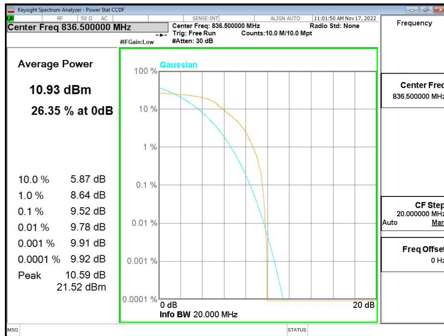
Band26-CH26915-836.5MHz-10MHz Bandwidth-QPSK
