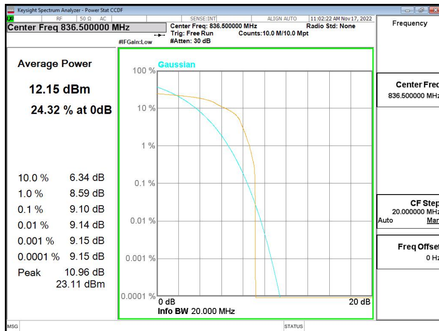
Band26-CH26915-836.5MHz-10MHz Bandwidth-16QAM
