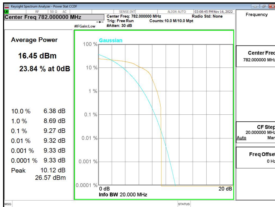
Band13-CH23230-782MHz-5MHz Bandwidth-16QAM
