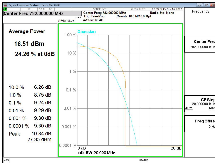
Band13-CH23230-782MHz-10MHz Bandwidth-16QAM
