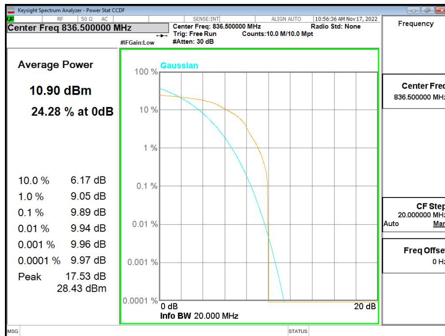
Band26-CH26915-836.5MHz-3MHz Bandwidth-16QAM
