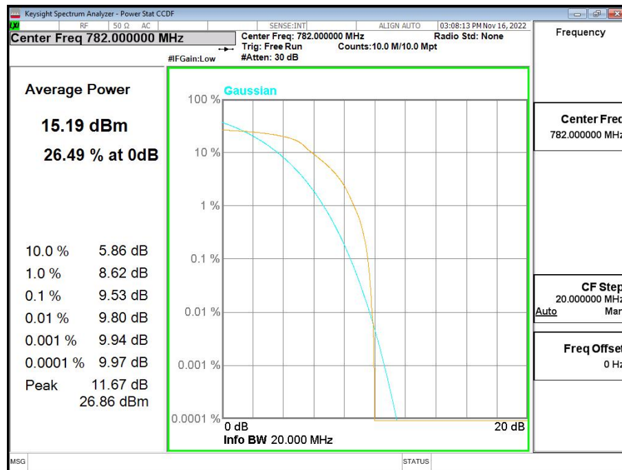
Band13-CH23230-782MHz-5MHz Bandwidth-QPSK
