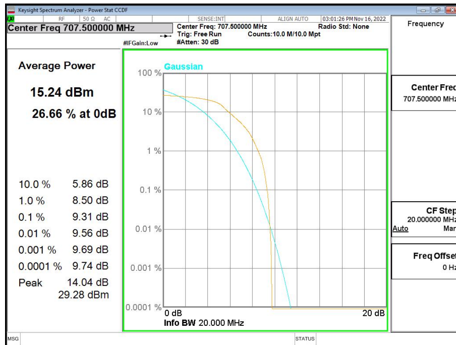
Band12-CH23095-707.5MHz-10MHz Bandwidth-QPSK
