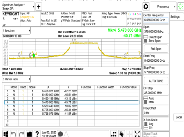
802.11ac_80M_5610 MHz_Peak_chain1
