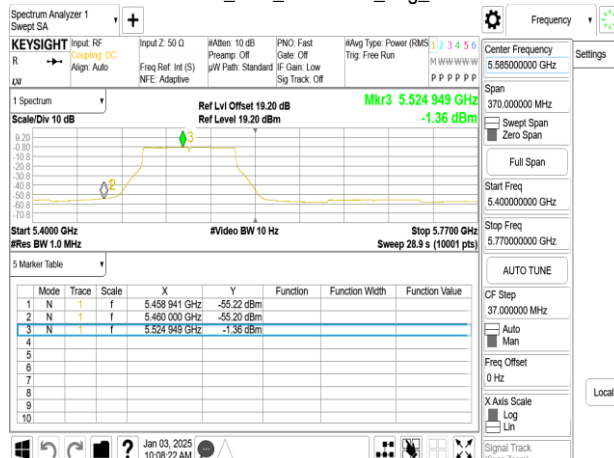
802.11ac_80M_5530 MHz_Avg_chain1
