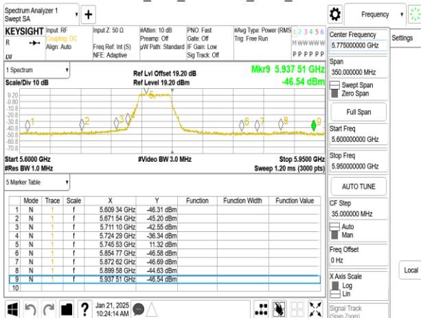
802.11n_40M_5755 MHz_Peak_chain0
