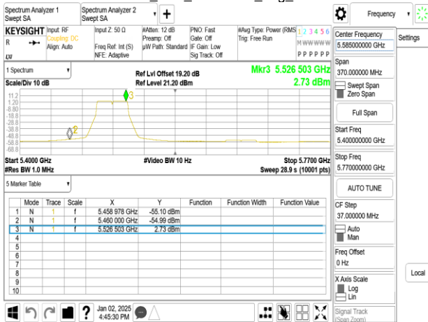
802.11n_40M_5510 MHz_Avg_chain1
