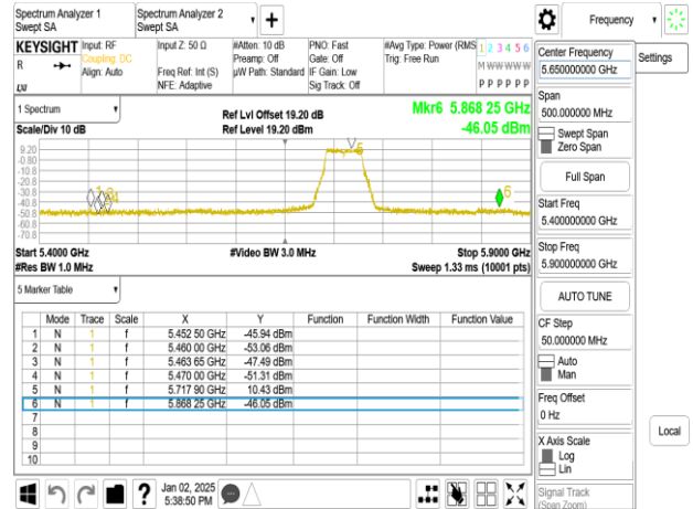
802.11n_40M_5710 MHz_Peak_chain1
