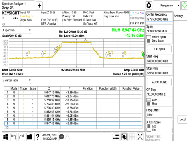
802.11ac_80M_5775 MHz_Peak_chain1
