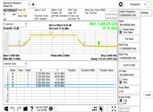
802.11ac_160M_5250 MHz_Avg_chain0
