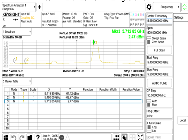
802.11n_20M_5720 MHz_Avg_chain0
