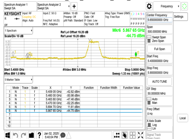
802.11n_40M_5710 MHz_Peak_chain1
