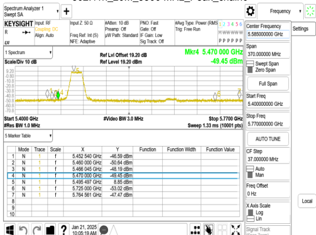
802.11n_20M_5500 MHz_Peak_chain1
