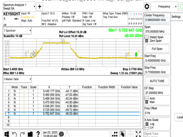
802.11ac_80M_5530 MHz_Avg_chain0
