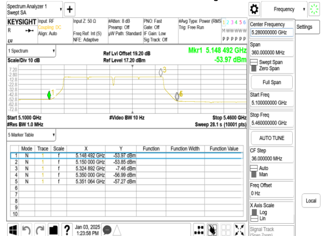
802.11ac_160M_5250 MHz_Avg_chain1
