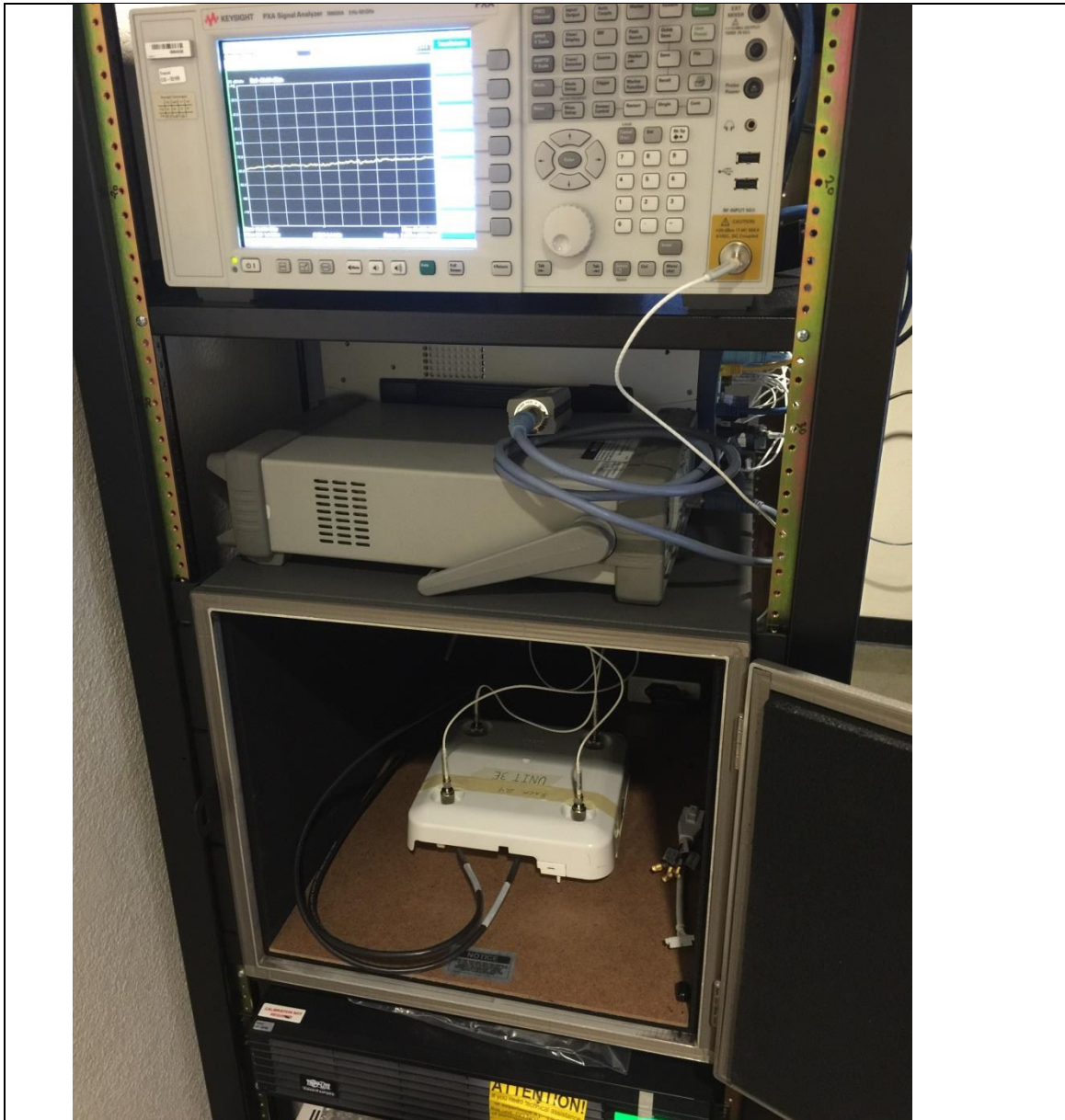
Title: Conducted Test Setup
